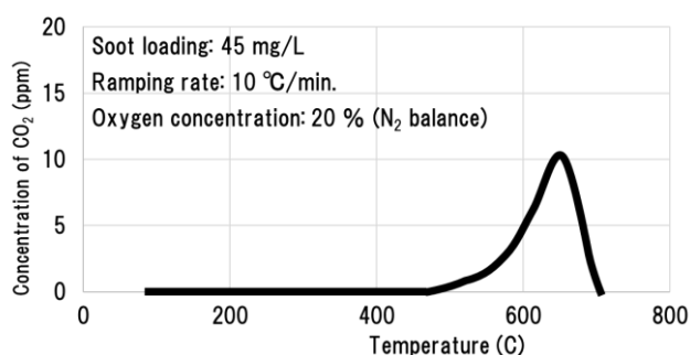
Fig.10 Temperature program oxidation of soot trapped on the TWC particles membrane filter
