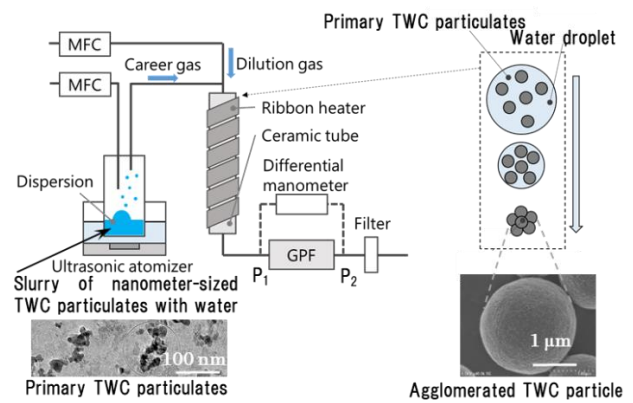
Fig.3 Schematic diagram for fabricating agglomerated TWC particle
