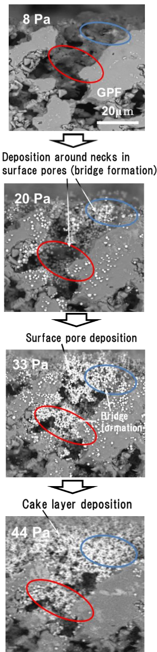
Fig.6 Time-lapse SEM images of cross-sectional views during deposition of TWC particles around surface pores of cordierite GPF substrate
