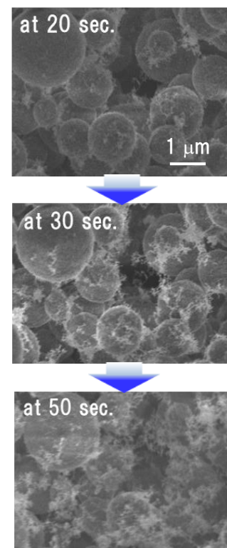
Fig.9 Time-lapse SEM images of surface views during soot deposition on the surface of TWC particles membrane filter
