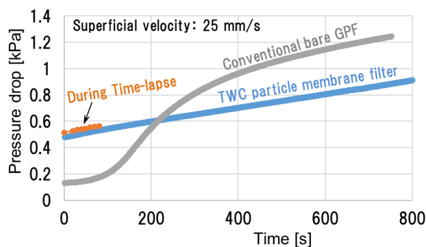
Fig.8 Pressure drop increase during soot deposition on TWC particles membrane filter on the cordierite GPF substrate and the conventional bare cordierite GPF
