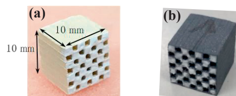
Fig.1 Miniature sized filters made of cordierite (a) and SiC (b)
