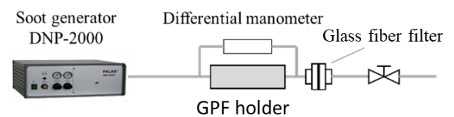
Fig.4 Schematic diagram of setup for soot trapping
