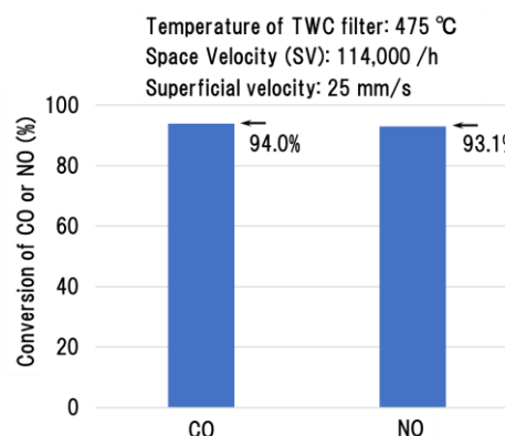
Fig.11 Conversion of CO and NO by TWC particles membrane filter
