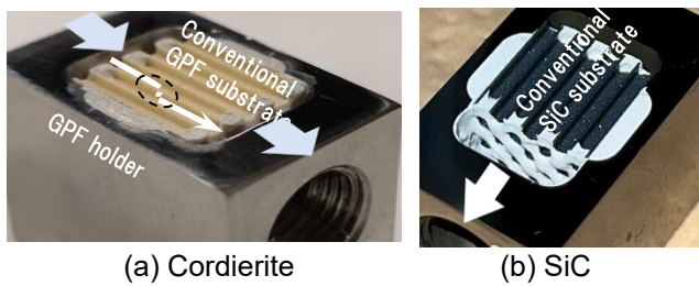
Fig.2 Filter holders with an open channel for time-lapse SEM visualization
