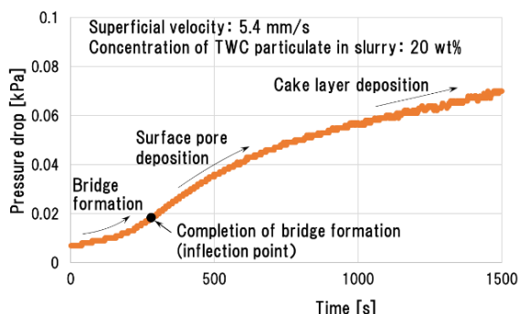
Fig.5 Pressure drop increase during deposition of TWC particulates on the conventional cordierite GPF substrate
