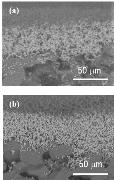
Fig.7 SEM images of cross-sectional view of TWC particles membrane on cordierite (a) and SiC (b) GPF substrates
