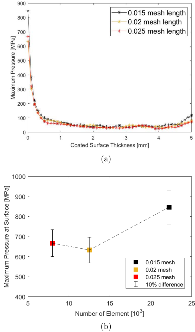
Figure 2.5: Maximum pressure (a) along coated surface thickness and (b) at coated material's surface.
