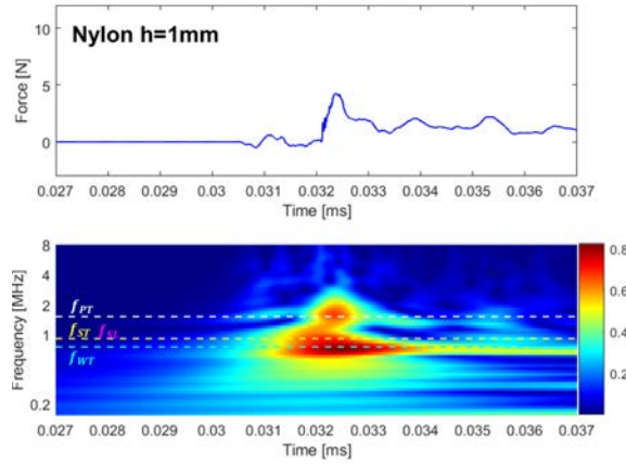
(c) Nylon h = 1\text{mm} .
