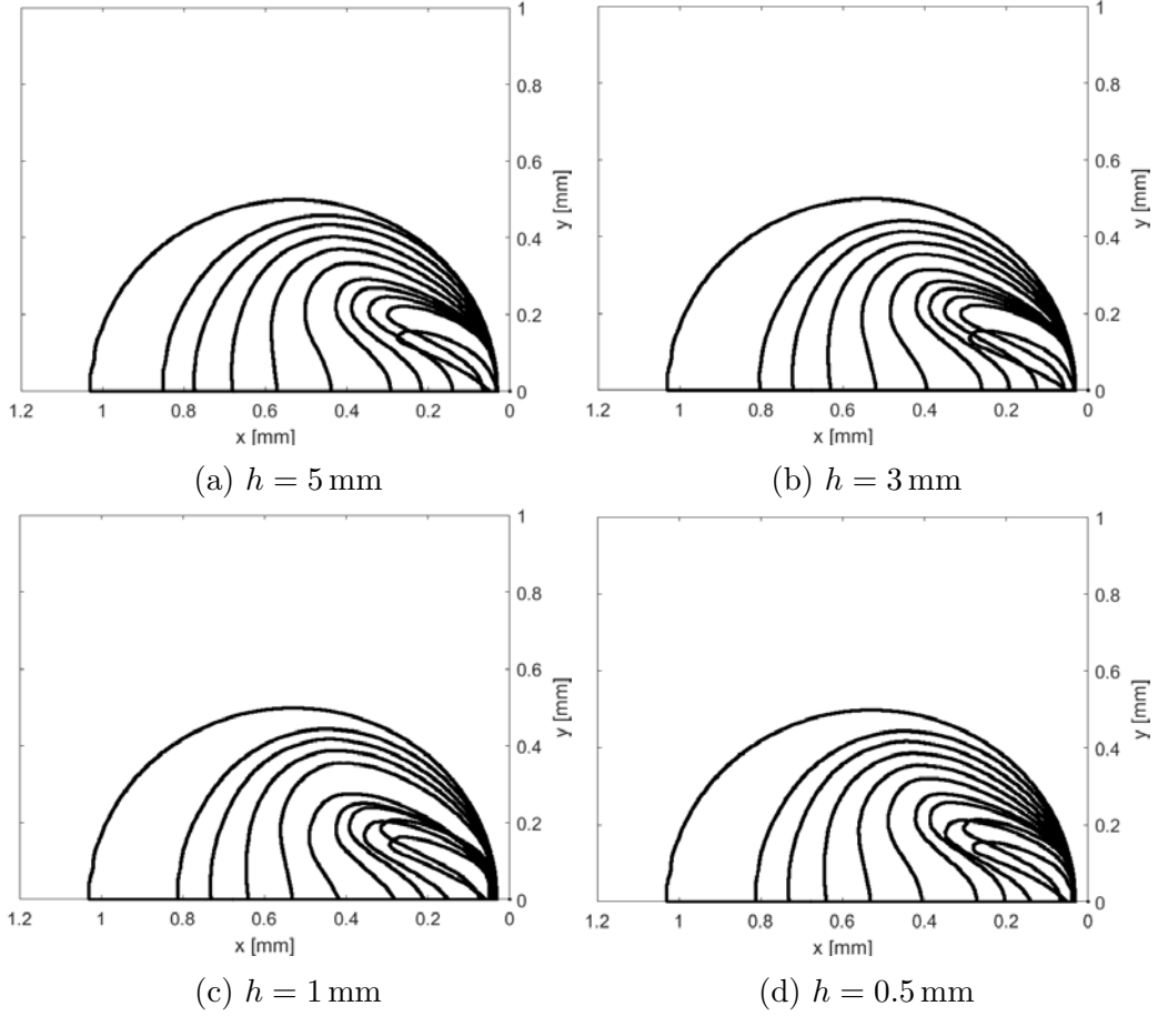
Figure 4.3: The evolution of nonpherical bubble deformation extracted at the same time for Titanium case.
