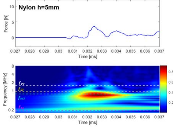
(a) Nylon h = 5\text{mm} .
