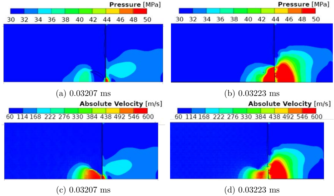
Figure 3.9: The profile contour (a) and (b), and absolute velocity (c) and (d) at toroidal bubble formation timing. Profile contour on Al2024 is von Mises stress with a similar scale as that in 3.3.
