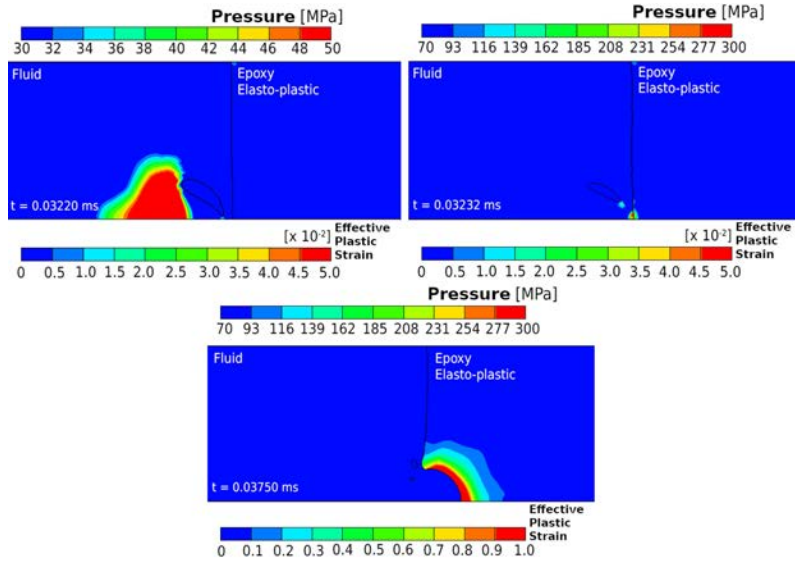
(b) Epoxy elasto-perfectly plastic.
