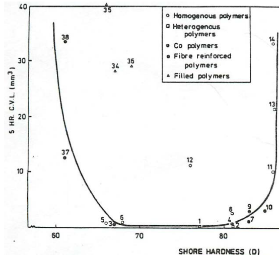
Figure 1.1: 5-hour Cavitation Volume Loss and Shore Hardness from [1.6].
