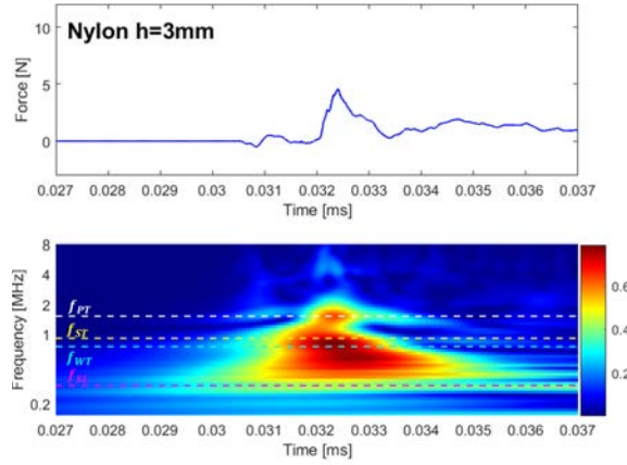
(b) Nylon h = 3\text{mm} .
