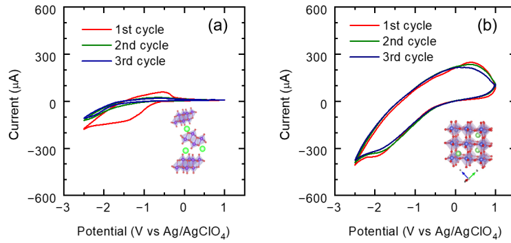
Fig. 1 Cyclic voltammogram for \alpha - and \beta - \text{MoO}_3 | \text{LiClO}_4 :PC| \text{LiCoO}_2 /Al electrochemical cells taken during repeated Li-ion electrochemical reactions.
