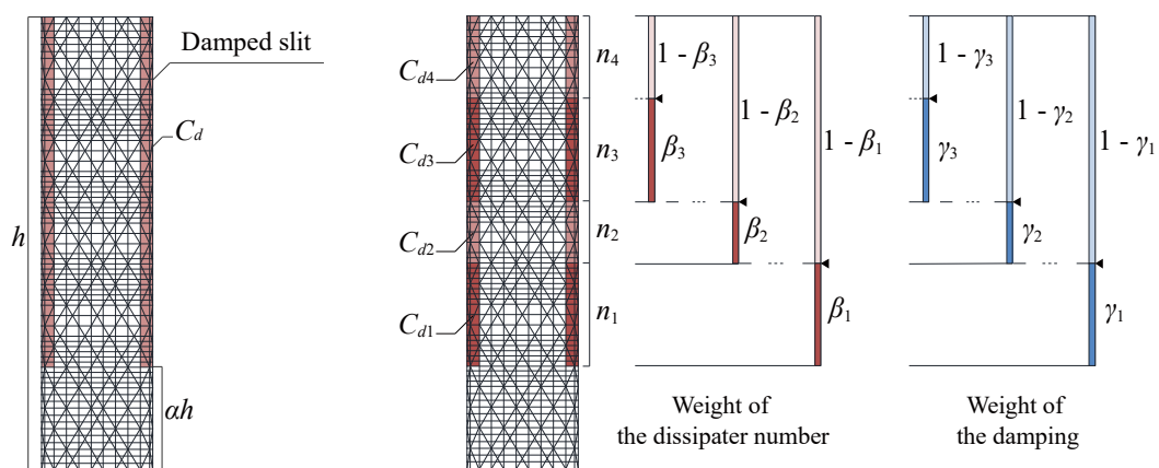
(a) Uniform dissipater distribution
