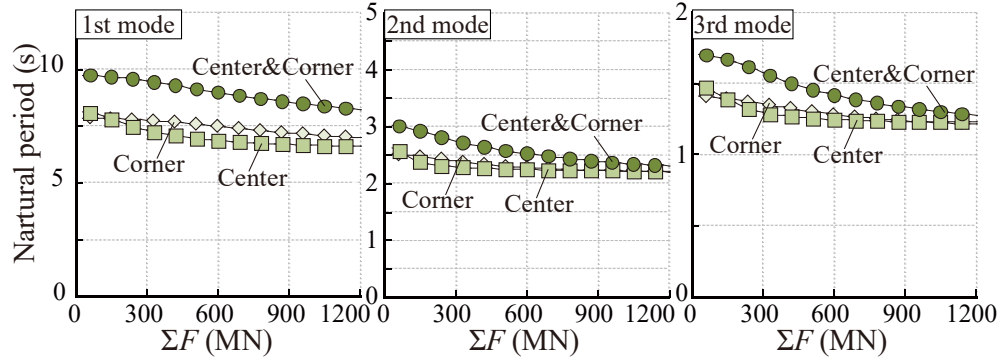
(b) 1st to 3rd mode natural period ( \alpha=0.22 )
