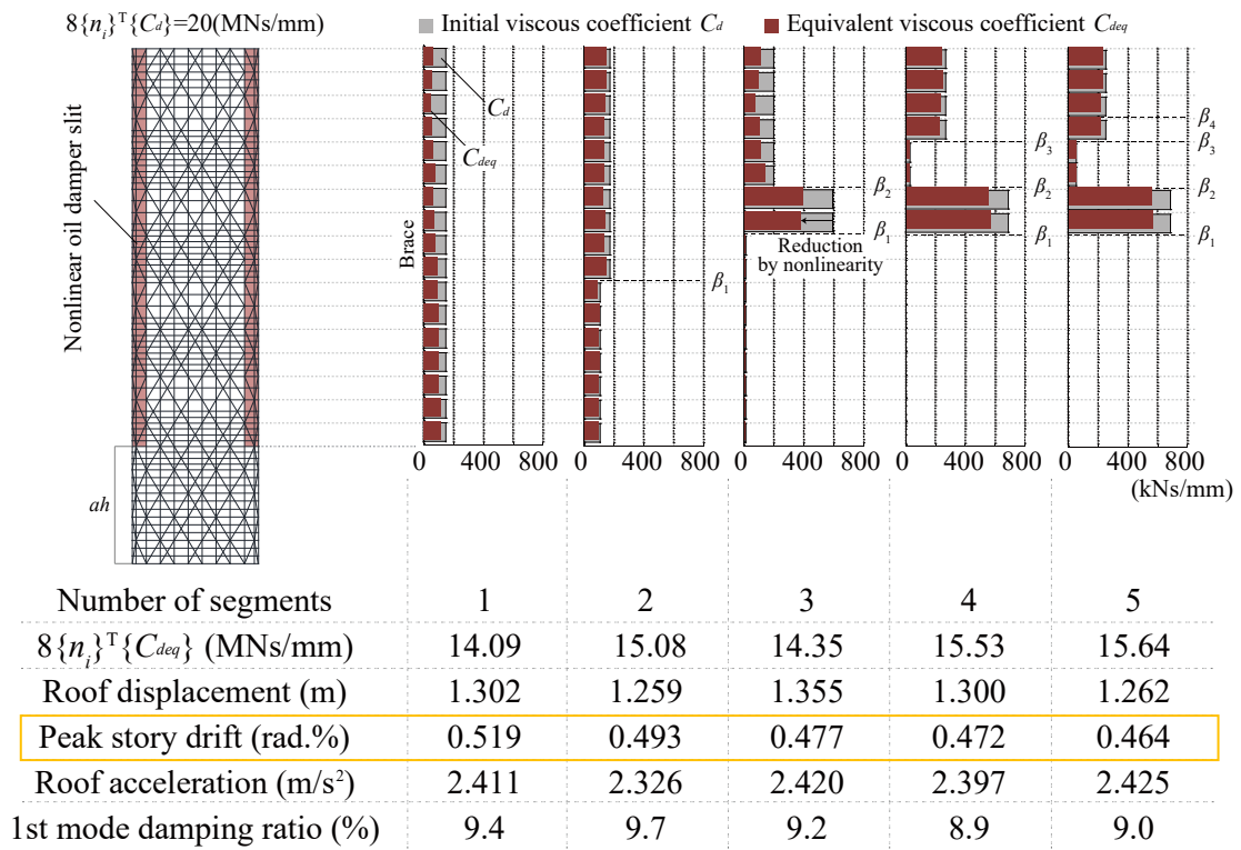
(b1) Minimization of peak story drift by spectrally matched waves
