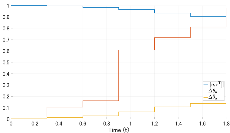
Fig. 3.10: The trajectory of l_2 -norm of the Euler parameter states of simulation and rotation angles of difference of rotation matrices: \Delta\theta_a and \Delta\bar{\theta}_a
