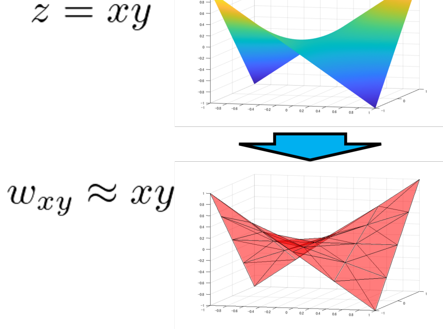
Fig. 3.2: An approximation of the quadratic term xy by MICP
