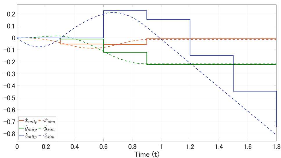
Fig. 3.9: Comparison of velocity states of the solution and simulator. Solid: the solution. Dashed: simulator.
