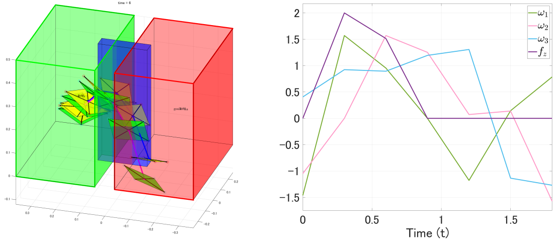
Fig. 3.6: Left: Comparison of the behavior of a solution and simulator. The green rectangle represents the simulation of the drone to which inputs obtained by the Mixed-Integer Linear Problem planning are applied. Right: Input sequences used in the simulator. We applied the First-order hold to the input obtained by the Mixed-Integer Linear Problem planning.
