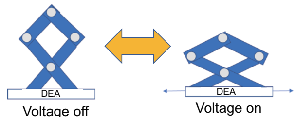
Fig.2 The Schematic of the mechanism consisting of DEA and a simple pantograph structure.
