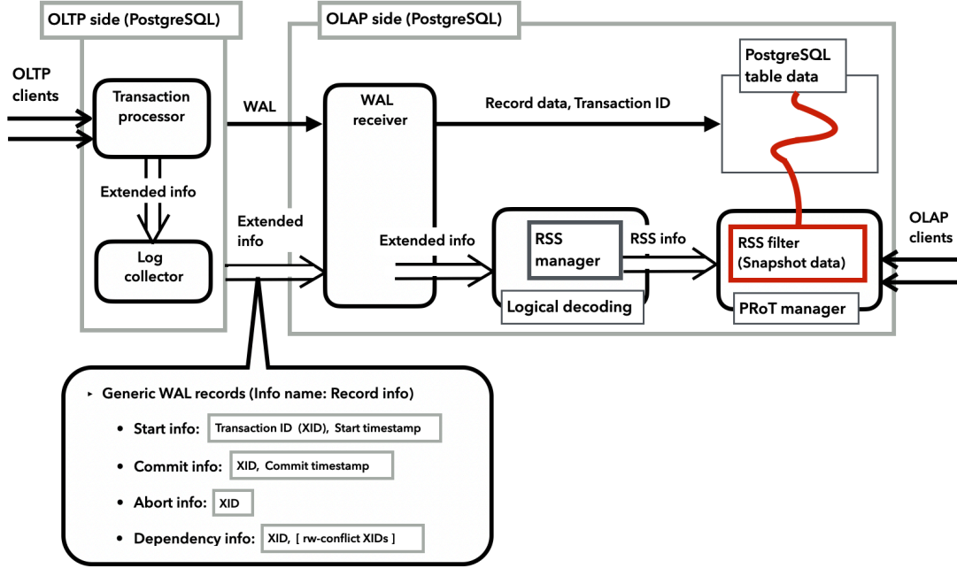
Figure 4.3: Decoupled storage (multinode) architecture overview. Twin arrows \Rightarrow represent clients. A single arrow \rightarrow represents existing processing flows of PostgreSQL. An open arrow \Rightarrow represents newly implemented processing flows.
