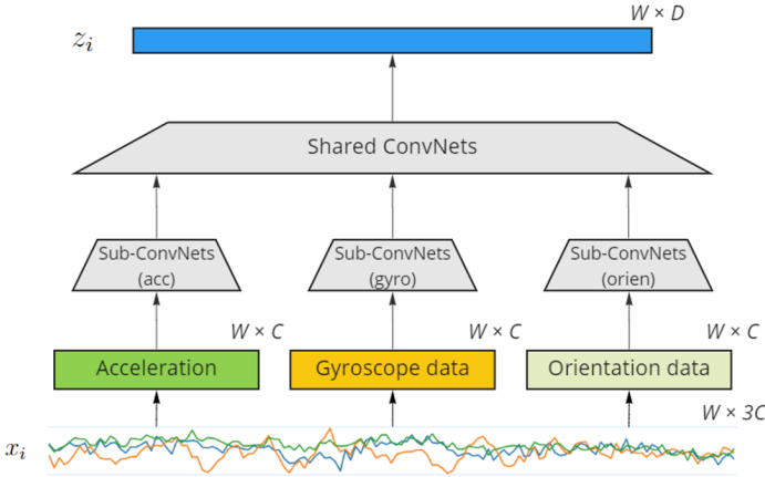
Fig. 3: Front-Processing Module: W refers to window size, i.e., the number of frames in each clip, D refers to the feature dimension, which is a predefined hyperparameter, C = 3 is the dimension of each data type
