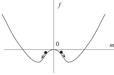
FIG. 7.4. Free energy of the Hopfield model when a single pattern is retrieved.
