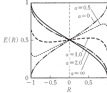
FIG. 8.4. Generalization error of the non-monotonic perceptron
