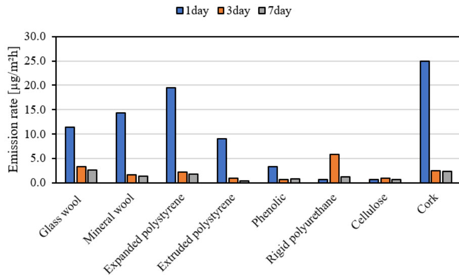
Figure 4-13. Acetaldehyde emission rates from insulation materials
