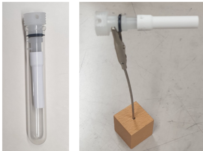
Figure 2-3. Passive Sampler of VOC
