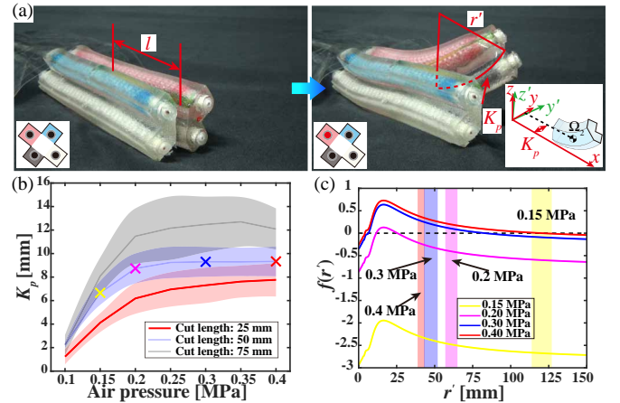
Fig. 14. (a) Bending experiment of the self-repairing soft robot to achieve first rotation. (b) Correction values for different cut lengths under different pressures were applied. (c) Condition for a robot with a cut length of 50 mm to achieve the first rotation. The shaded regions show the experimental values of the radius of curvature ( r' ) under different air pressures.
