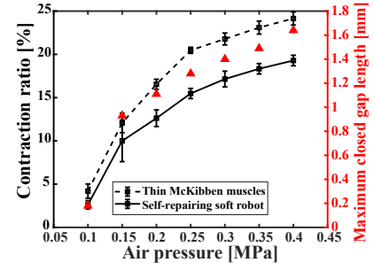
Fig. 11. The relationship between applied air pressure and contraction ratio in thin McKibben muscles (black dashed line) and the self-repairing soft robot (black solid line), and the maximum gap length (red triangles) that can be repaired under different air pressure.
