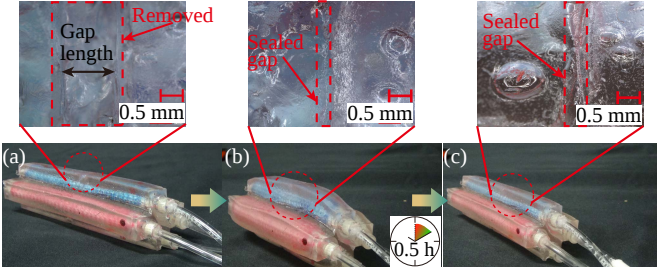
Fig. 10. The process of the self-repairing soft robot recovering from material removal. Here, a digital microscope (VHX-8000 series, KEYENCE) is used to observe the cut surfaces. (a) Damage with a gap length of 1.5 mm. (b) Repairing the damage. (c) Repair accomplished.
