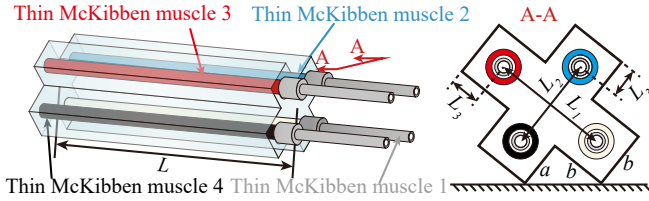
Fig. 3. Prototype of the novel self-repairing soft robot: CAD design and cross-section. Here, b + 2a = L_2 + 2 \times L_3 and 3b = L_1 + 2 \times L_3 .
