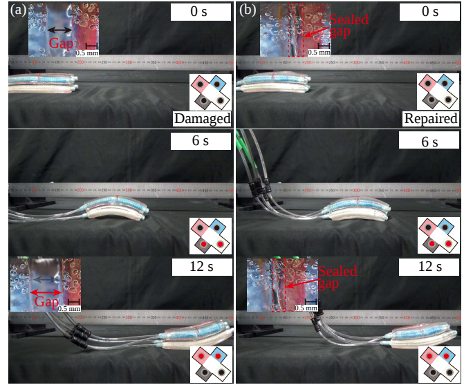
Fig. 12. Photograph sequence of the self-repairing soft robot crawling on a textured surface after material removal and repair. (a) Material removal with a gap length of 1.64 mm. (b) Robot after repair.
