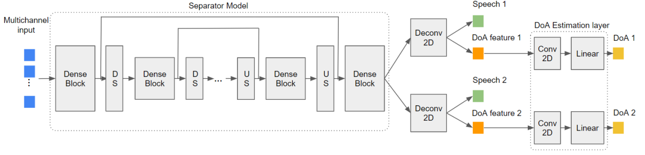
Figure 1: Architecture of the proposed method based on Dense-UNet. DS and US blocks are downsampling and upsampling layers, respectively.
