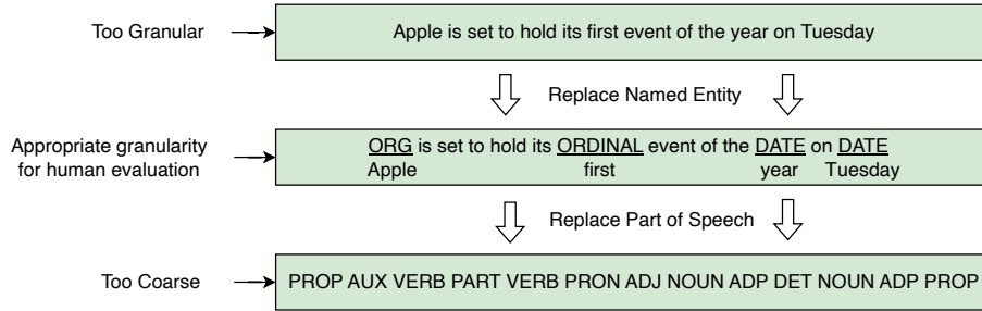
Figure 3.3: Different levels of granularity for sentence representation
