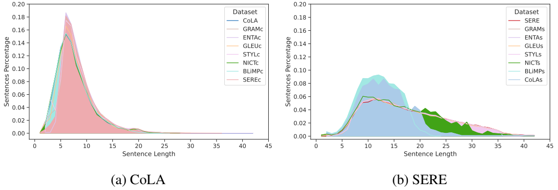
Figure 4.7: Sentence length distribution of datasets when transformed to emulate (a) CoLA and (b) SERE
