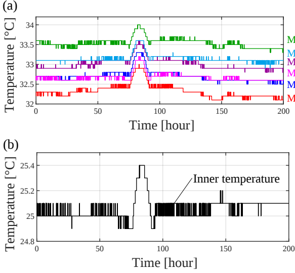
Fig. 3: The temperature measurement result of the drift calibration experiments (a) Head surface temperature of each laser displacement meter (b) Inner temperature
