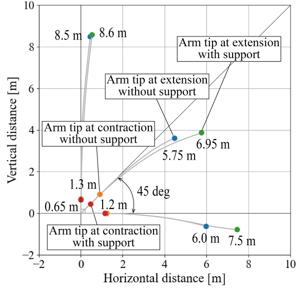
Fig. 8. Results of extension/contraction experiments.
