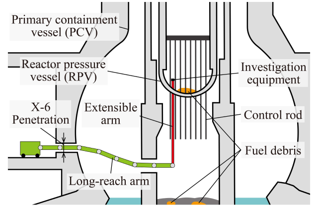
Fig. 1. Planned robotic RPV investigation in Fukushima Daiichi Nuclear Power Plant.
