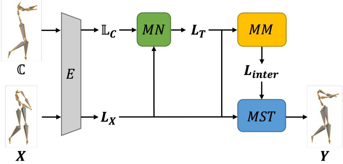
Figure 4.1: System overview: The user’s input motion \mathbf{X} and candidate motions \mathbb{C} are encoded into latent space by encoder \mathbf{E} . The motion navigator \mathbf{MN} selects an optimal learning target. The motion manipulator \mathbf{MM} combines the user’s latent vector with the target to create an intermediate representation, which the motion style transformer \mathbf{MST} decodes into the output motion \mathbf{Y} .
