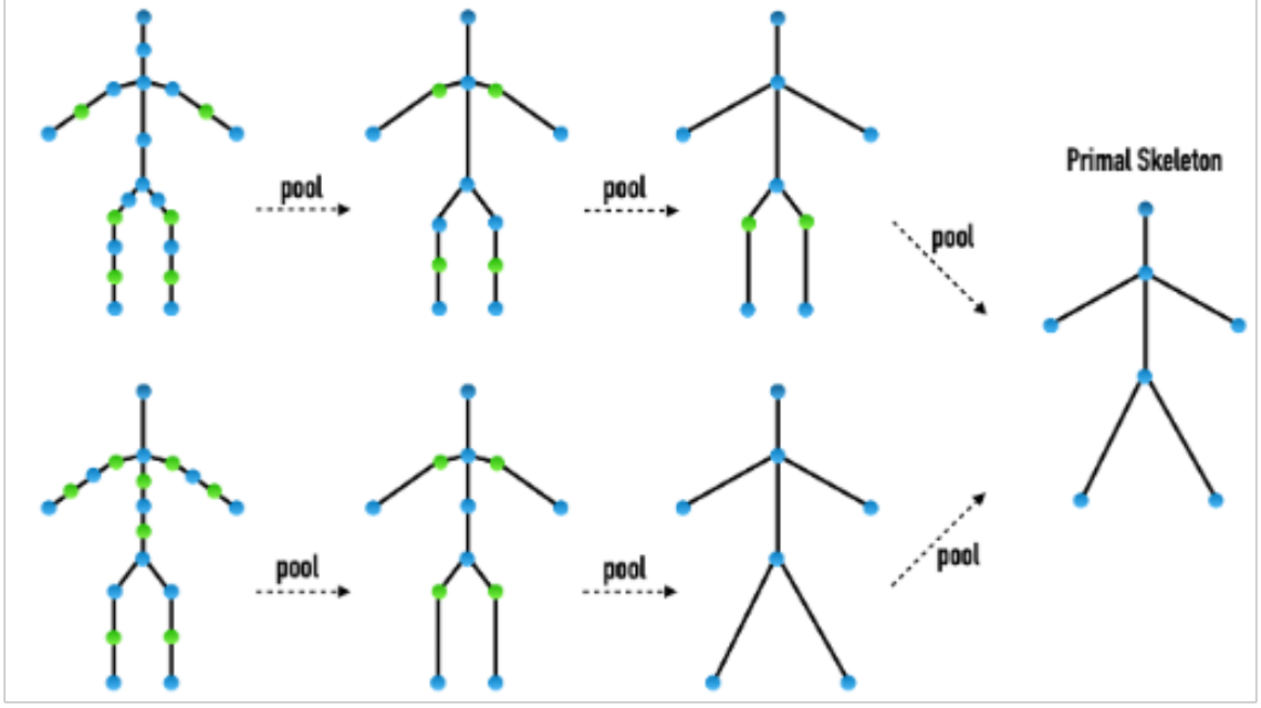
Figure 4.5: Skeletal pooling operation, which reduces the dimensionality while preserving structural information. [9]
