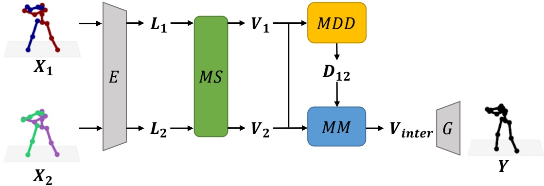
Figure 5.2: System overview. \mathbf{X} is the input motion sequence and \mathbf{Y} is the output human poses restored from the latent space.
