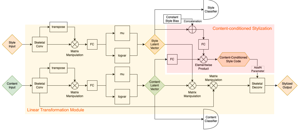
Figure 4.6: Content-preserving motion stylization network architecture.
