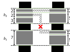
Fig. 3 An enhanced Bin Packing derived from GGCR.
