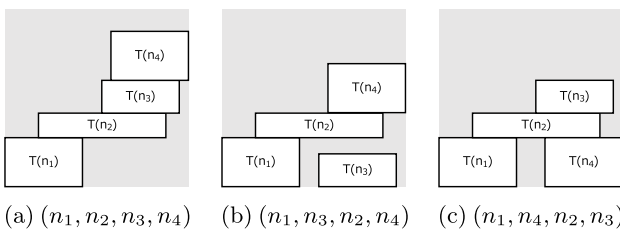
Fig. 4 Allocations by different orders.
