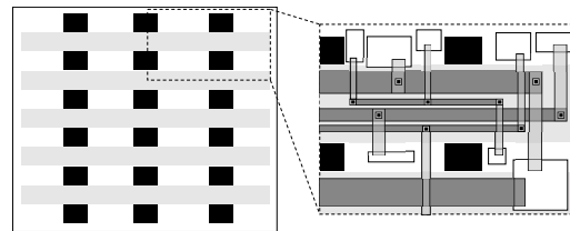
Fig. 1 Gridless gap channel. Gaps (gray) are defined horizontally between obstacles (black) regularly arranged. The pins of nets are defined on modules (white rectangles) inside area. The width of horizontal wires (dark gray) of nets varies.
