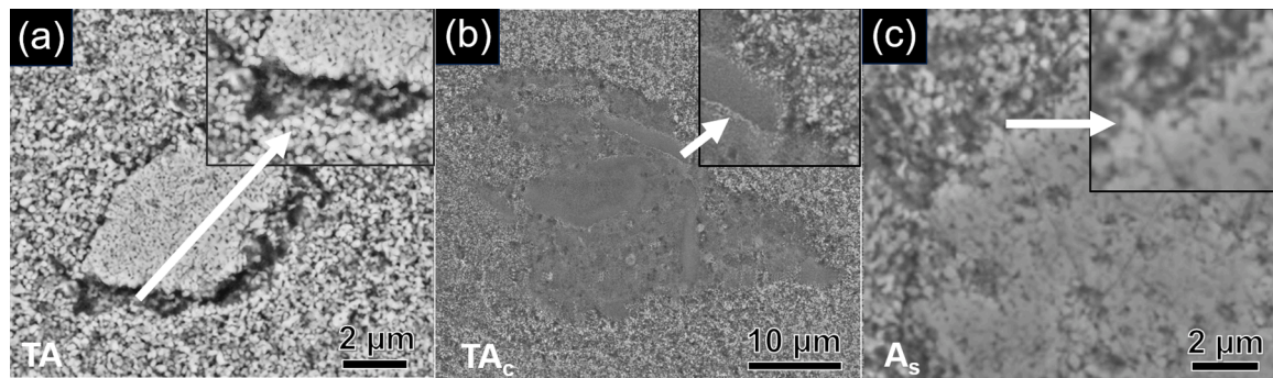
Fig. 5. SEM image of (a) a structure (TA) evolved from transition alumina aggregate, (b) a large composite structure (TA c ) evolved from transition alumina aggregate, (c) small white agglomerates (A s ) in the calcined body ( \rho = 62.8\% ).
