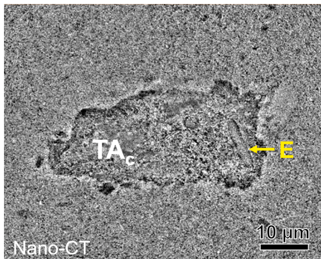
Fig. 4. Enlarged view of a darker, large composite structure evolved from transition alumina aggregate (TA c ), located in the area enclosed by the square in Fig. 3(a), as observed by nano-CT. (E) indicates the elongated structure.
