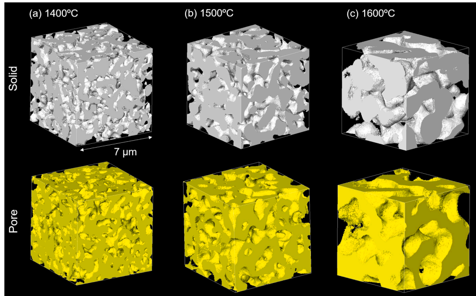
Fig. 8. 3D solid and pore structures within complex pores at (a) 1400°C, (b) 1500°C, and (c) 1600°C.
