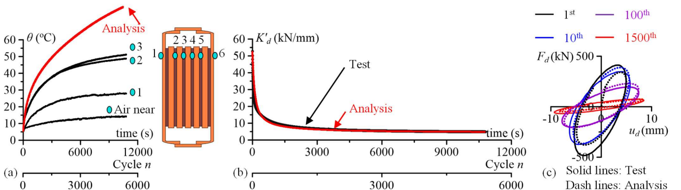
Figure 4. Analysis vs. Test: (a) time-history results of temperature, (b) storage stiffness and (c) hysteresis curves.
