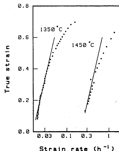
Fig. 7. True strain vs true strain rate calculated from the deformation curves.
