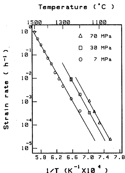
Fig. 4. Steady-state creep rate vs reciprocal absolute temperature for Y-TZP.
