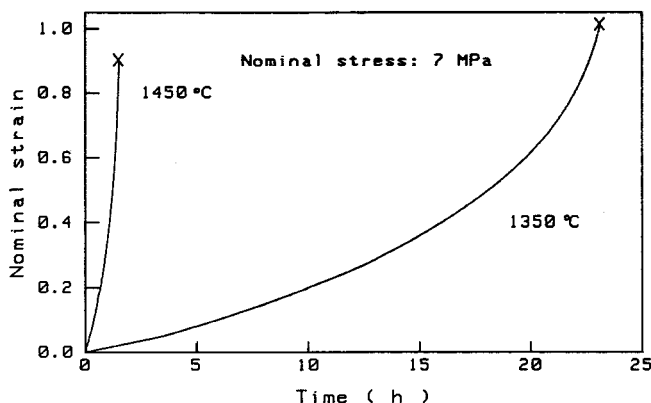
Fig. 5. Typical creep curves with a constant load corresponding to the nominal stress of 7 MPa showing large deformations during the accelerating creep.
