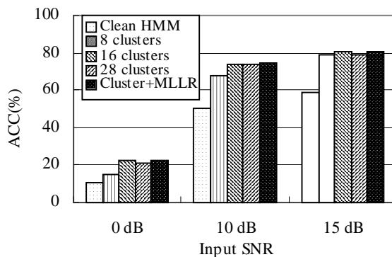
Fig. 5: Recognition results using PLT for Test-1 (crowd-noise-added speech).
