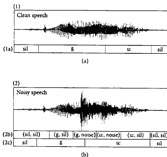
FIGURE 5: Segmentation for sound "gu:". Segmentations (1a) and (2c) are given by clean-speech HMMs. Segmentation (2b) is given by FHMM, where each unit is represented by a pair of speech and noise units.
