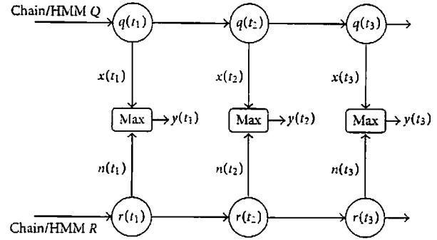
FIGURE 1: Structure of FHMM composed of two HMMs, Q and R .
