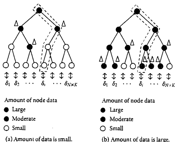
FIGURE 2: Tree structure for shifts estimation.
