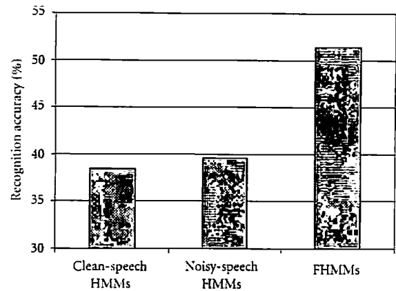
FIGURE 7: Recognition rates of clean HMMs (baseline), noisy HMMs, and noisy FHMMs for recorded noisy speech.
