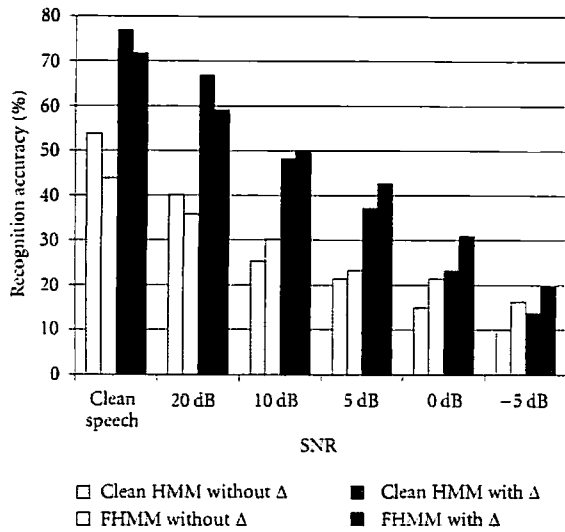
FIGURE 6: Recognition rates of speech artificially corrupted by sudden noise. HMMs (baseline) and the proposed method (noisy FHMMs) with and without \Delta features.
