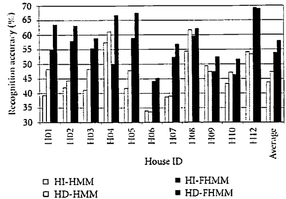
FIGURE 8: Results for supervised home-environment adaptation.
