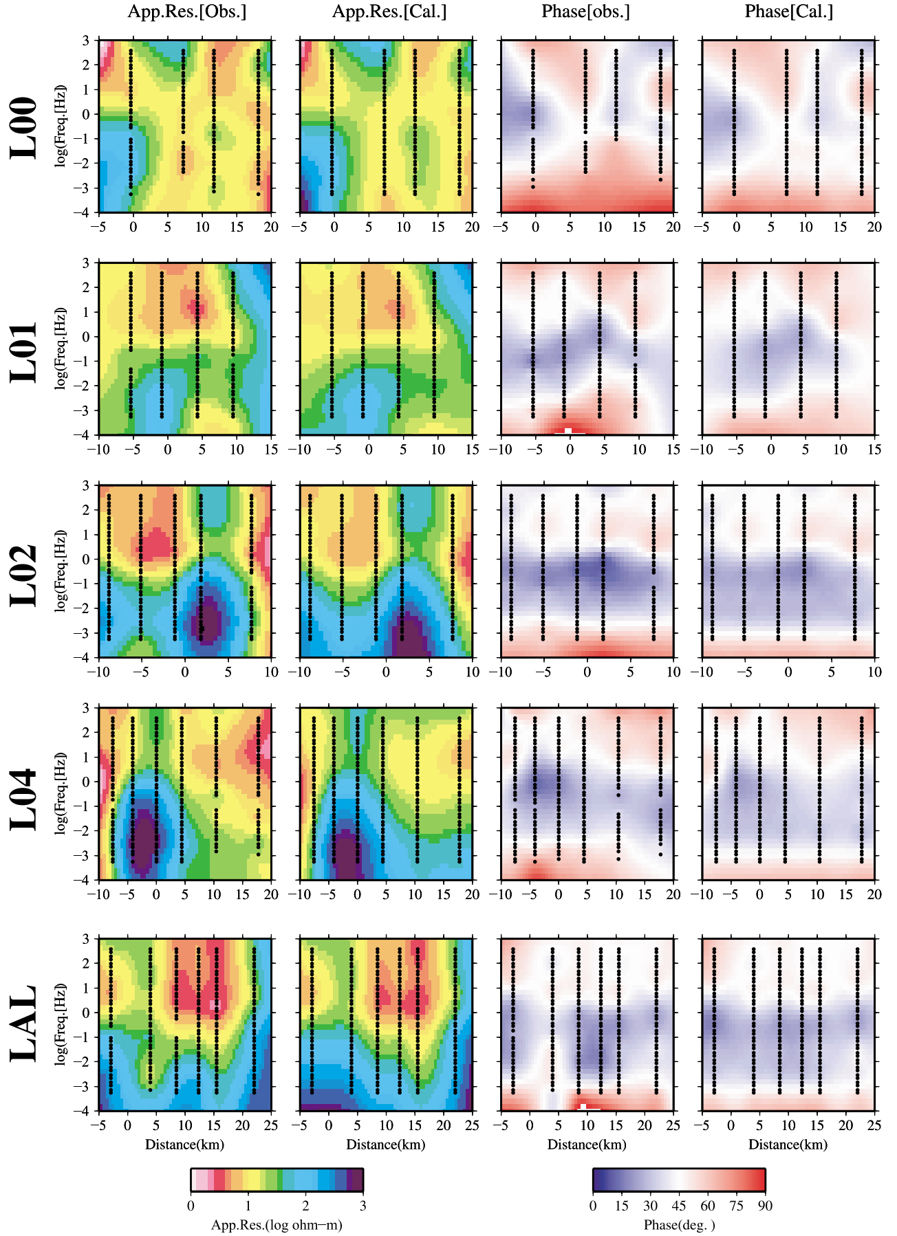
Fig. 3. Pseudo-sections for the observed and calculated data. Rows 1 to 5 show the profiles L00, L01, L02, L04 and LAL, respectively. Columns 1–4 are the observed and calculated apparent resistivity, and the observed and calculated phase for the TM mode, respectively.
