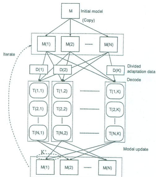
図 3: Aggregated (Ag) adaptation. ( T(n,k) : recognition hypothesis of the k -th subset made by using n -th Ag model)
