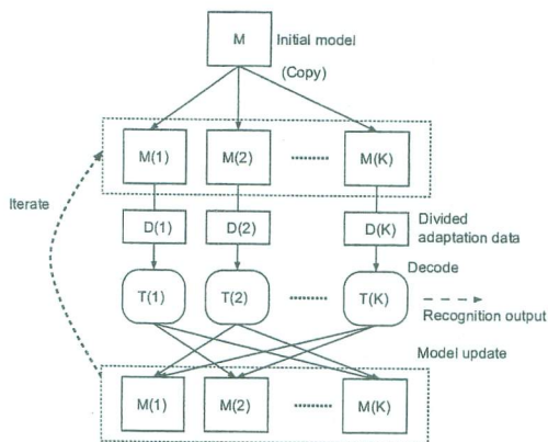
図 2: Cross-validation (CV) adaptation.
