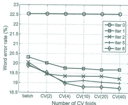
図 4: Number of cross-validation folds ( K ) of CV adaptation and recognition performance. The zeroth iteration is the result by the speaker independent model. (batch: batch-mode baseline adaptation result)
