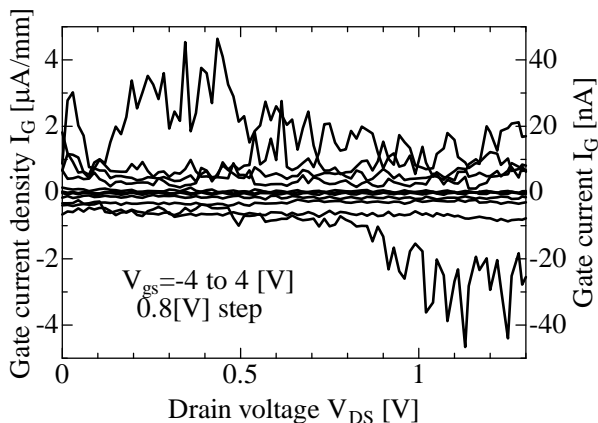
(b) Gate current
