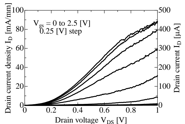
(a) Drain current
