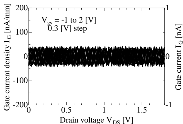
(b) Gate current
