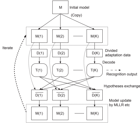
Fig. 1. Unsupervised cross-validation (CV) adaptation. M is a model, D(k) is the k -th Data subset, T is a transcript, D_k is a data subset excluding D(k) .
