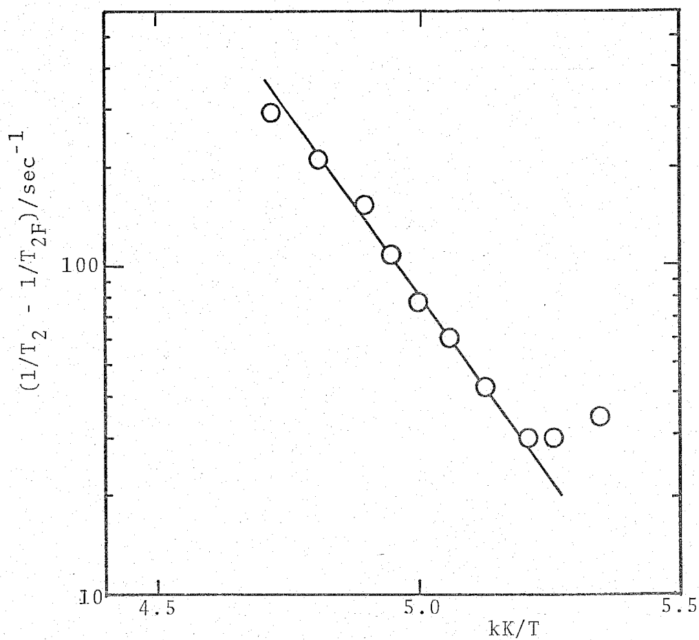
Fig. 3. A semilogarithmic plot of (1/T_2 - 1/T_{2F}) against the reciprocal temperature for the exchange of water in uranyl aqua complex. [\text{UO}_2^{2+}] = 0.139 \text{ M} , [\text{UO}_2^{2+}] : [\text{H}^+] : [\text{H}_2\text{O}] : [\text{CD}_3\text{COCD}_3] = 1 : 0.15 : 13.0 : 93.6 .
