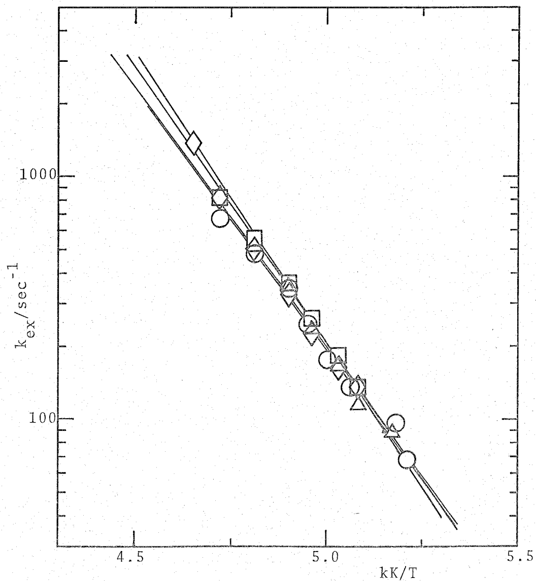
Fig. 4. Semilogarithmic plots of k_{\text{ex}} against the reciprocal temperature for the exchange of water in uranyl aqua complex. The symbols of ○, △, □, and ◇ correspond to (i), (ii), (iii), and (iv) in Table 1.
