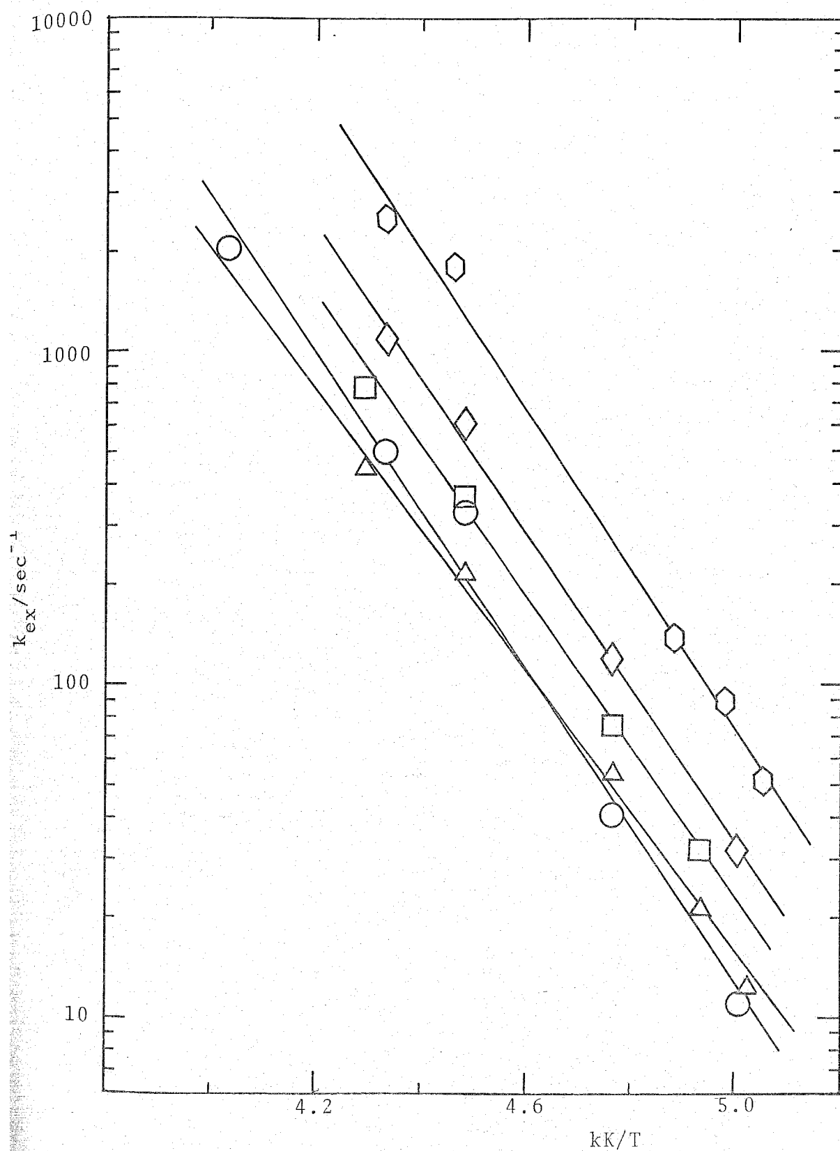
Fig. 15. Semilogarithmic plots of k_{\text{ex}} against the reciprocal temperature for the exchange of DMF in \text{UO}_2(\text{DMF})_5^{2+} . The symbols of ○, △, □, ◇, and ⬡ correspond to (i), (ii), (iii), (iv), and (v) in Table 7.
