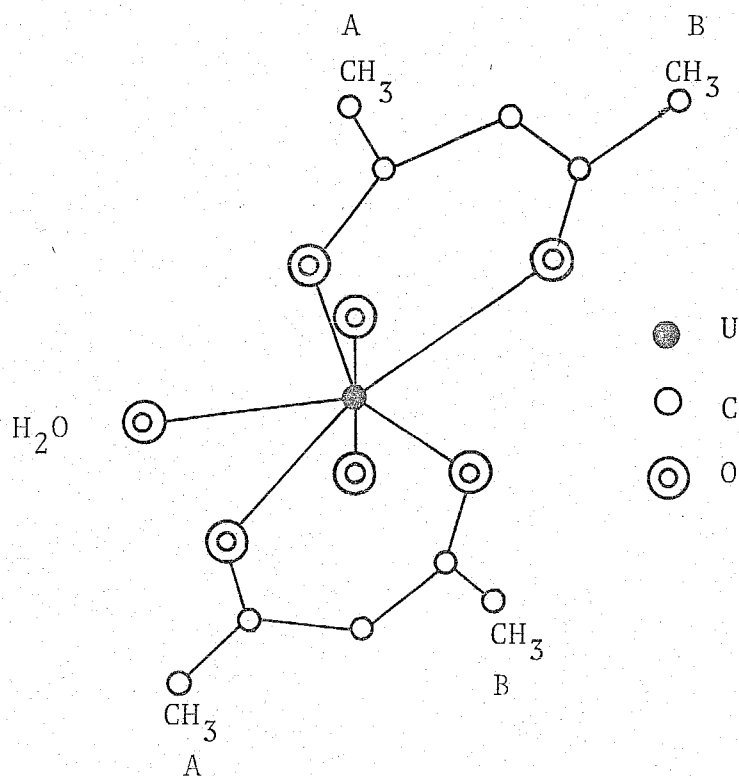
Fig. 1. The perspective view of the structure of \text{UO}_2(\text{acac})_2\text{H}_2\text{O} complex. The U-O bond lengths are 2.51 \pm 0.07 \text{ \AA} for the oxygen atoms in the rings, 2.48 \pm 0.07 \text{ \AA} for water oxygen and 1.60 \pm 0.07 \text{ \AA} for the oxygen atoms in the uranyl group. E. Frasson, G. Bombieri and C. Panattoni, Coord. Chem. Rev. , 1 , 145(1966).
