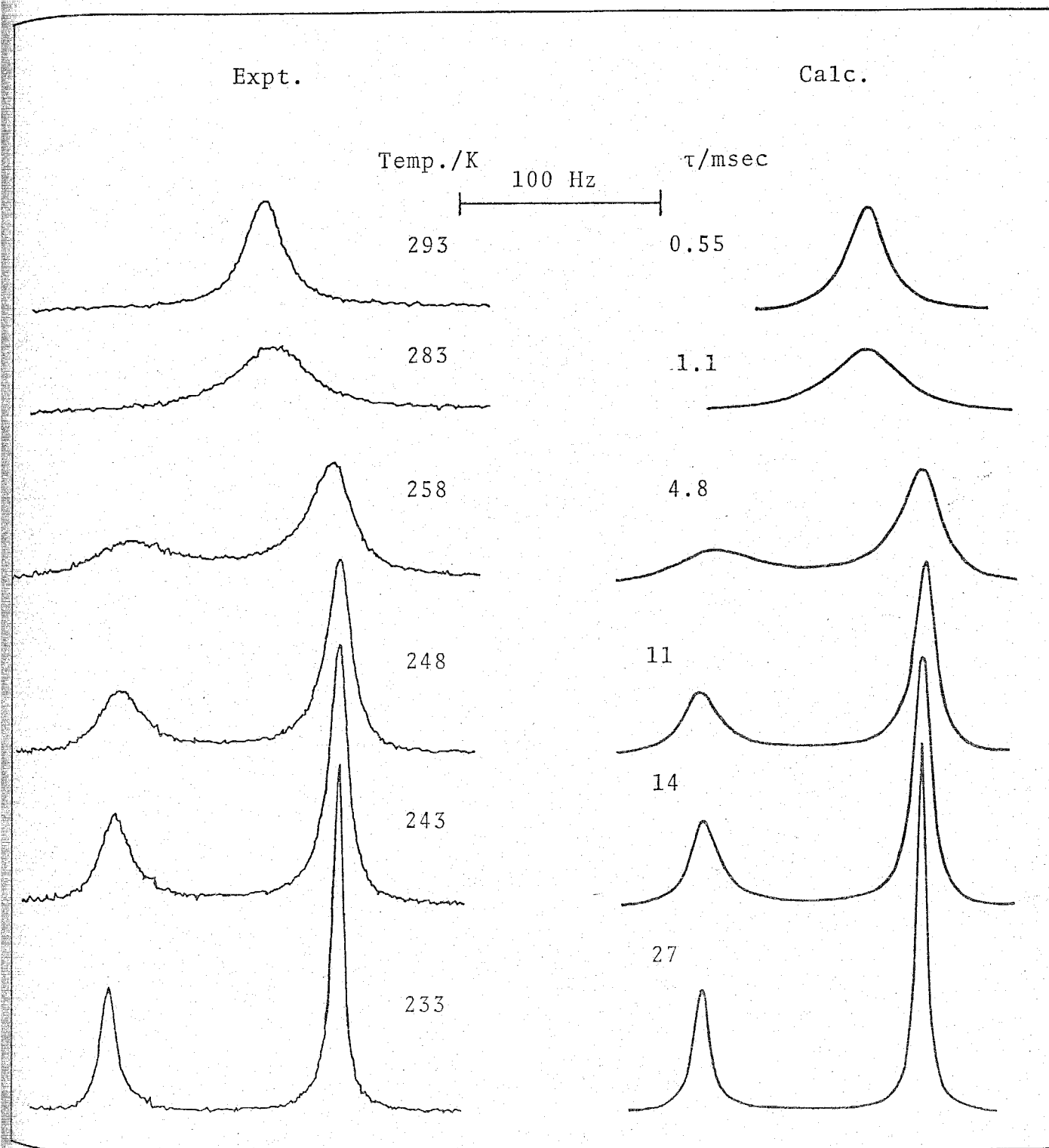
Fig. 22. Experimental(left-hand side) and best-fit calculated ^1\text{H} NMR lineshapes of a solution consisting of \text{UO}_2(\text{acac})_2\text{DMF}(0.116 \text{ M}) , \text{DMF}(0.215 \text{ M}) , and \text{CD}_2\text{Cl}_2(14.7 \text{ M}) . Temperatures and best-fit \tau -values are shown at the center of the figure.
