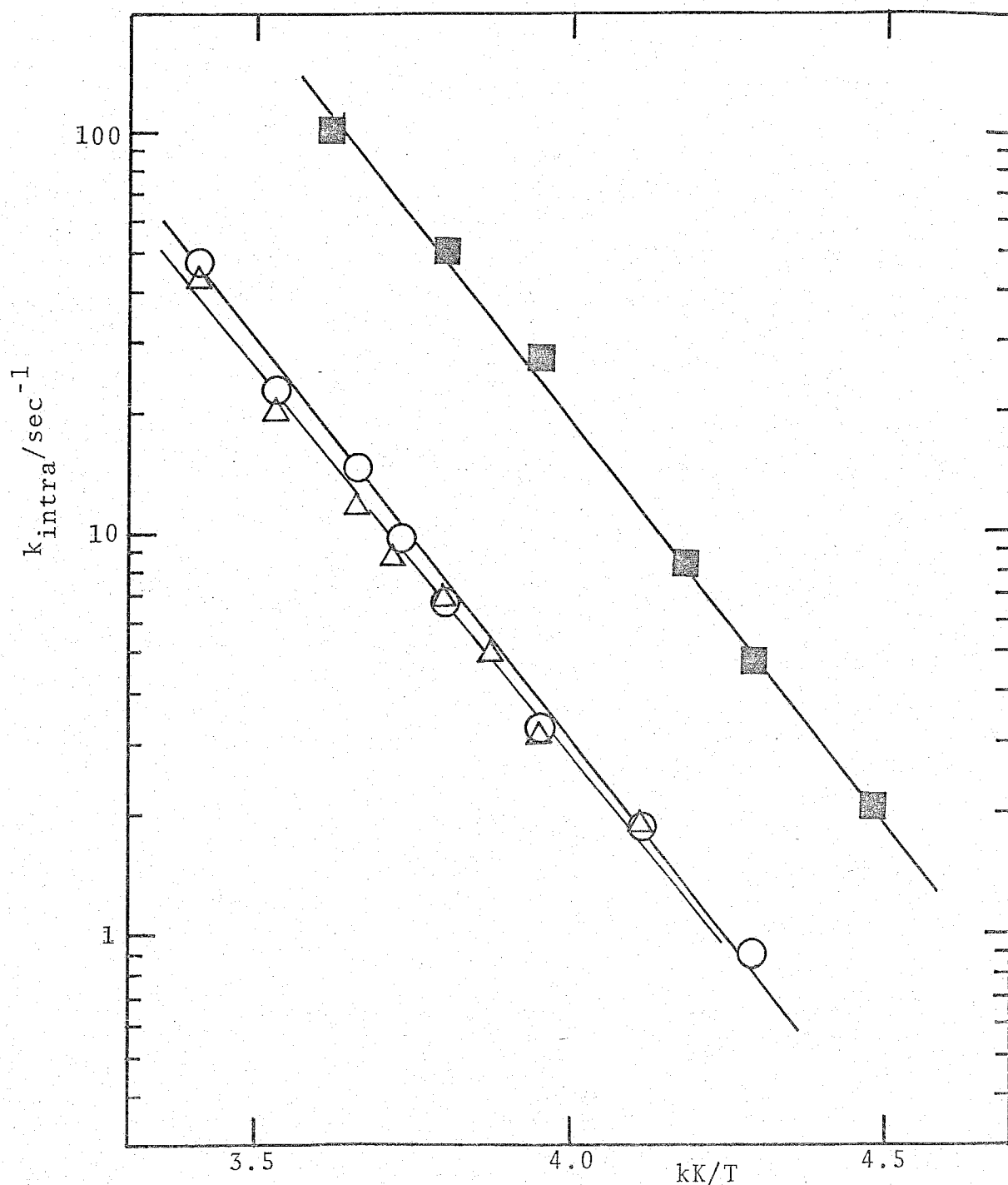
Fig. 14. Semilogarithmic plots of k_{\text{intra}} against the reciprocal temperature for the exchange of methyl groups of acac in \text{UO}_2(\text{acac})_2\text{L} (L= DMF and DEF). \bigcirc : \text{UO}_2(\text{acac})_2\text{DMF} in \text{CD}_2\text{Cl}_2 ; \blacksquare : \text{UO}_2(\text{acac})_2\text{DMF} in \text{CD}_3\text{COCD}_3 ; \triangle : \text{UO}_2(\text{acac})_2\text{DEF} in \text{CD}_2\text{Cl}_2 .
