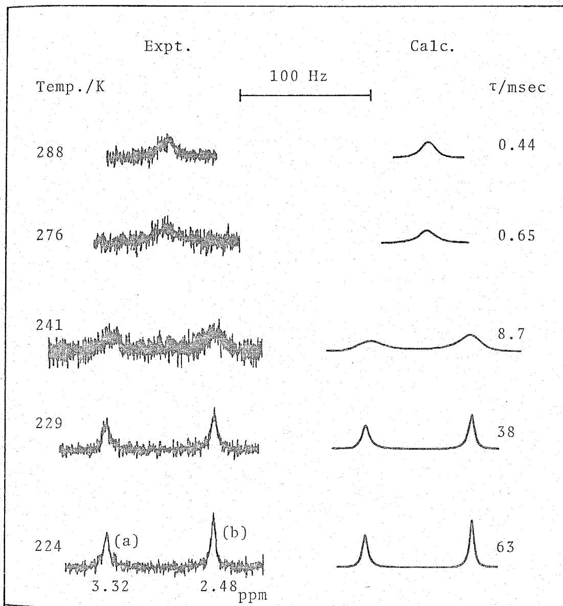
Fig. 9. Experimental(left-hand side) and best-fit calculated ^1\text{H} NMR lineshapes of a solution consisting of \text{UO}_2(\text{DMSO})_5^{2+}
