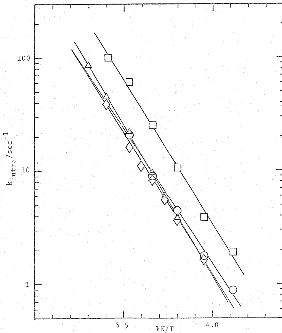
Fig. 9. Semilogarithmic plots of k_{\text{intra}} against the reciprocal temperature for the exchange of methyl groups of acac in \text{UO}_2(\text{acac})_2\text{DMSO} . \circ : \text{CD}_2\text{Cl}_2 ; \triangle : o\text{-C}_6\text{H}_4\text{Cl}_2 ; \square : \text{CD}_3\text{COCD}_3 ; \diamond : \text{CD}_3\text{NO}_2 .
