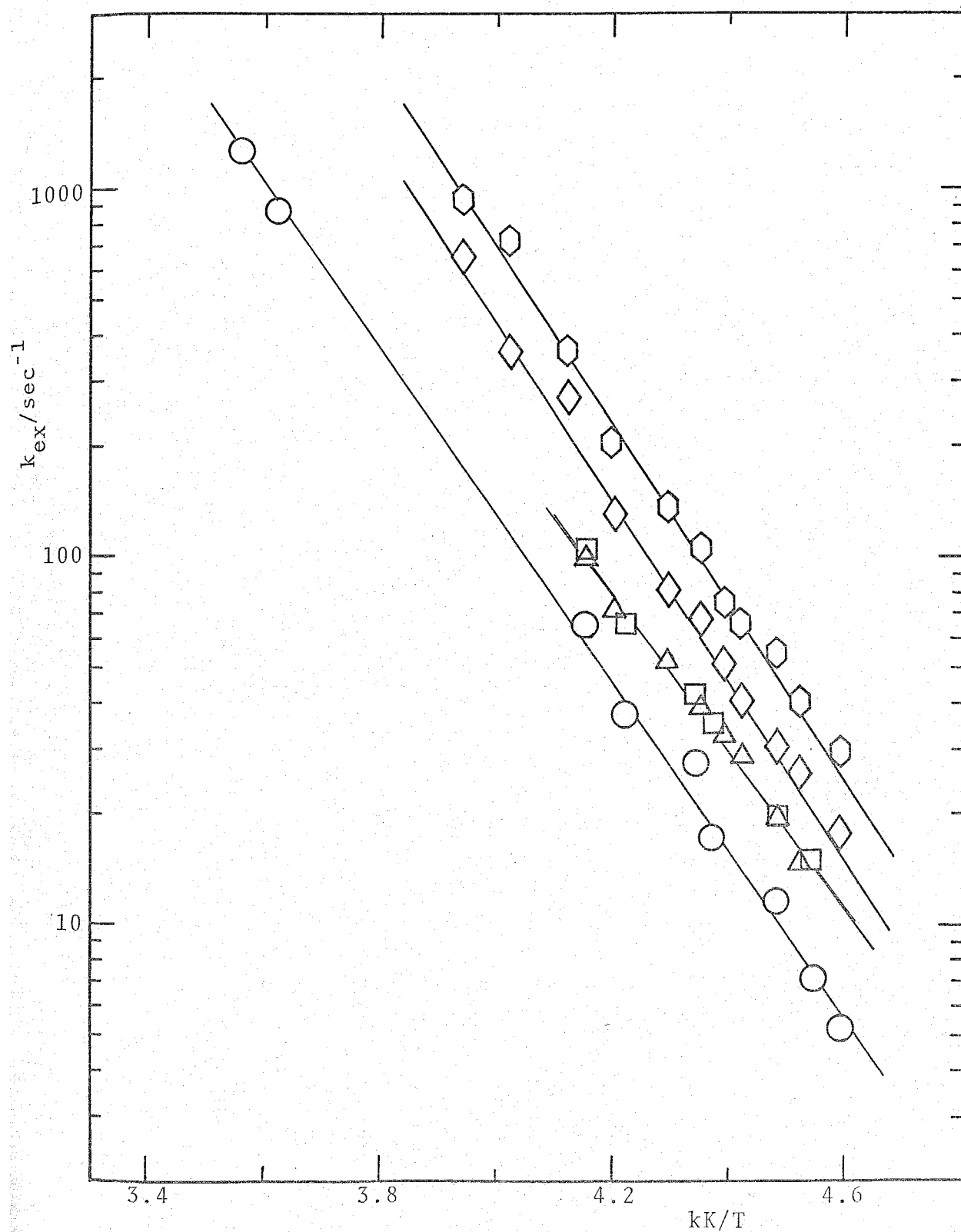
Fig. 10. Semilogarithmic plots of k_{\text{ex}} against the reciprocal temperature for the exchange of DMSO in \text{UO}_2(\text{DMSO})_5^{2+} . The symbols of ○, △, □, ◇, and ⬡ correspond to (i), (ii), (iii), (iv), and (v) in Table 4.
