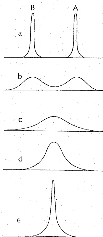
Fig. 1. Lineshapes of NMR signals as a function of exchange rate in the two site exchange reaction.
