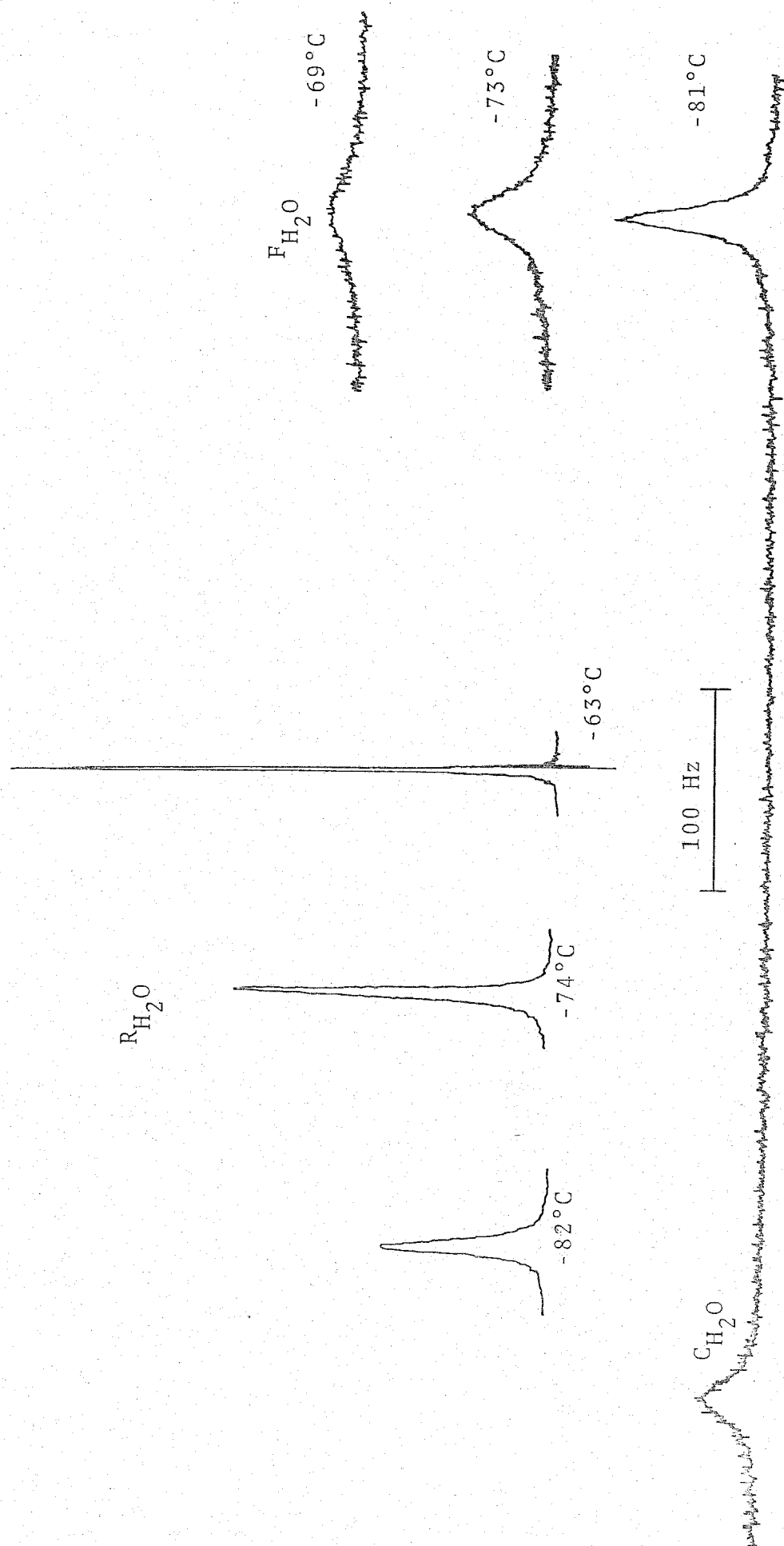
Fig. 2. Temperature dependence of ^1\text{H} NMR spectra of bulk water in the presence of uranyl ion and of water in the absence of uranyl ion in \text{CD}_3\text{COCD}_3 .
