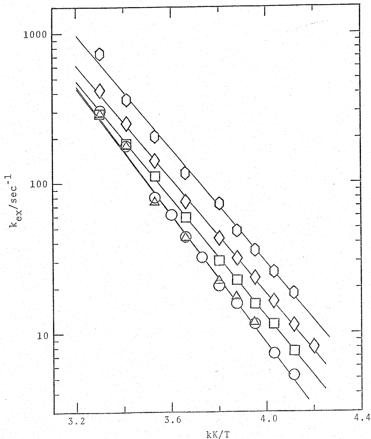
Fig. 7. Semilogarithmic plots of k_{\text{ex}} against the reciprocal temperature for the exchange of DMSO in \text{UO}_2(\text{acac})_2 DMSO in \text{CD}_2\text{Cl}_2 . The symbols of \bigcirc , \triangle , \square , \diamond , and \hexagon correspond to (i), (ii), (iii), (iv), and (v) in Table 3.
