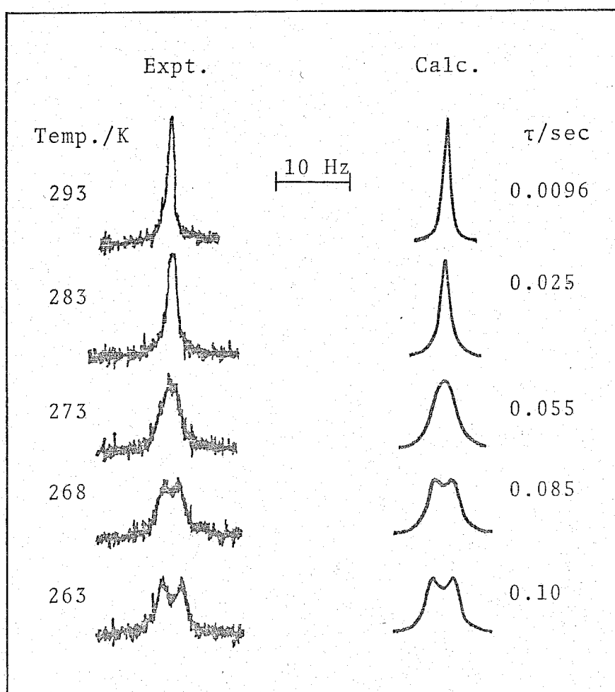
Fig. 5. Experimental(left-hand side) and best-fit calculated ^1\text{H} NMR lineshapes of \text{UO}_2(\text{acac})_2\text{DMSO} (0.0349 m) in o\text{-C}_6\text{H}_4\text{Cl}_2 . Temperatures and best-fit \tau -values are shown at the left- and right-hand sides of the figure, respectively.
