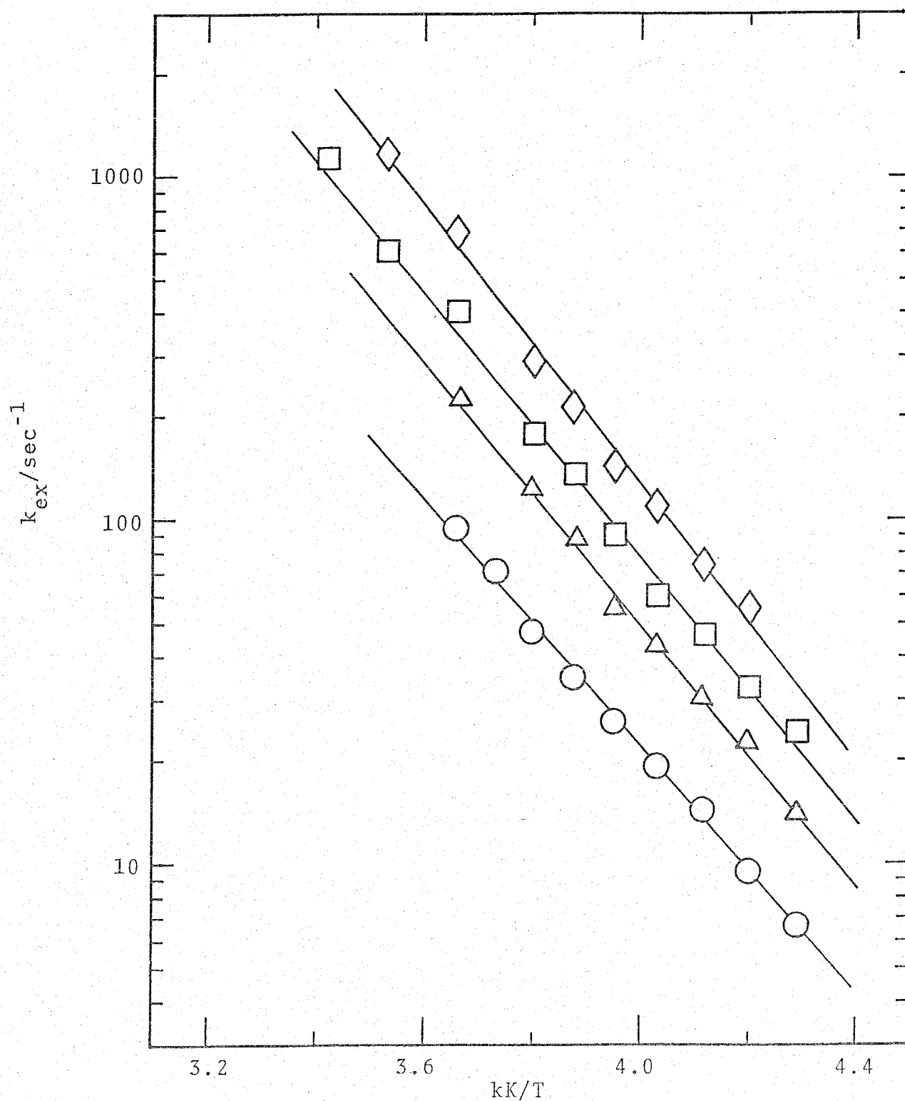
Fig. 23. Semilogarithmic plots of k_{\text{ex}} against the reciprocal temperature for the exchange of DMF in \text{UO}_2(\text{acac})_2\text{DMF}
