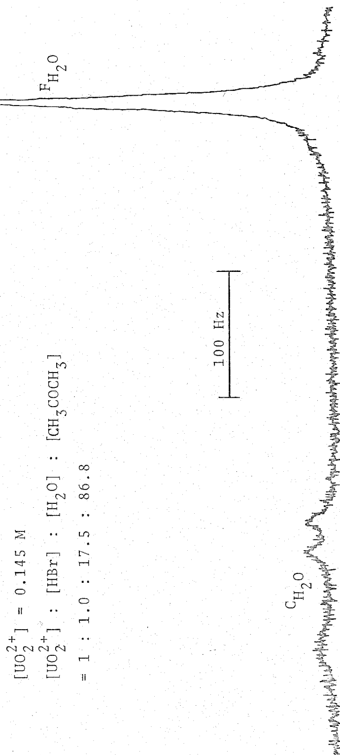
Fig. 7. The ^1\text{H} NMR spectrum of solution consisting of \text{UO}_2(\text{ClO}_4)_2 , \text{HBr} , \text{H}_2\text{O} and \text{CH}_3\text{COCH}_3 at -90^\circ\text{C} .
