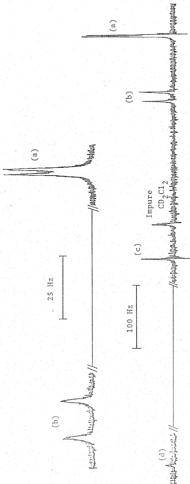
Fig. 10. The ^1\text{H} NMR spectrum of \text{UO}_2(\text{acac})_2\text{DMF} (0.0364 m) in \text{CD}_2\text{Cl}_2 at -40^\circ\text{C} .
