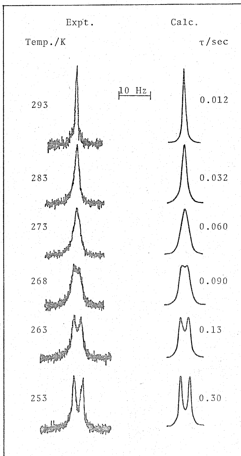
Fig. 6. Experimental (left-hand side) and best-fit calculated ^1\text{H} NMR lineshapes of \text{UO}_2(\text{acac})_2 \cdot \text{DMSO} (0.0417 m) in \text{CD}_3\text{NO}_2 . Temperatures and best-fit \tau -values are shown at the
