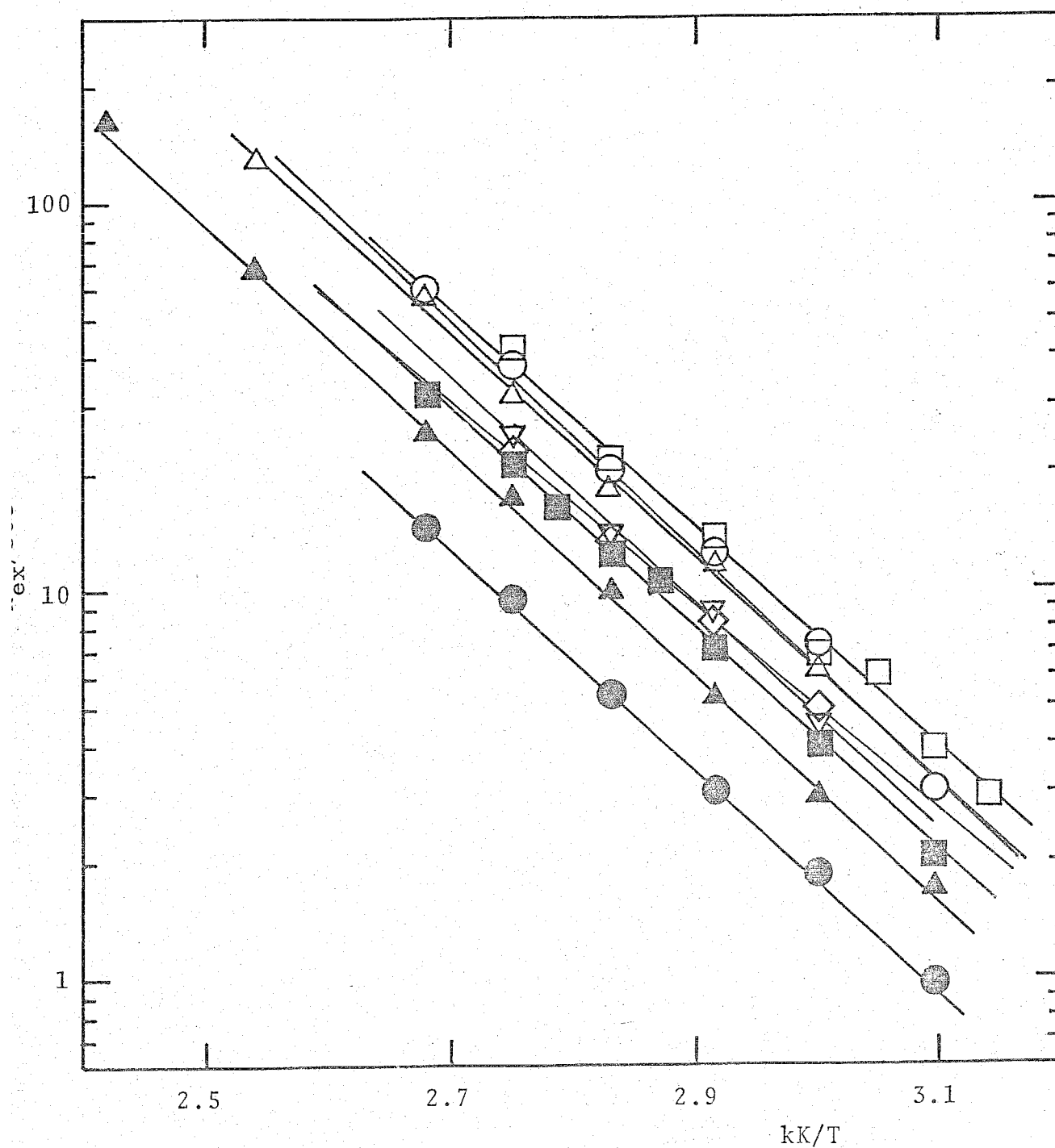
g. 4. Semilogarithmic plots of k_{\text{ex}} against the reciprocal temperature for the exchange of acac in \text{UO}_2(\text{acac})_2\text{DMSO} . The symbols of ●, ▲, ■, ○, △, □, ◇, and ▽ correspond to (i), (ii), (iii), (iv), (v), (vi), (vii), and (viii) in Table 1, respectively.
