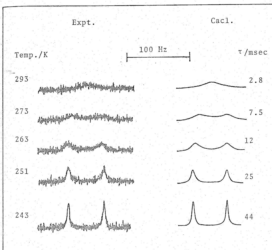
3. 14. Experimental (left-hand side) and best-fit calculated ^1\text{H} NMR lineshapes of a solution consisting of \text{UO}_2(\text{dbm})_2 DMSO (0.0637 M), DMSO (0.0627 M), and \text{CD}_2\text{Cl}_2 (14.8 M). Temperatures and best-fit \tau -values are shown at left- and right-hand sides of the figure, respectively.
