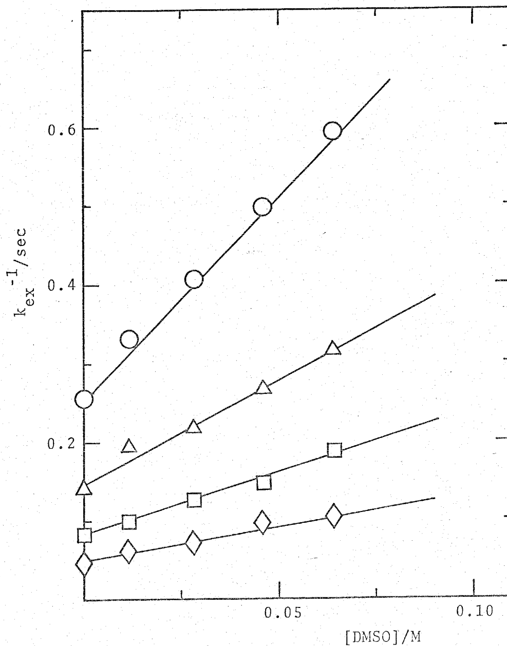
Fig. 9. Plots of 1/k_{\text{ex}} vs. [\text{DMSO}] for the effect of added DMSO on the exchange of acac in \text{UO}_2(\text{acac})_2\text{DMSO} . \bigcirc : 60 °C; \triangle : 70 °C; \square : 80 °C; \diamond : 90 °C.
