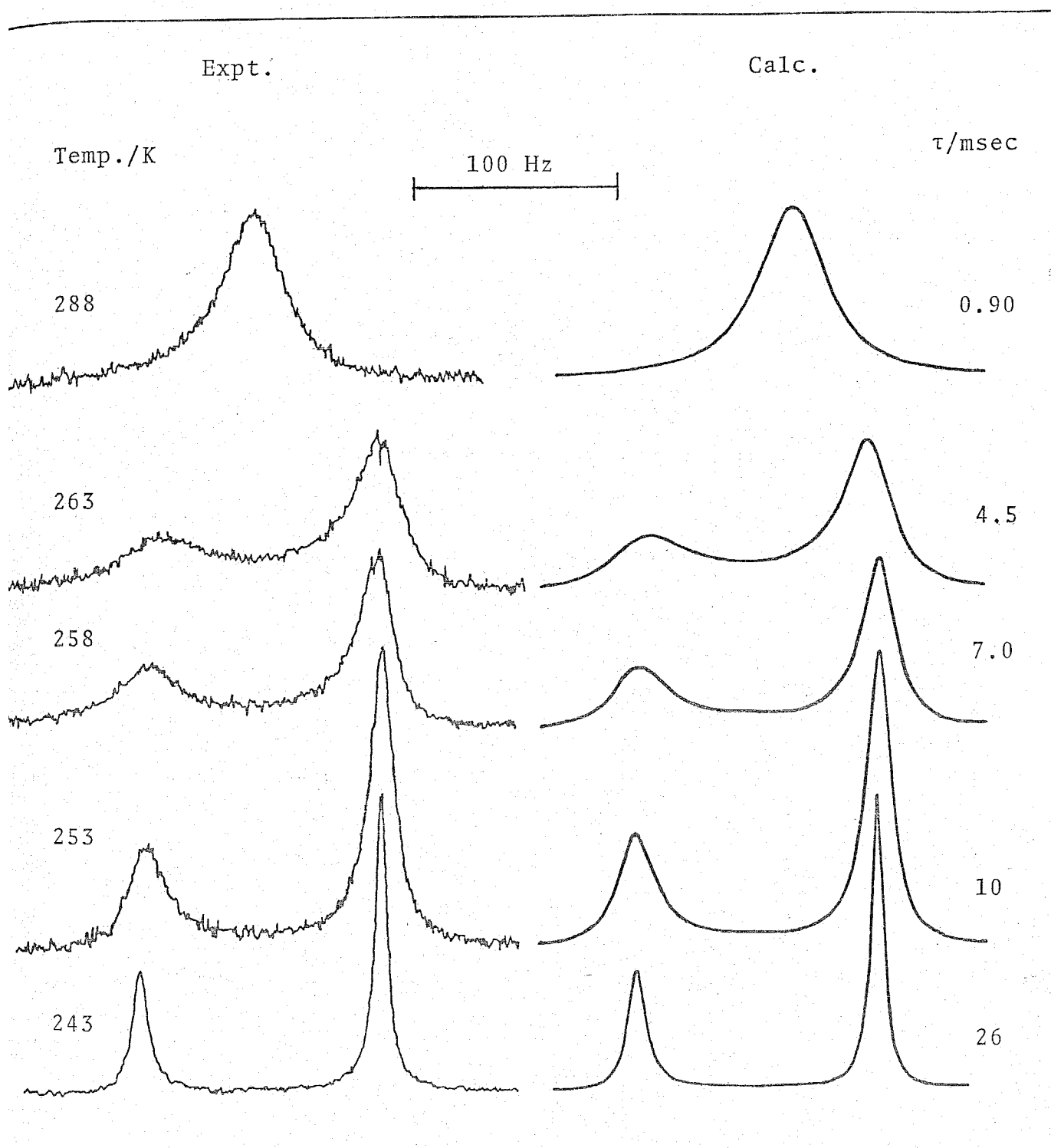
Fig. 20. Experimental(left-hand side) and best-fit calculated ^1\text{H} NMR lineshapes of a solution consisting of \text{UO}_2(\text{acac})_2\text{DMF}(0.0661\text{ M}) , \text{DMF}(0.112\text{ M}) , and \text{CD}_3\text{COCD}_3(13.3\text{ M}) . Temperatures and best-fit \tau -values are shown at the left- and right-hand sides of the figure respectively.
