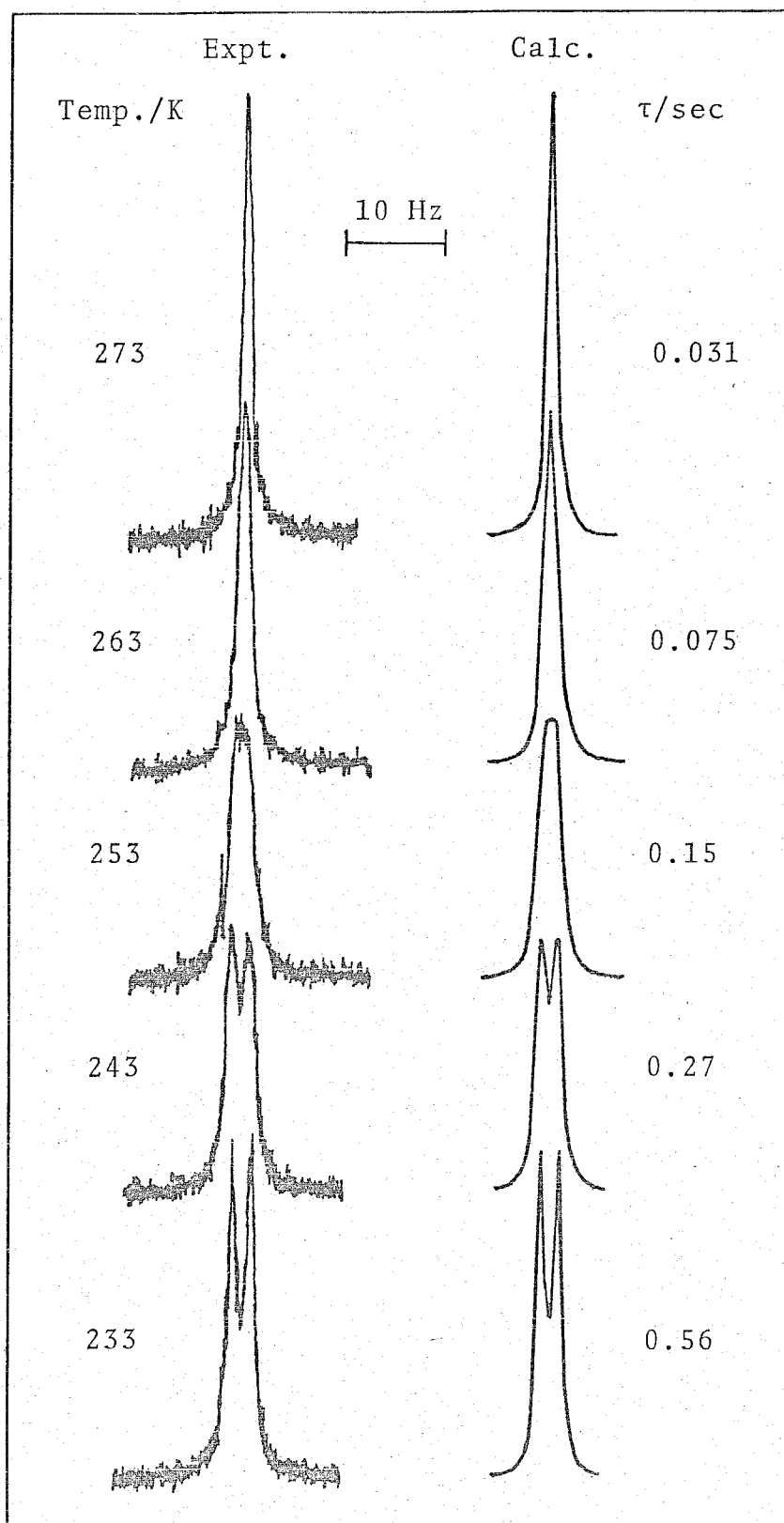
Fig. 12. Experimental(left-hand side) and best-fit calculated ^1\text{H} NMR lineshapes of \text{UO}_2(\text{acac})_2\text{DMF} (0.0364 m) in \text{CD}_2\text{Cl}_2 . Temperatures and best-fit \tau -values are shown at the left- and right-hand sides of the figure, respectively.
