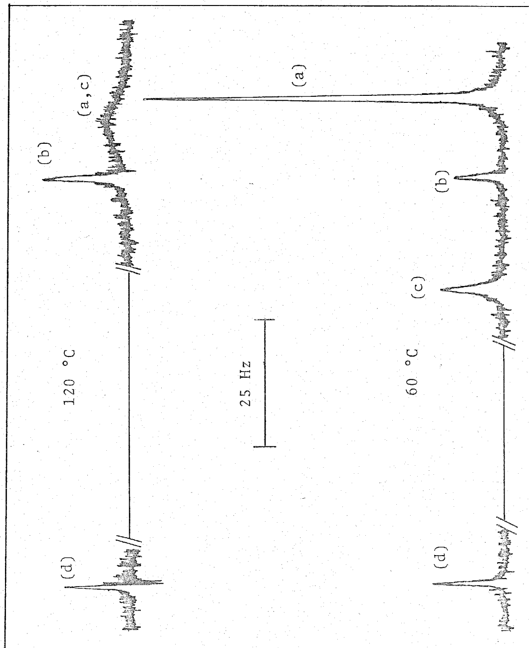
Fig. 1. The ^1\text{H} NMR spectra of a solution consisting of \text{UO}_2(\text{acac})_2 in \text{DMSO} ( 0.0679\text{ M} ), \text{Hacac} ( 0.487\text{ M} ), and o\text{-C}_6\text{H}_4\text{Cl}_2 ( 8.62\text{ M} ) at 60 and 120\text{ }^\circ\text{C} , respectively.
