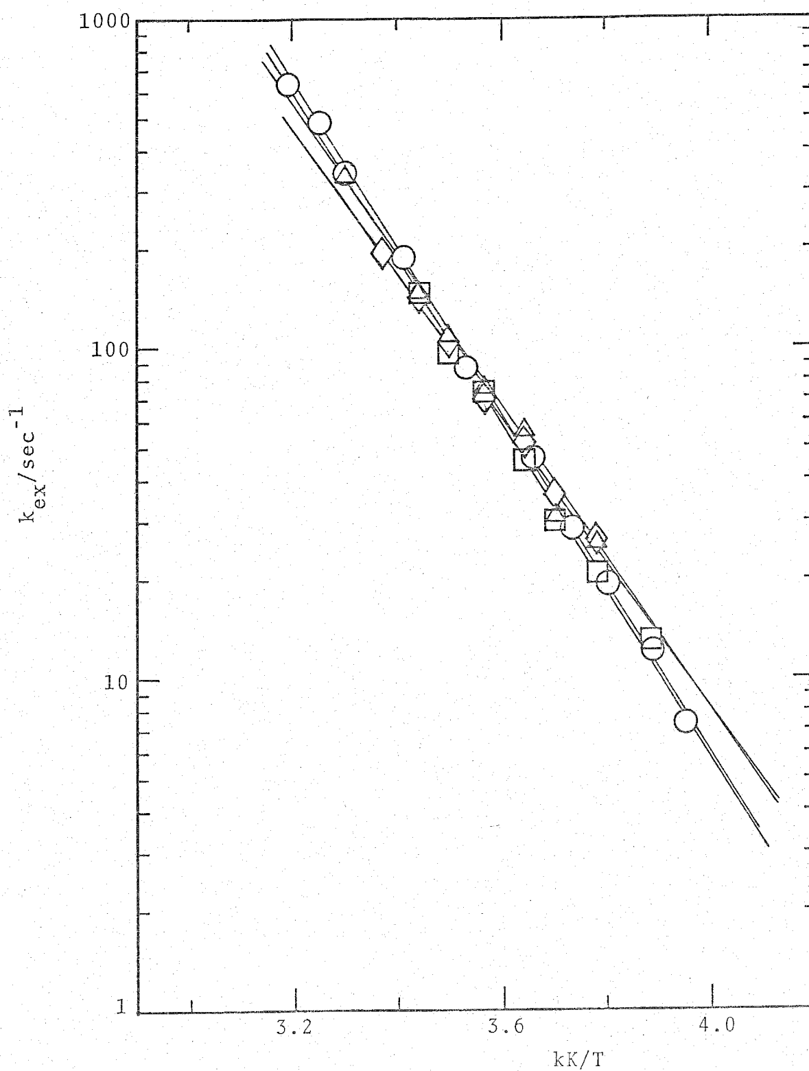
Fig. 5. Semilogarithmic plots of k_{\text{ex}} against the reciprocal temperature for the exchange of DMSO in \text{UO}_2(\text{acac})_2 DMSO in \text{CD}_3\text{COCD}_3 . The symbols of ○, △, □, and ◇ correspond to (i), (ii), (iii), and (iv) in Table 1.
