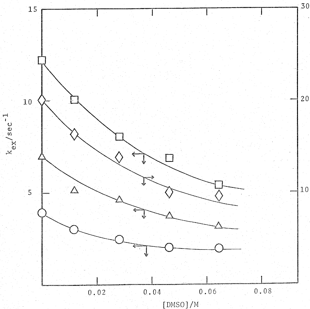
Fig. 8. Plots of k_{\text{ex}} vs. [\text{DMSO}] for the effect of added DMSO on the exchange of acac in \text{UO}_2(\text{acac})_2\text{DMSO} .
