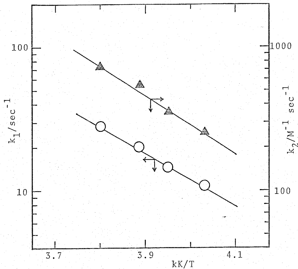
Fig. 25. Semilogarithmic plots of k_1 and k_2 against the reciprocal temperature for the exchange of DMF in \text{UO}_2(\text{acac})_2\text{DMF} in \text{CD}_2\text{Cl}_2 .
