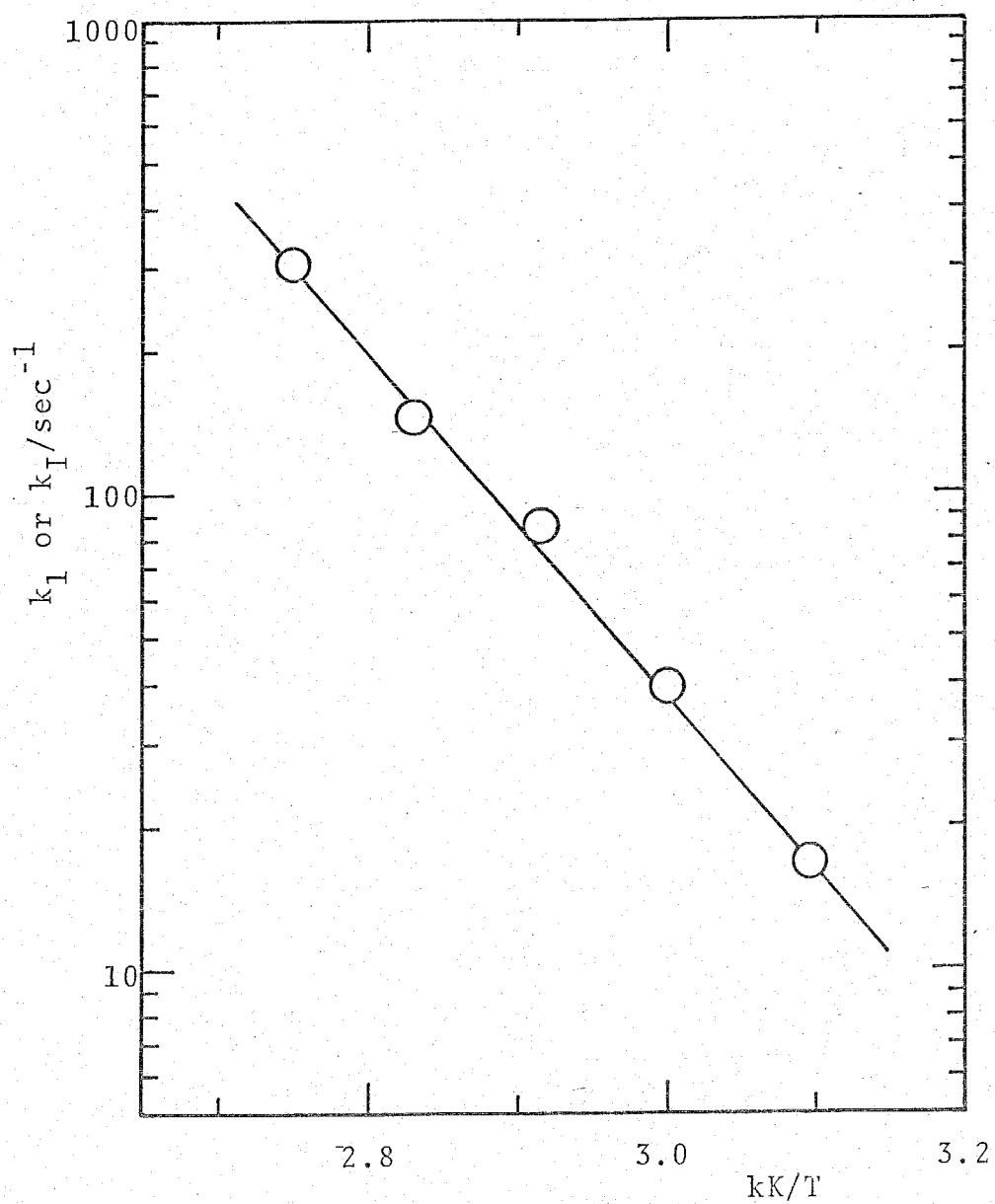
Fig. 10. A semilogarithmic plot of k_I or k_{I'} against the reciprocal temperature for the exchange of acac in \text{UO}_2(\text{acac})_2\text{DMSO} .
