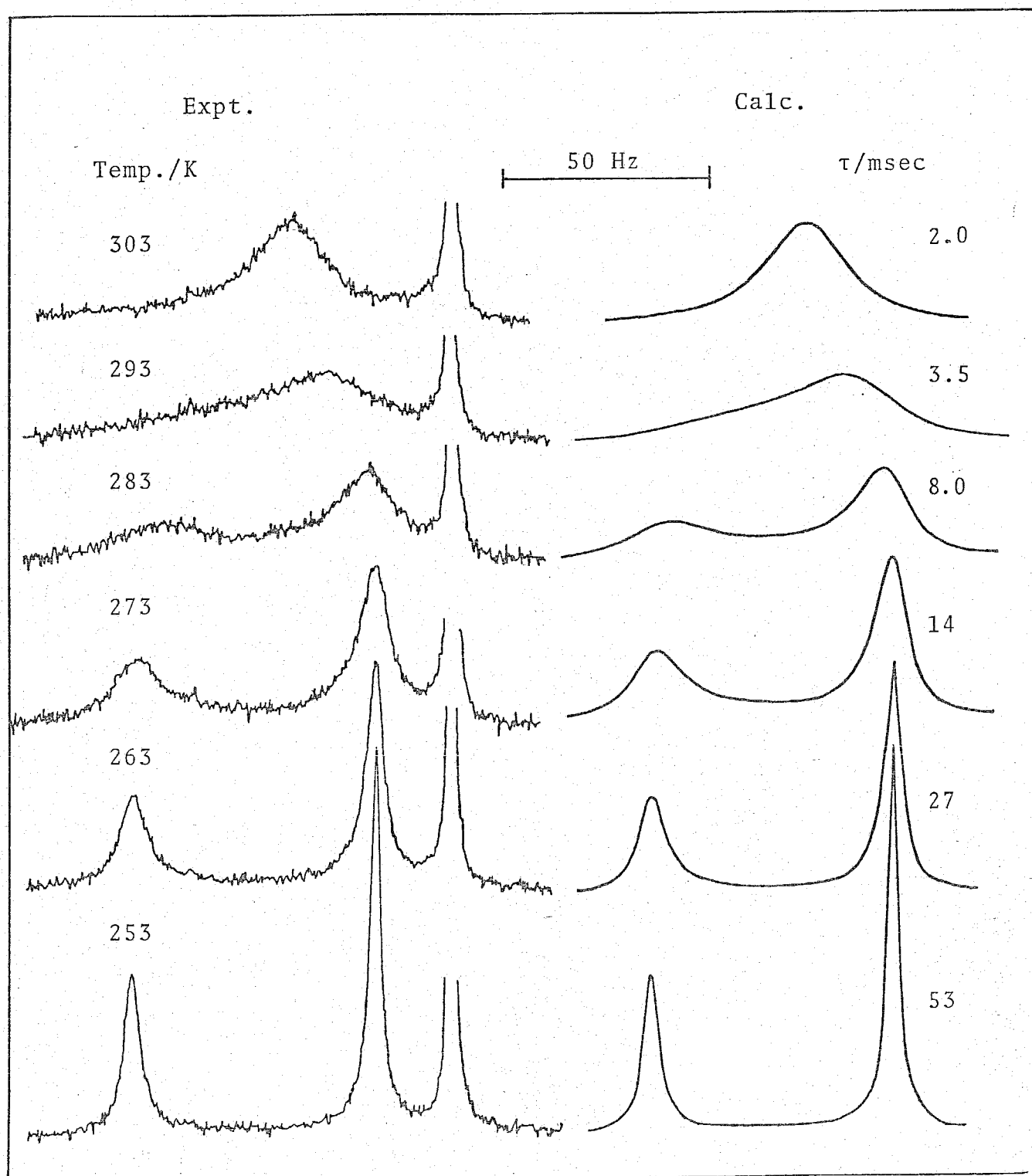
6. Experimental(left-hand side) and best-fit calculated ^1\text{H} NMR lineshapes of a solution consisting of \text{UO}_2(\text{acac})_2 DMSO(0.0179 M), DMSO(0.0282 M), and \text{CD}_2\text{Cl}_2 (15.8 M). Temperatures and best-fit \tau -values are shown at left- and right-hand sides of the figure,
