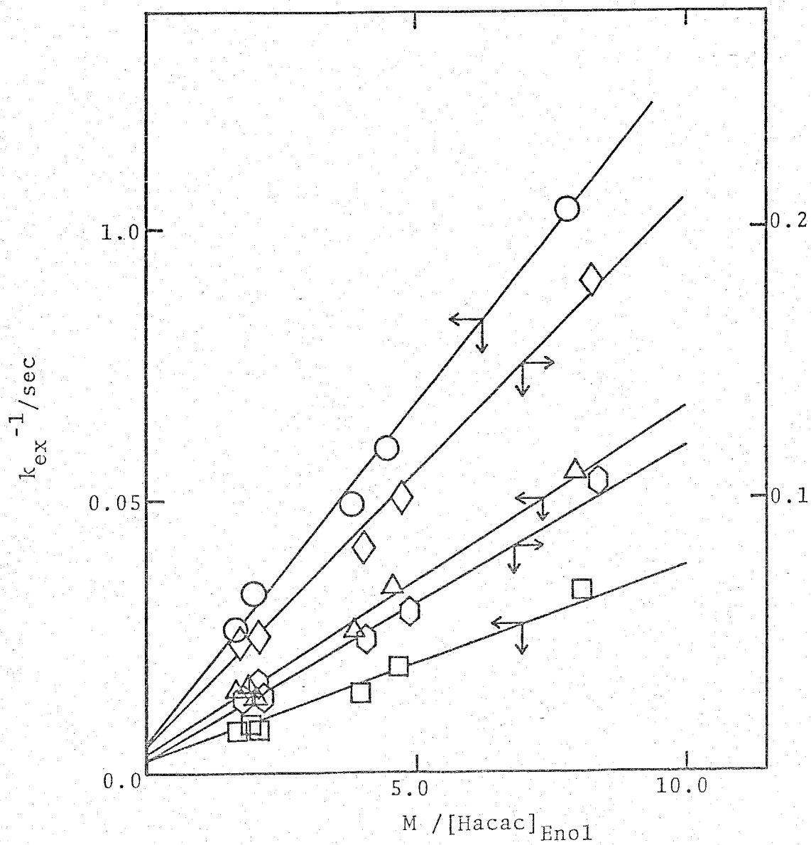
Fig. 6. Plots of 1/k_{\text{ex}} vs. 1/[\text{Hacac}]_{\text{Enol}} for the exchange of acac in \text{UO}_2(\text{acac})_2\text{DMSO} . \bigcirc : 50 °C; \triangle : 60 °C; \square : 70 °C; \diamond : 80 °C; \hexagon : 90 °C.
