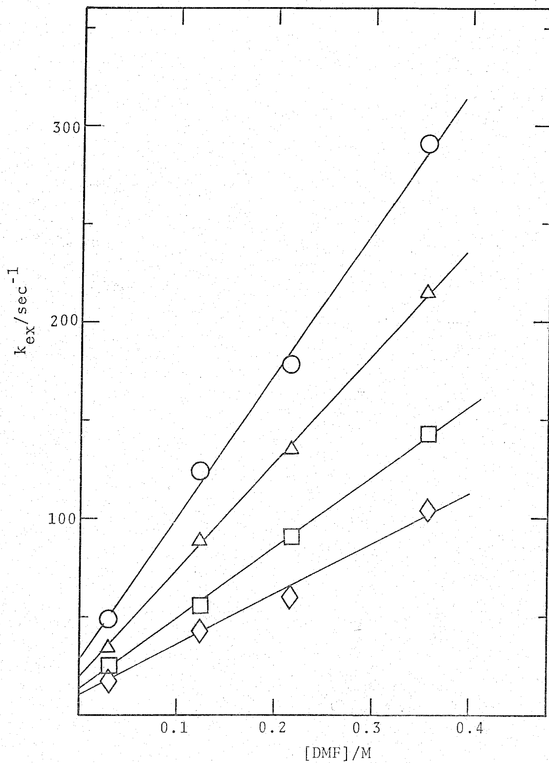
Fig. 24. Plots of k_{ex} vs. [DMF] for the exchange of DMF in UO_2(acac)_2DMF in CD_2Cl_2 . ○ : -10 °C; △ : -15 °C; ◇ : -25 °C.
