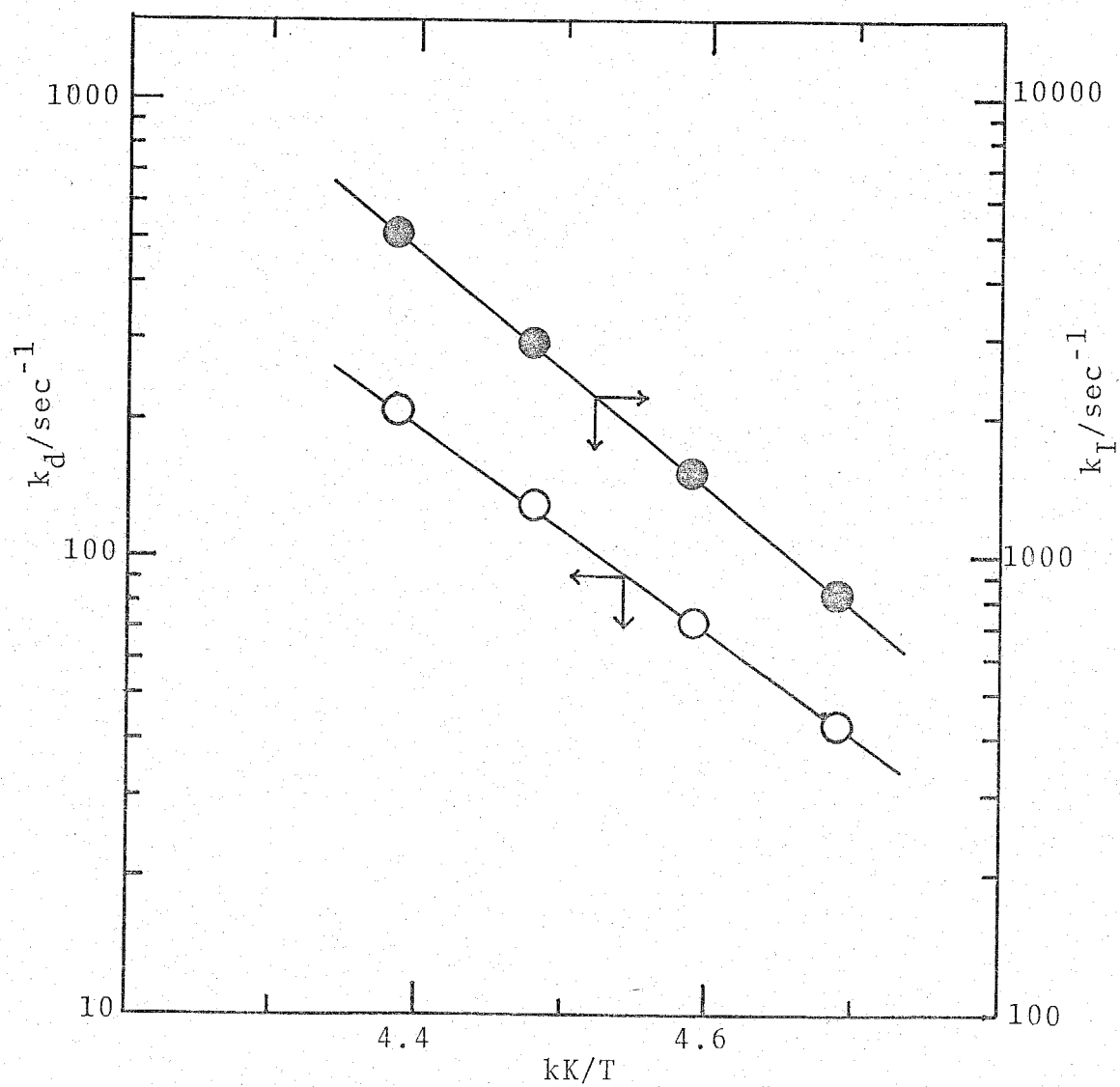
Fig. 17. Semilogarithmic plots of k_d and k_I against the reciprocal temperature for the exchange of DMF in \text{UO}_2(\text{DMF})_5^{2+} .
