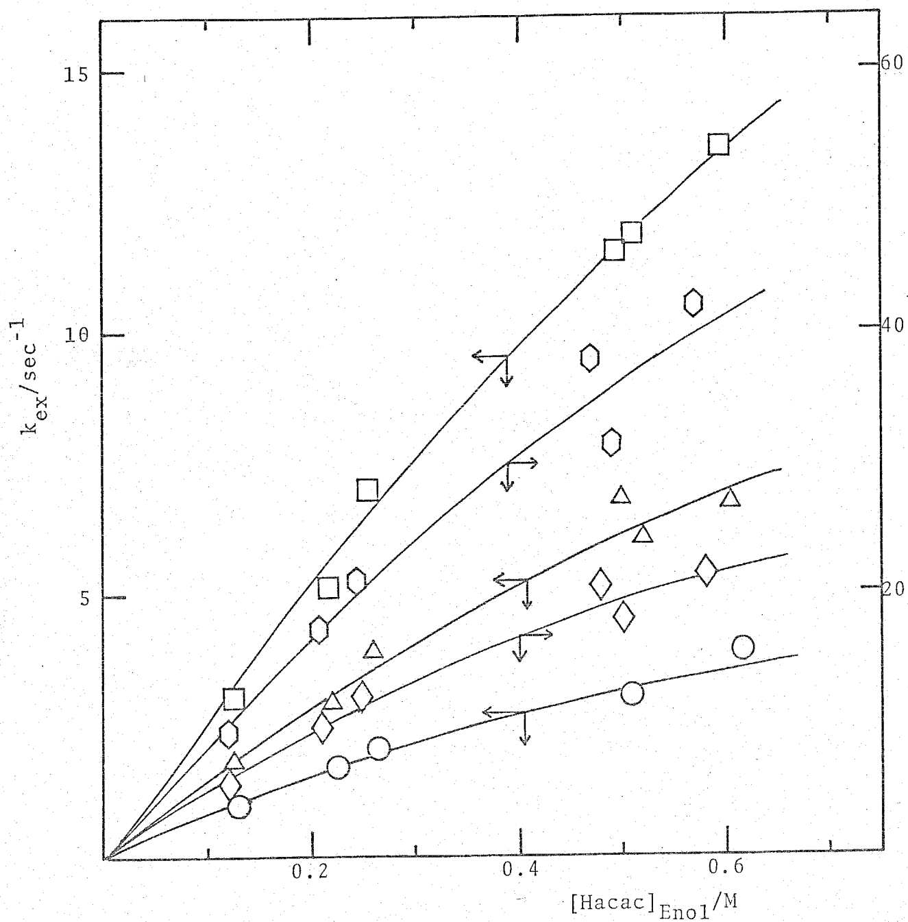
Fig. 5. Plots of k_{\text{ex}} vs. [\text{Hacac}]_{\text{Enol}} for the exchange of acac in \text{UO}_2(\text{acac})_2 \cdot \text{DMSO} . \bigcirc : 50 °C; \triangle : 60 °C; \square : 70 °C; \diamond : 80 °C; \hexagon : 90 °C.
