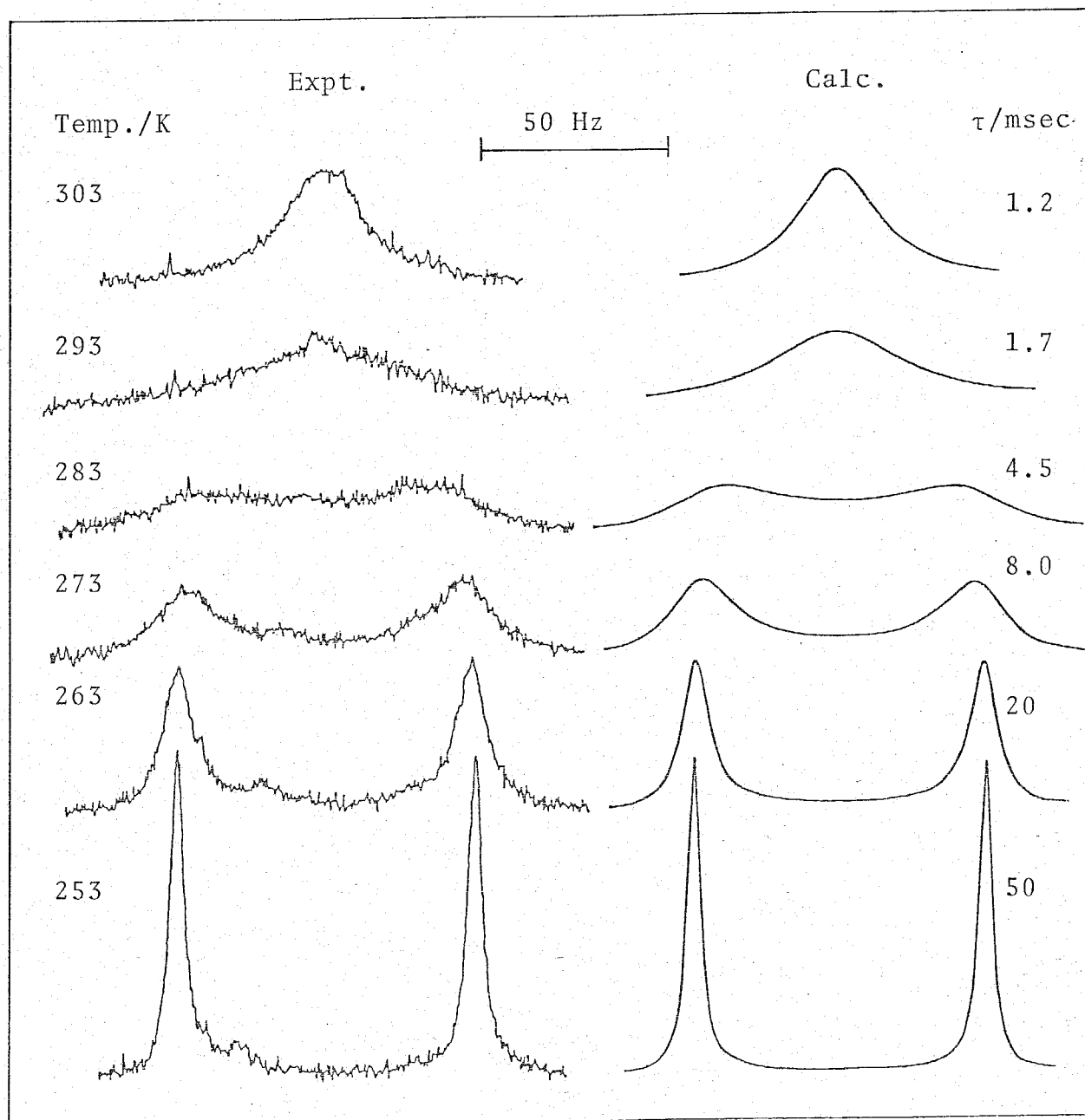
Fig. 12. Experimental(left-hand side) and best-fit calculated ^1\text{H} NMR lineshapes of a slution consisting of \text{UO}_2(\text{dbm})_2 DMSO (0.0117 M), DMSO(0.0115 M), and \text{CD}_3\text{COCD}_3 (13.5 M). Temperatures and best-fit \tau -values are shown at left- and right-hand sides of the figure, respectively.
