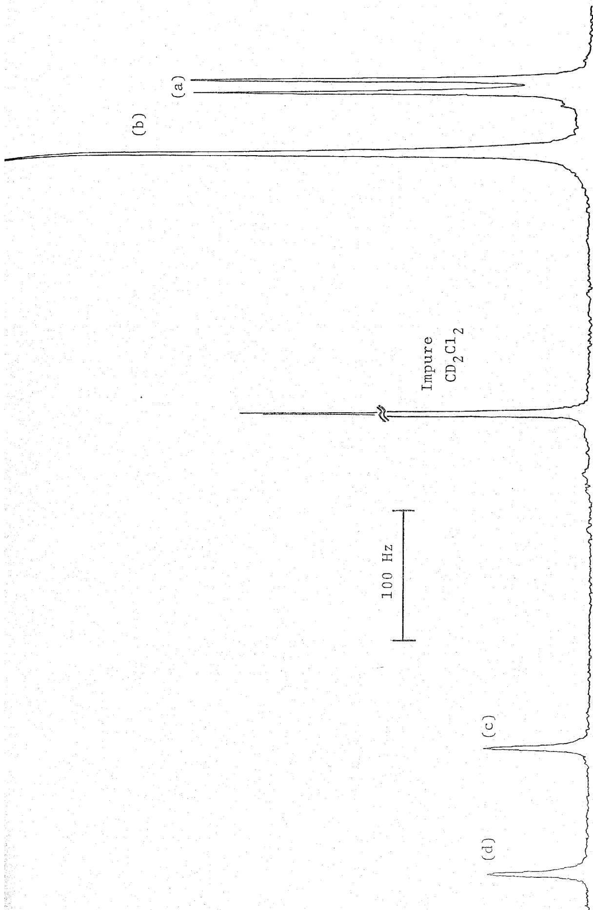
Fig. 13. The ^1\text{H} NMR spectrum of a solution consisting of \text{UO}_2(\text{DMF})_5^{2+} (0.00611 M), DMF (0.0304 M), and \text{CD}_2\text{Cl}_2 (16.1 M) at -80^\circ\text{C} .
