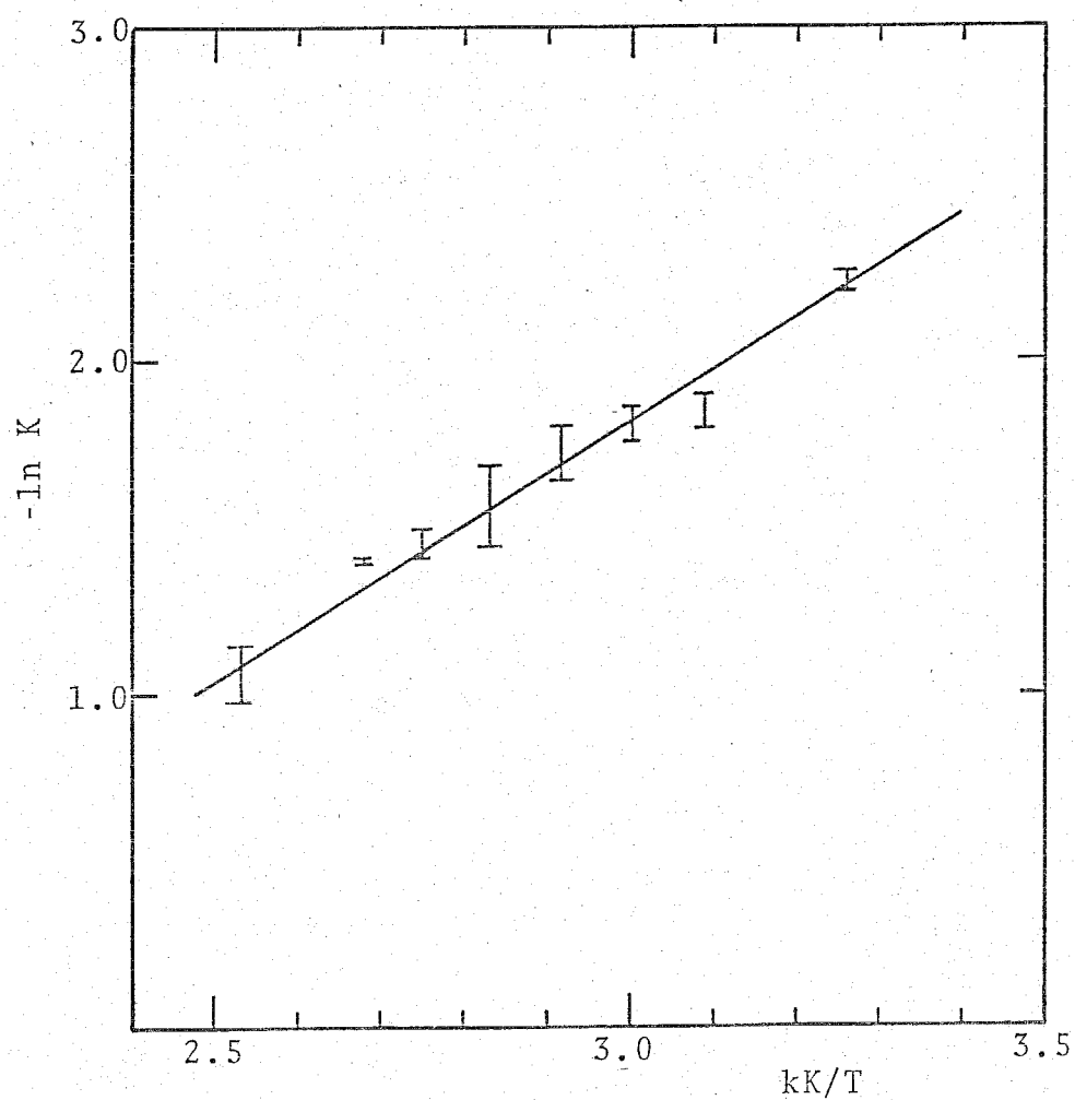
Fig. 2. A plot of -\ln K against the reciprocal temperature for the keto-enol equilibrium of acetylacetone in o\text{-C}_6\text{H}_4\text{Cl}_2 .
