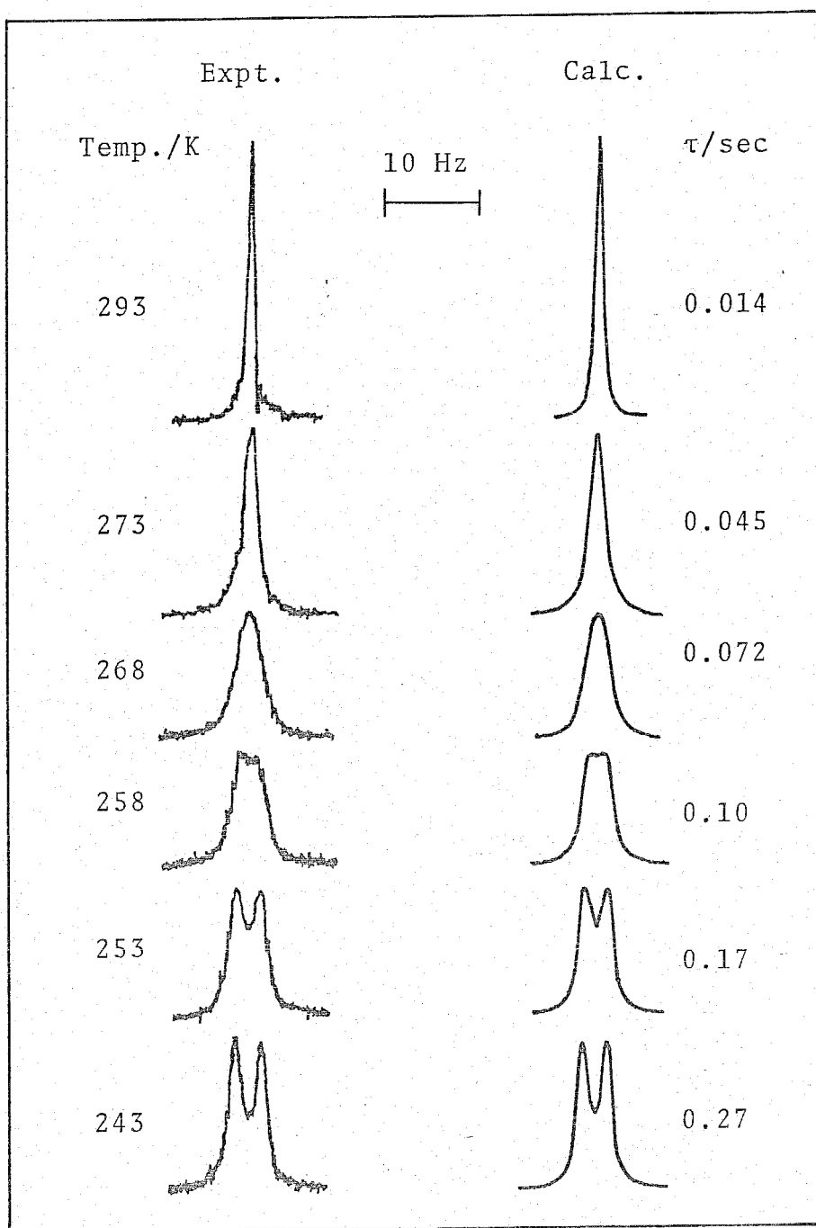
Fig. 13. Experimental(left-hand side) and best-fit calculated ^1\text{H} NMR lineshapes of \text{UO}_2(\text{acac})_2\cdot\text{DEF} (0.0472 m) in \text{CD}_2\text{Cl}_2 . Temperatures and best-fit \tau -values are shown at the left- and right-hand sides of the figure, respectively.
