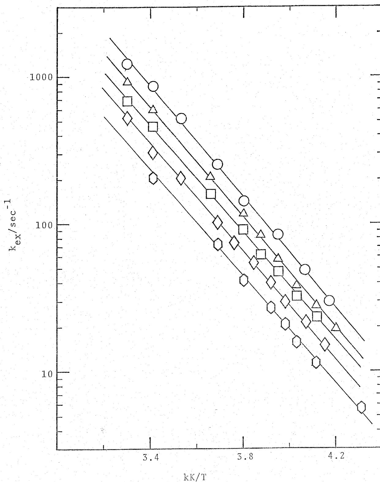
Fig. 15. Semilogarithmic plots of k_{\text{ex}} against the reciprocal temperature for the exchange of DMSO in \text{UO}_2(\text{dbm})_2\text{DMSO} in \text{CD}_2\text{Cl}_2 . The symbols of \diamond , \square , \triangle , and \circ correspond to (i), (ii), (iii), (iv), and (v) in Table 7.
