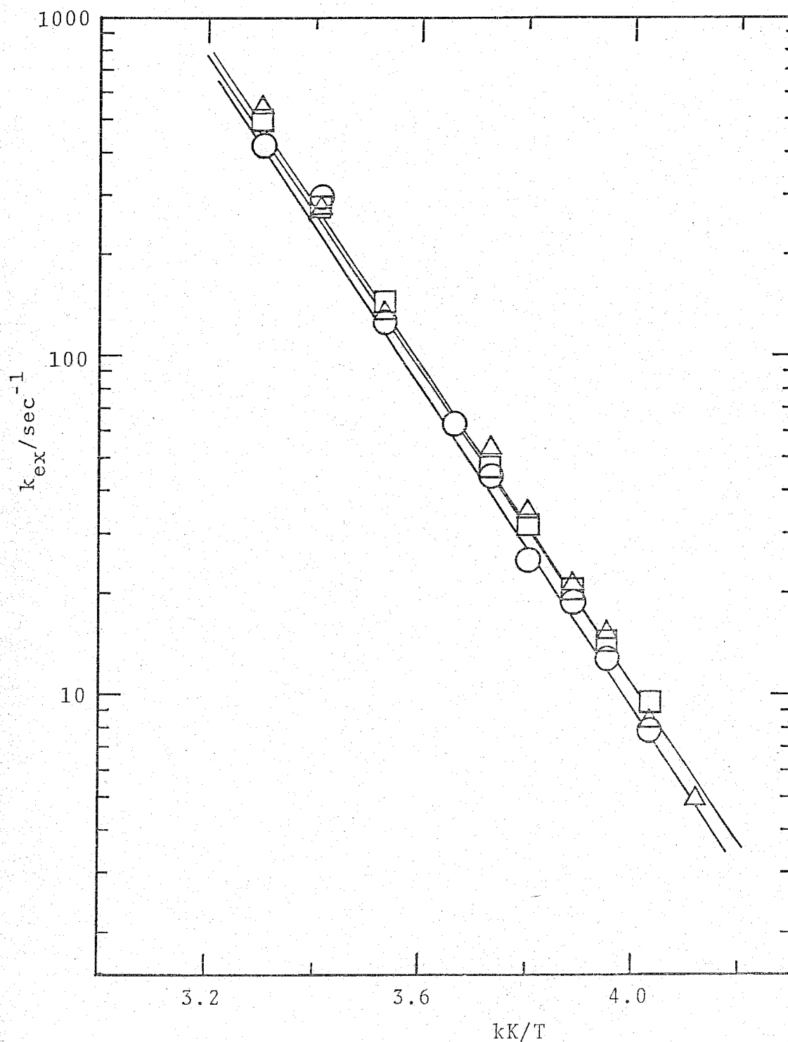
Fig. 13. Semilogarithmic plots of k_{\text{ex}} against the reciprocal temperature for the exchange of DMSO in \text{UO}_2(\text{dbm})_2 DMSO in \text{CD}_3\text{COCD}_3 . The symbols of \bigcirc , \Delta , and \square correspond to (i), (ii), and (iii) in Table 6.
