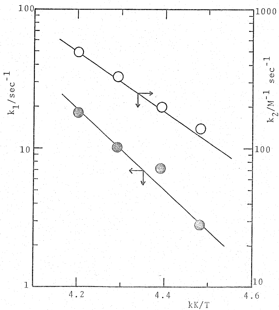
Fig. 12. Semilogarithmic plots of k_1 and k_2 against the reciprocal temperature for the exchange of DMSO in \text{UO}_2(\text{DMSO})_5^{2+} .
