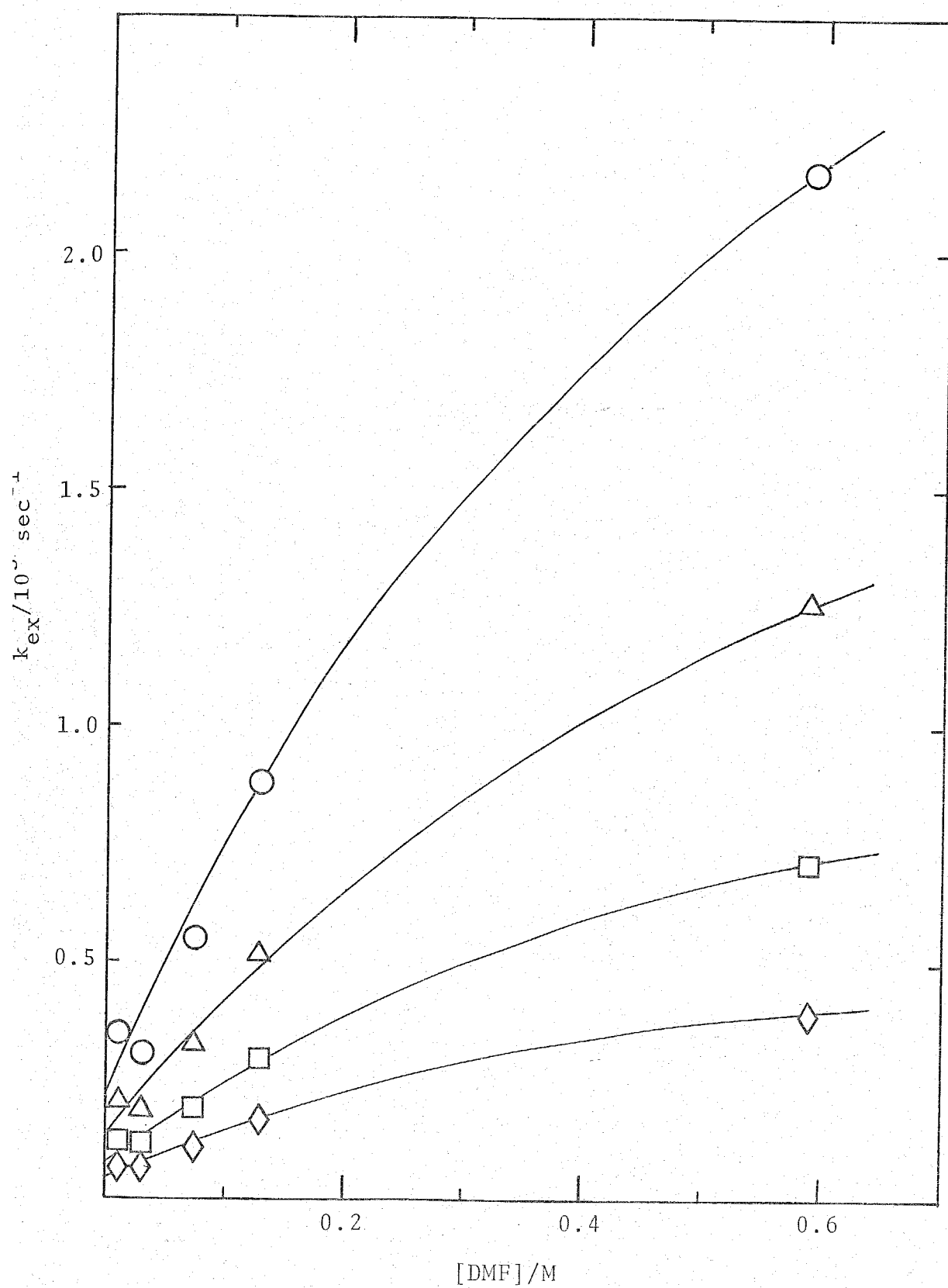
Fig. 16. Plots of k_{\text{ex}} vs. [\text{DMF}] for the exchange of DMF in \text{UO}_2(\text{DMF})_5^{2+} . \bigcirc : -45 °C; \triangle : -50 °C; \square : -55 °C; \diamond : -60 °C. The solid lines are the least-squares fit lines.
