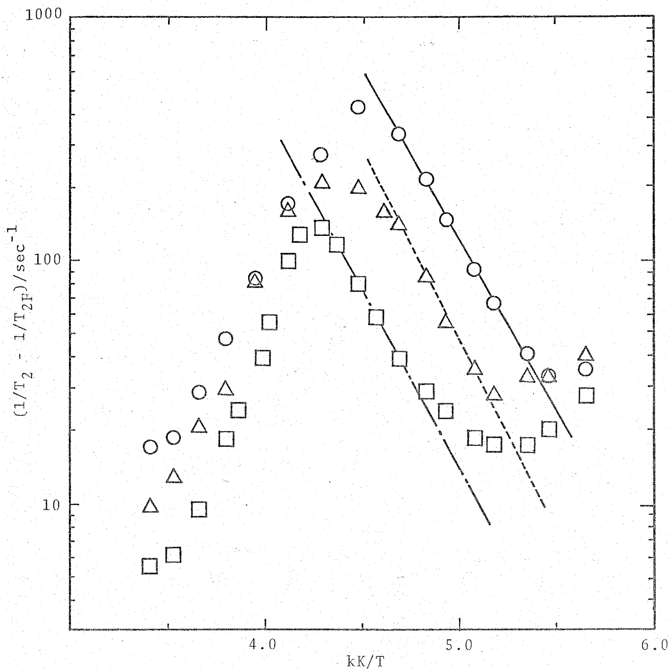
g. 8. A semilogarithmic plot of (1/T_2 - 1/T_{2F}) against the reciprocal temperature for the exchange of water in uranyl mono DMSO, mono chloro, and mono bromo complexes: \bigcirc , [\text{UO}_2^{2+}] = 0.150 \text{ M} , [\text{UO}_2^{2+}] : [\text{DMSO}] : [\text{H}^+] : [\text{H}_2\text{O}] : [\text{CH}_3\text{COCH}_3] = 1 : 1.0 : 12.0 : 84.6 ; \square , [\text{UO}_2^{2+}] = 0.145 \text{ M} , [\text{UO}_2^{2+}] : [\text{HCl}] : [\text{H}_2\text{O}] : [\text{CH}_3\text{COCH}_3] = 1 : 1.0 : 27.9 : 90.4 ; \triangle , [\text{UO}_2^{2+}] = 0.145 \text{ M} , [\text{UO}_2^{2+}] : [\text{HBr}] :
