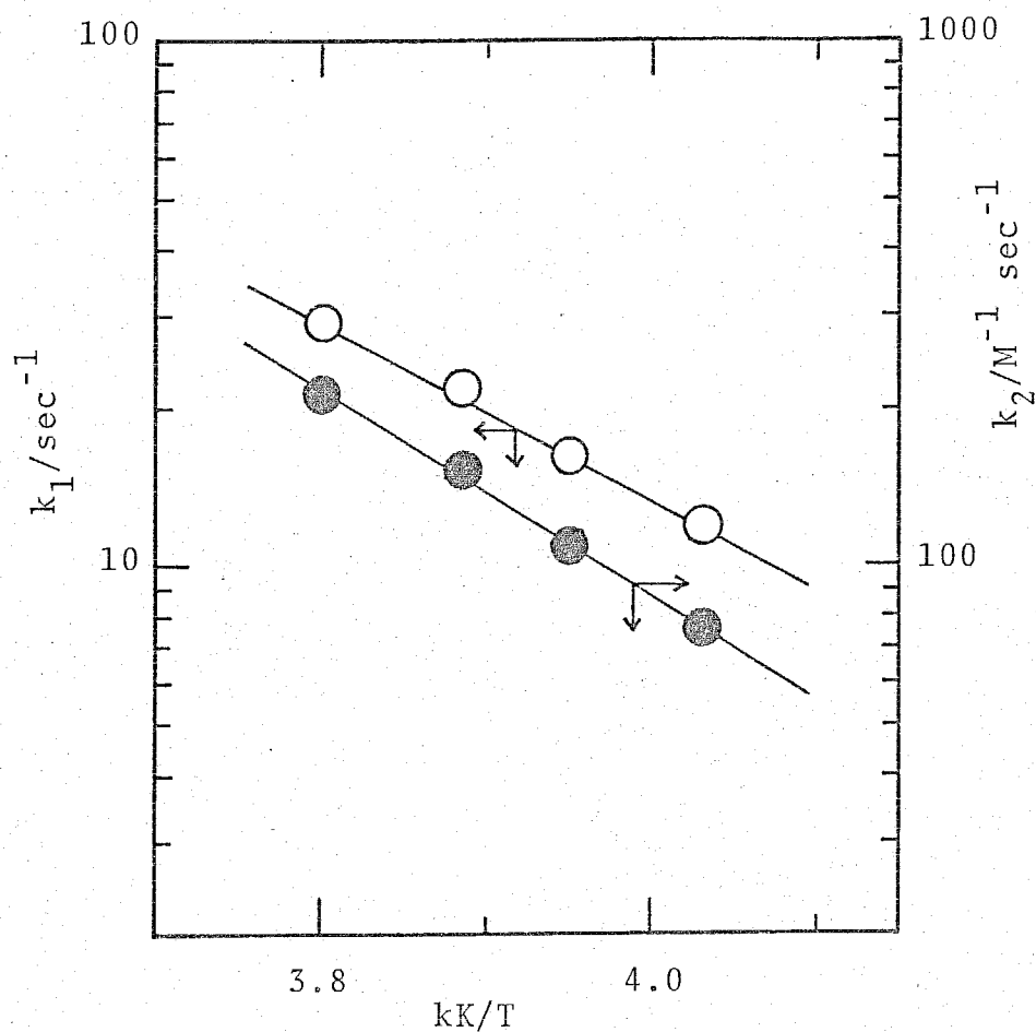
Fig. 17. Semilogarithmic plots of k_1 and k_2 against the reciprocal temperature for the exchange of DMSO in \text{UO}_2(\text{dbm})_2 DMSO in \text{CD}_2\text{Cl}_2 .
