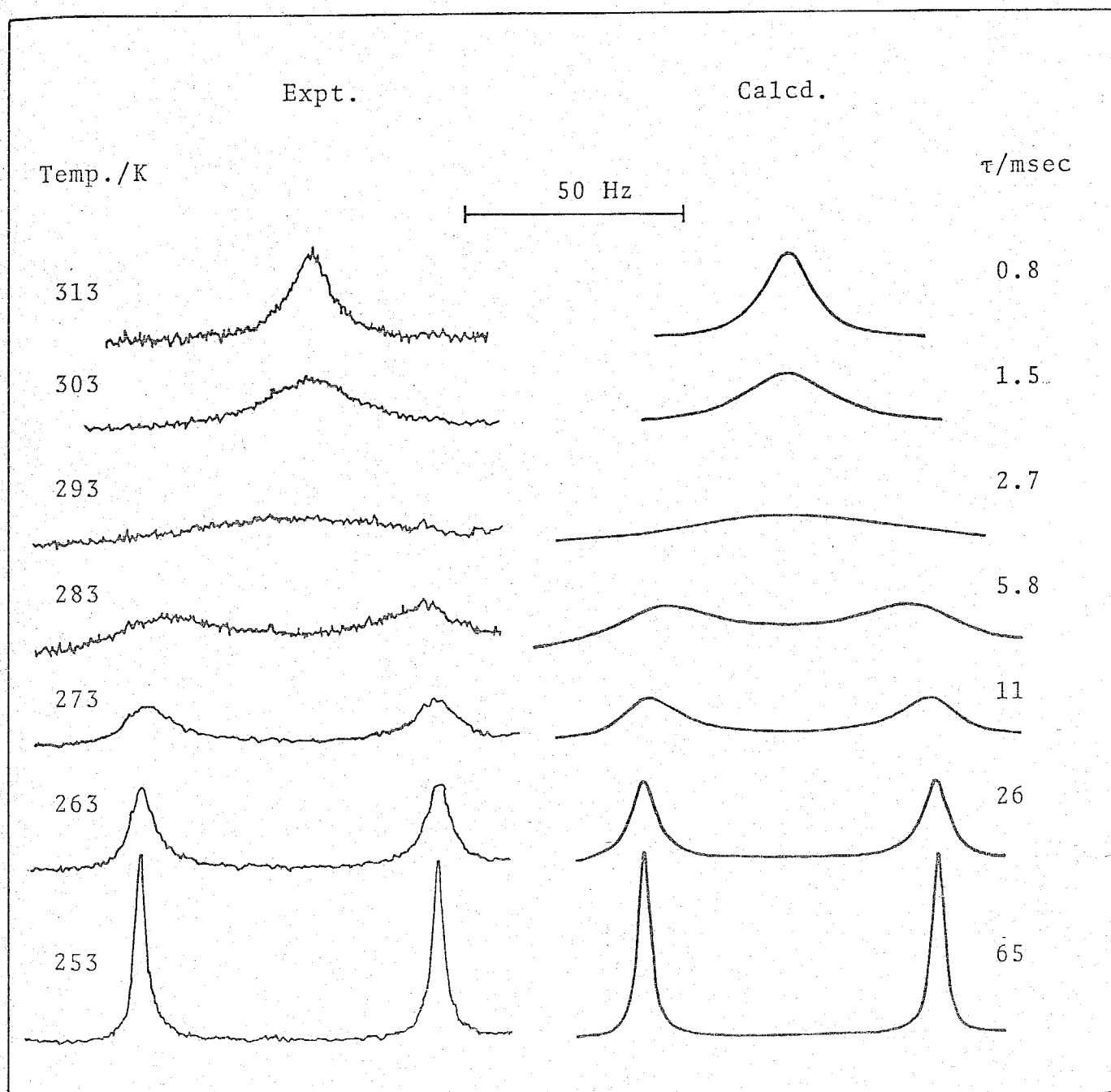
8. 4. Experimental(left-hand side) and best-fit calculated ^1\text{H} NMR lineshapes of a solution consisting of \text{UO}_2(\text{acac})_2 DMSO(0.0298 M), DMSO(0.0294 M), and \text{CD}_3\text{COCD}_3 (13.6 M). Temperatures and best-
