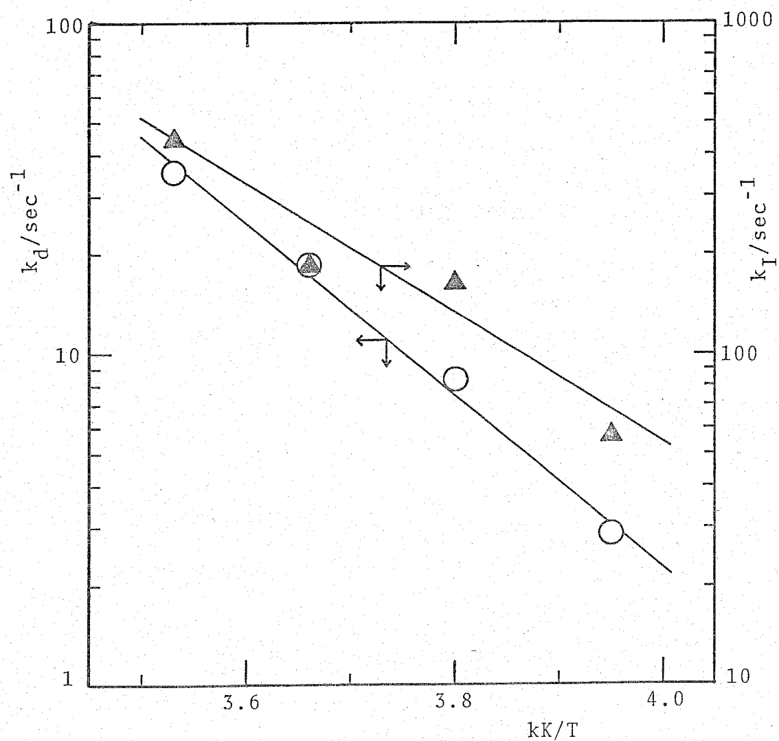
Fig. 9. Semilogarithmic plots of k_d and k_I against the reciprocal temperature for the exchange of DMSO in \text{UO}_2(\text{dbm})_2 DMSO in \text{CD}_2\text{Cl}_2 .
