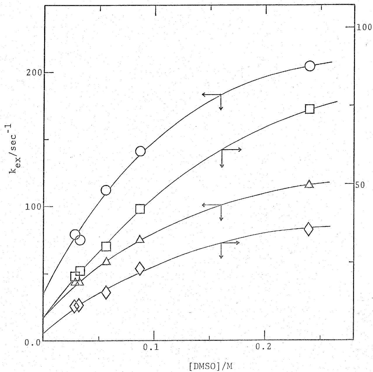
Fig. 8. Plots of k_{\text{ex}} vs. [\text{DMSO}] for the exchange of DMSO in \text{UO}_2(\text{acac})_2\text{DMSO} in \text{CD}_2\text{Cl}_2 . \bigcirc : 10 °C; \triangle : 0 °C; \square : -10 °C; \diamond : -20 °C.
