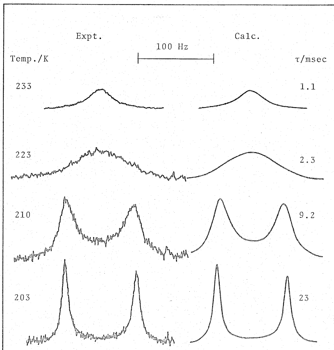
Fig. 14. Experimental(left-hand side) and best-fit calculated ^1\text{H} NMR lineshapes of a solution consisting of \text{UO}_2(\text{DMF})_5^{2+} (0.00611 M), DMF(0.0304 M), and \text{CD}_2\text{Cl}_2 (16.1 M). Temperatures and best-fit \tau -values are shown at left- and right-hand sides of the figure, respectively.
