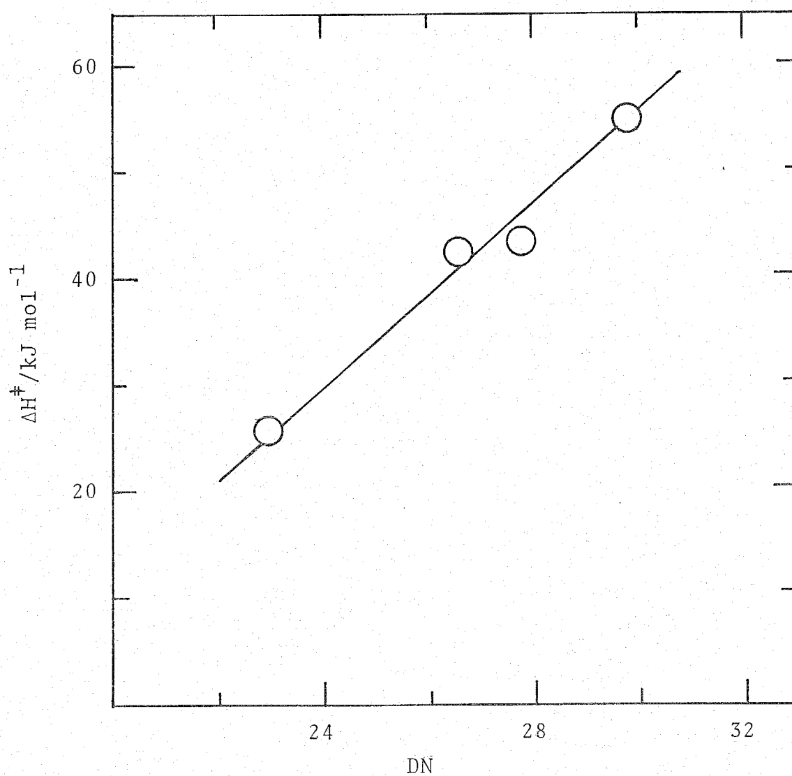
Fig. 18. A plot of \Delta H^\ddagger vs. DN for the ligand exchange in various uranyl complexes.
