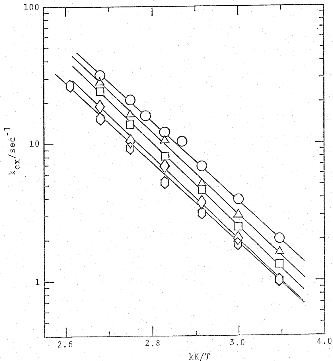
Fig. 7. Semilogarithmic plots of k_{\text{ex}} against the reciprocal temperature for the exchange of acac in \text{UO}_2(\text{acac})_2\text{DMSO} in o\text{-C}_6\text{H}_4\text{Cl}_2 containing the free DMSO. The symbols of \circ , \triangle , \square , \diamond , and \hexagon correspond to (i), (ii), (iii), (iv) and (v) in Table 4, respectively.
