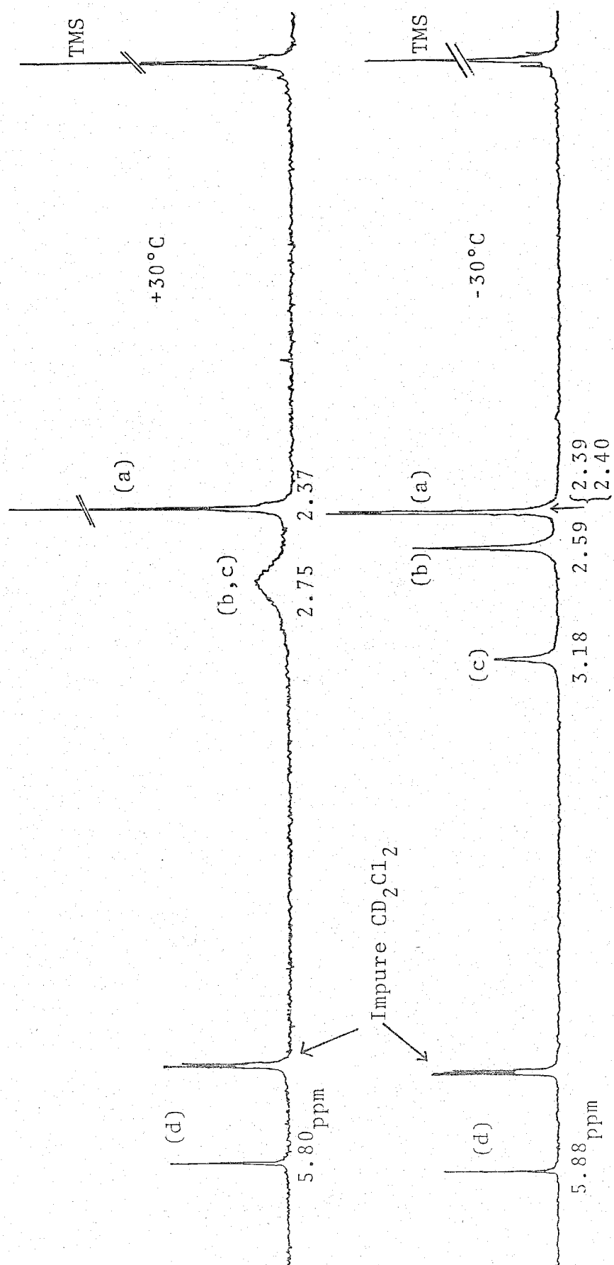
Fig. 3. The ^1\text{H} NMR spectra of a solution consisting of \text{UO}_2(\text{acac})_2 in \text{DMSO} (0.0179 M), \text{DMSO} (0.0282 M), and \text{CD}_2\text{Cl}_2 (15.8 M) at -30 and +30^\circ\text{C} , respectively.
