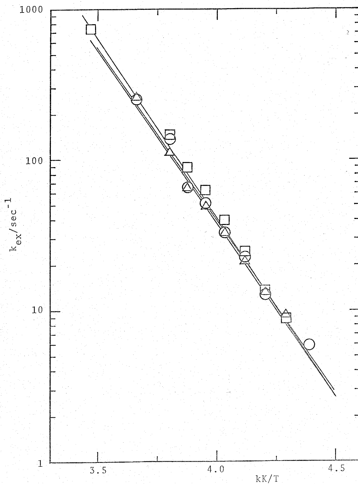
Fig. 21. Semilogarithmic plots of k_{\text{ex}} against the reciprocal temperature for the exchange of DMF in \text{UO}_2(\text{acac})_2\text{DMF} in \text{CD}_3\text{COCD}_3 . The symbols of ○, △, and □ correspond to (i), (ii), and (iii) in Table 11.
