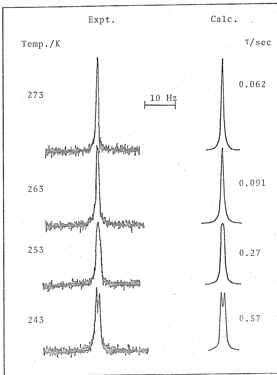
Fig. 7. Experimental(left-hand side) and best-fit calculated ^1\text{H} NMR lineshapes of \text{UO}_2(\text{acac})_2\text{DMSO}(0.0311 \text{ m}) in \text{CD}_2\text{Cl}_2 . Temperatures and best-fit \tau -values are shown at the left- and right-hand sides of the
