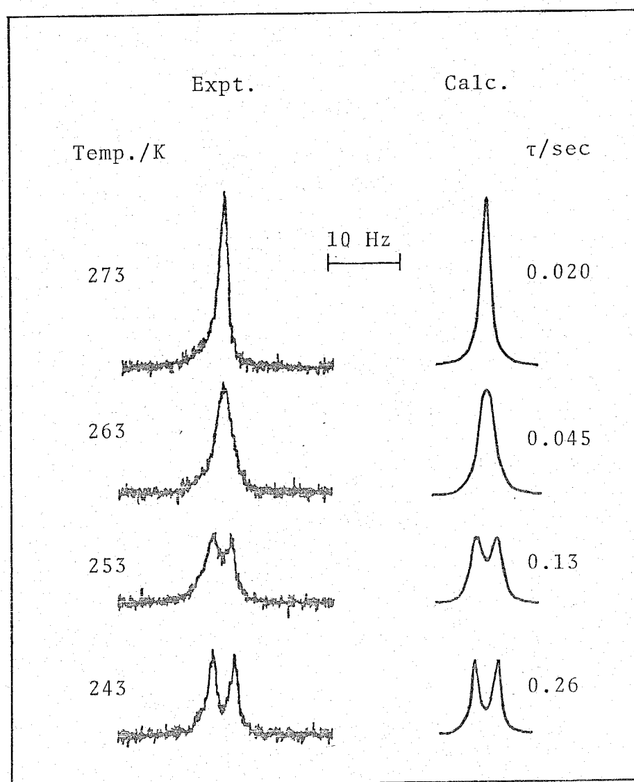
Fig. 8. Experimental (left-hand side) and best-fit calculated ^1\text{H} NMR lineshapes of \text{UO}_2(\text{acac})_2 \cdot \text{DMSO} (0.0574 m) in \text{CD}_3\text{COCD}_3 . Temperatures and best-fit \tau -values are shown at the left- and right-hand sides of the figure, respectively.
