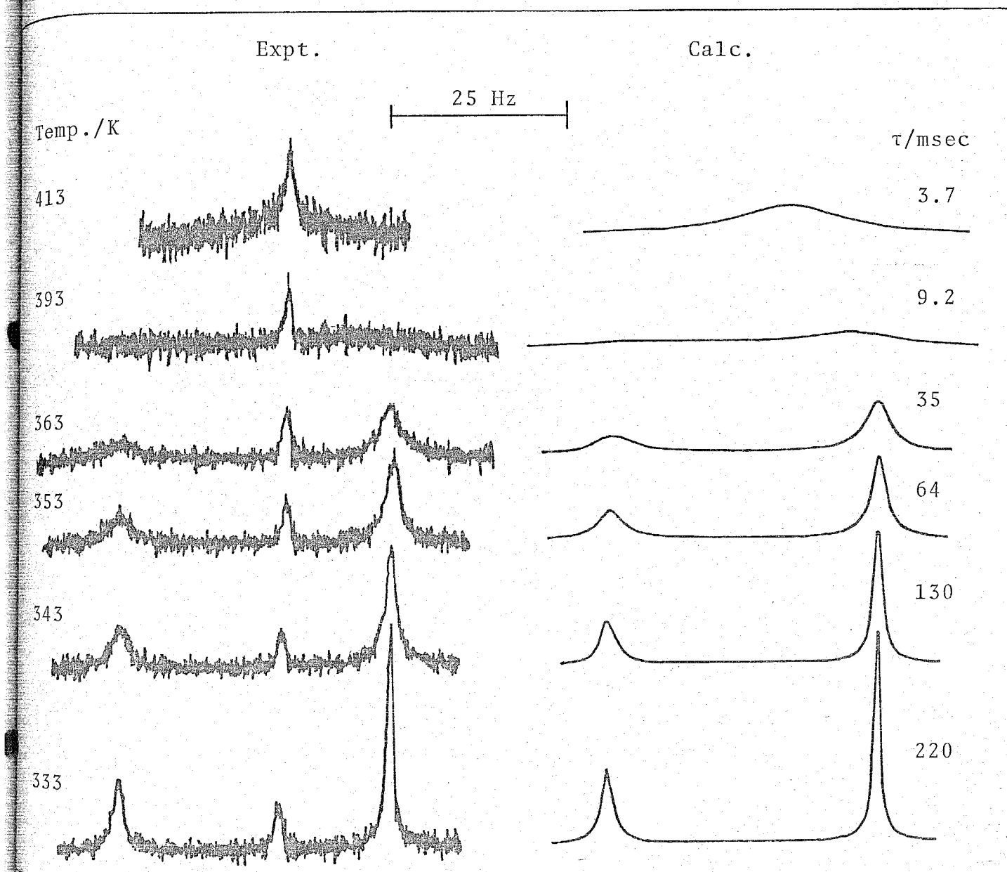
Fig. 3. Experimental(left-hand side) and best-fit calculated ^1\text{H} NMR lineshapes of a solution consisting of \text{UO}_2(\text{acac})_2 DMSO(0.0600 M) Hacac(0.256 M) and \text{o-C}_6\text{H}_4\text{Cl}_2 (8.71 M). Temperatures and best-fit \tau -values are shown at left- and right-hand sides of the figure, respectively.
