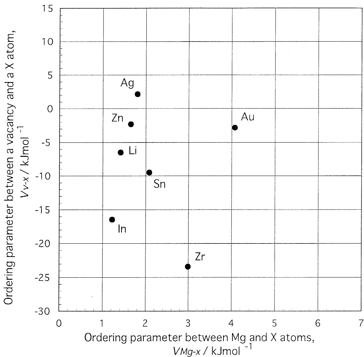
Fig.7.13 Relationships between V_{v-x} and V_{Mg-x} for various elemental atoms, x ( V_{v-x} : ordering parameter between a vacancy and a x atom, V_{Mg-x} : ordering parameter between Mg and x atoms).
