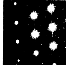
Fig. 7.5 Continued; (e) Si-added, (f) Mg-added and (g) (Mg+Ag)-added alloys aged at 463K for 86.4ks.
