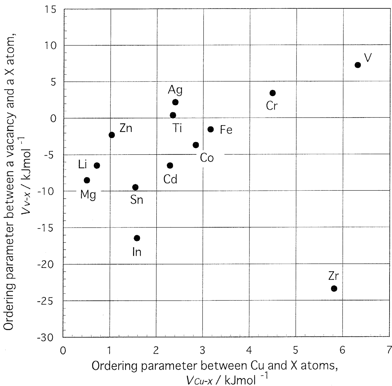
Fig.4.8 Relationships between V_{V-X} and V_{Cu-X} for various elemental atoms, X ( V_{V-X} : ordering parameter between a vacancy and a X atom, V_{Cu-X} : ordering parameter between Cu and X atoms).
