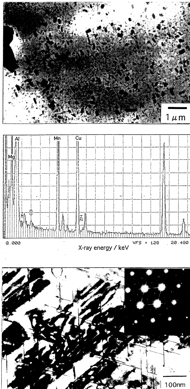
Fig.8.8 Electron micrographs(a)(c) for 2.3Cu-0.6Mg-Zn-Mn alloy aged at 433K for 346ks and EDS analysis profile(b) of the block-shaped or rod-shaped precipitates in micrograph(a).
