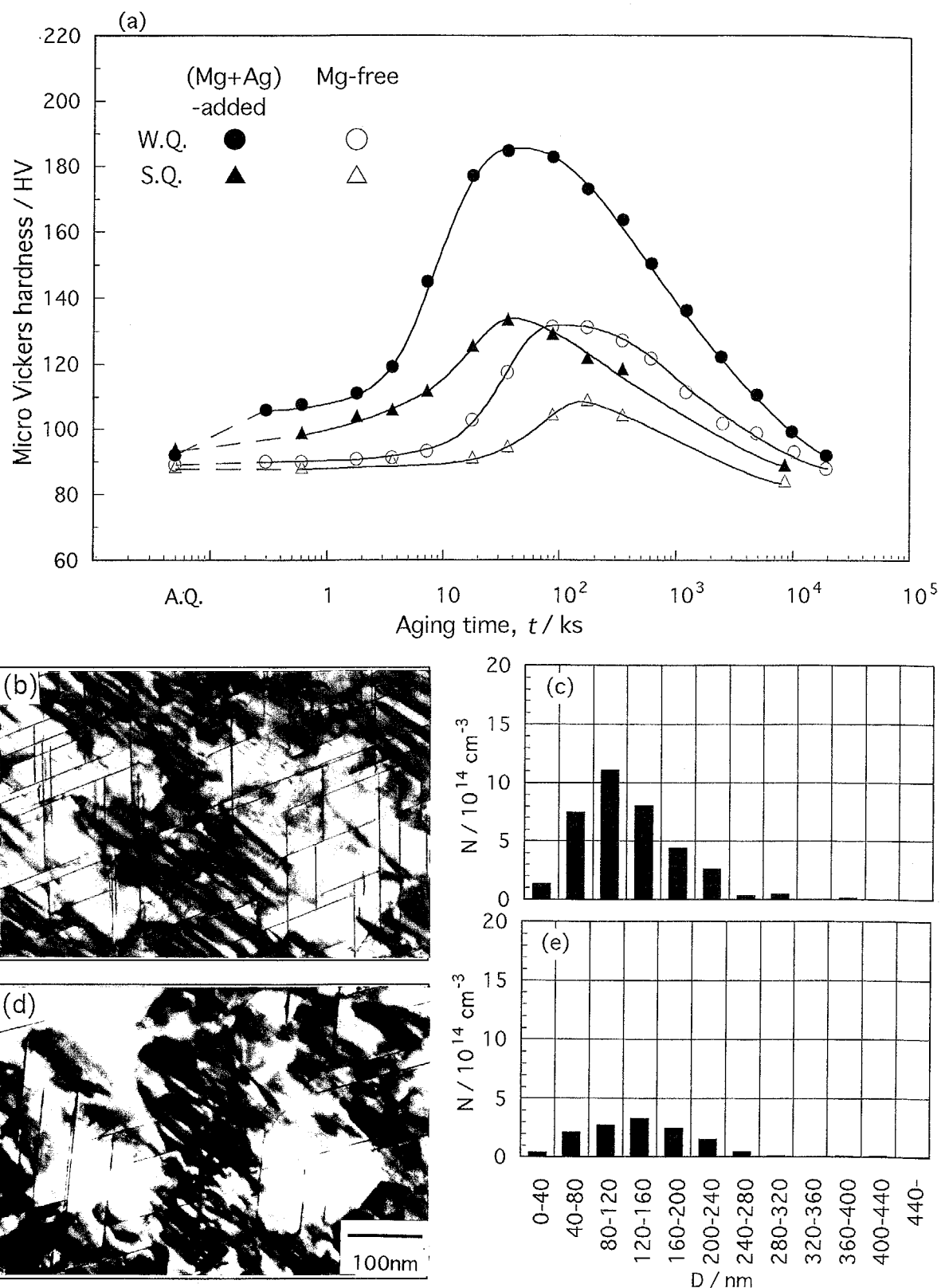
Fig.7.8 Variations of hardness with aging time for 463K aging (a) and electron micrographs and precipitate size distributions for (Mg+Ag)-added alloys aged at 463K for 36ks after W.Q. treatment from 778K (b,c) and S.Q. treatment from 673K (d,e).
