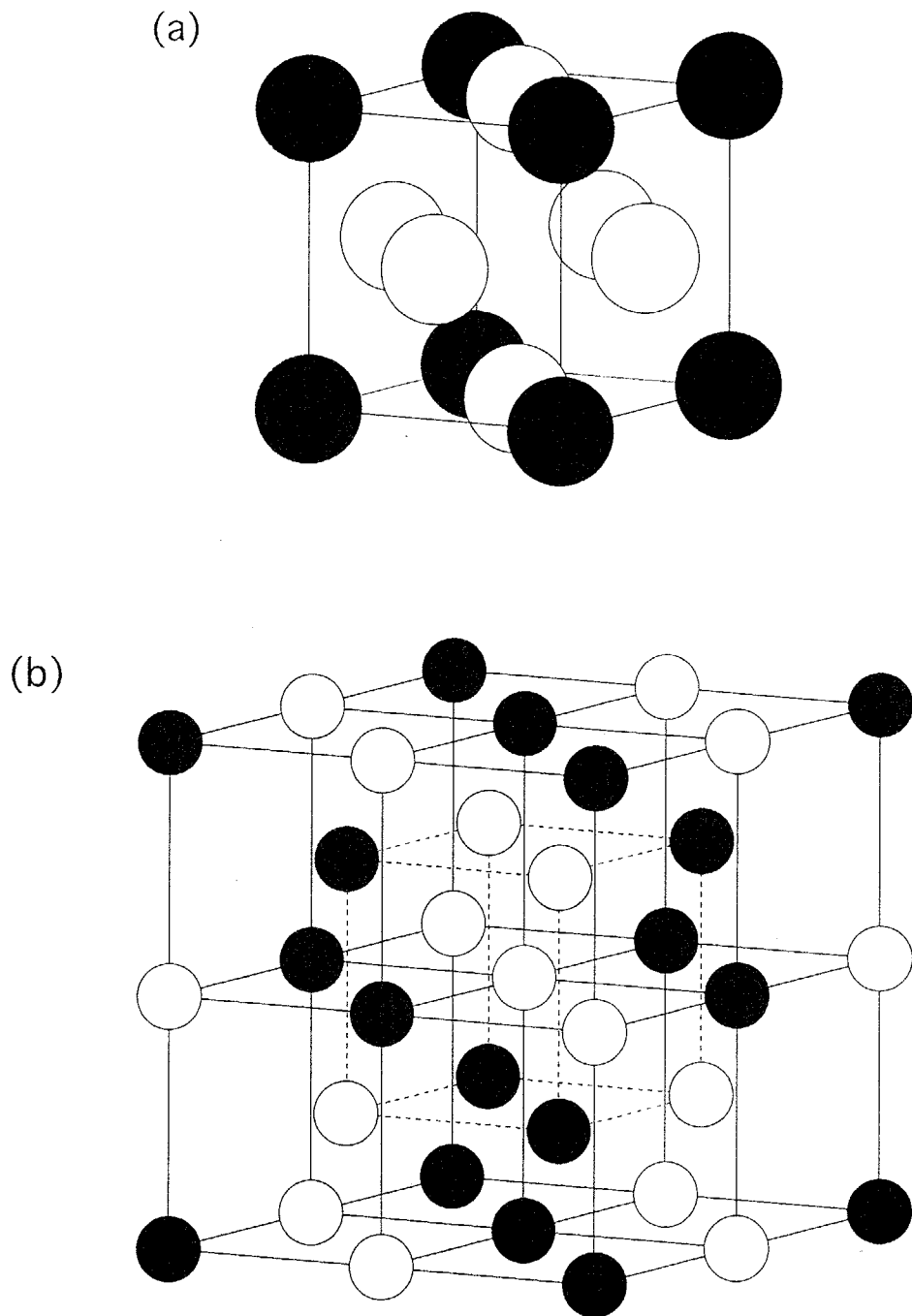
Fig.1.2 Unit cells of crystal structures of two precipitates in Al-Li alloys; (a) metastable \delta' ( \text{Al}_3\text{Li} ) phase having a \text{L1}_2 -structure and (b) stable \delta ( \text{AlLi} ) phase having a \text{B32} -structure. The open and solid circles represent Al and Li atoms, respectively.
