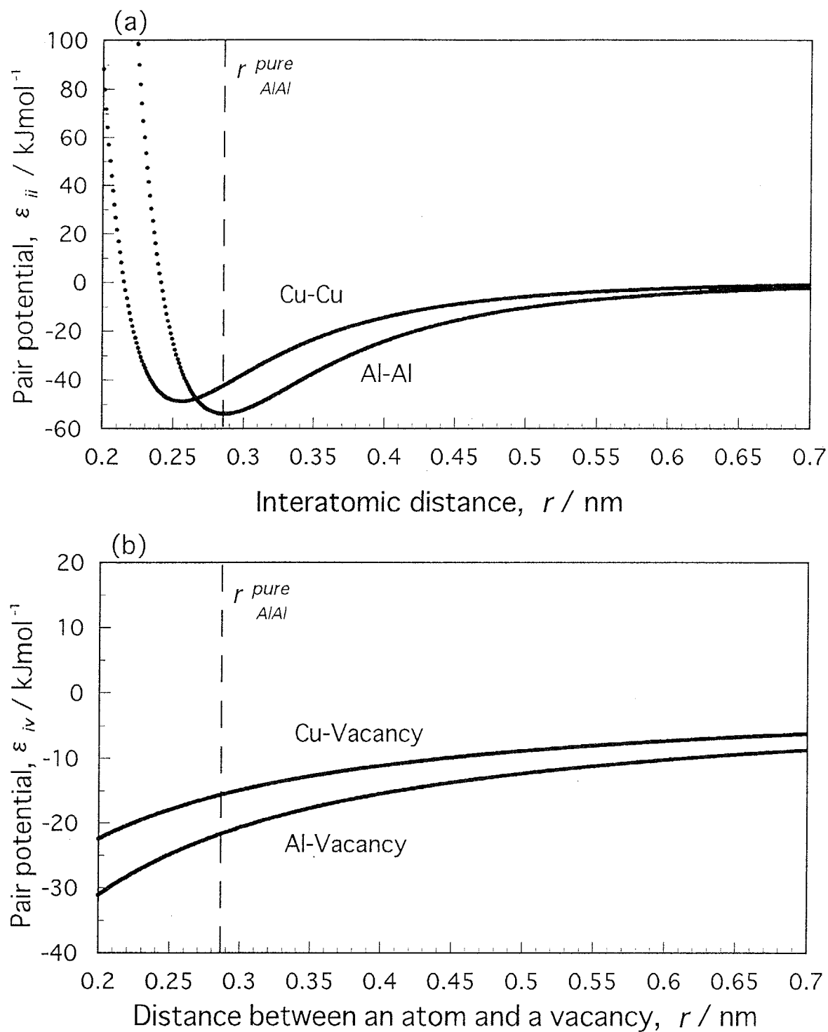
Fig.3.5 Variations in assumed pair interactions between same atom species, \epsilon_{ii} (a) and between an atom and a vacancy, \epsilon_{iv} (b) as a function of the distance between them. The vertical broken lines represent an interatomic distance of an arbitrary pair located on Al lattice sites.
