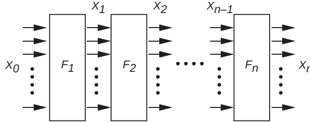
Fig. 3.1. The layered network as a cascade of vector-to-vector functions F_1, F_2, \dots, F_n . Matrices X_0, X_1, \dots, X_n denote the layer response trace for all the training sets, in the style of the notations defined above.
