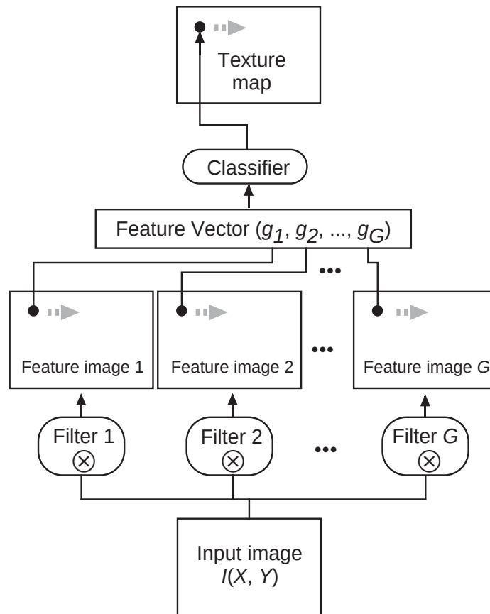
Fig. 5.1. The procedure of texture classification by multichannel filtering. The operator “ \otimes ” denotes the two-dimensional convolution of the filter kernel and the image. The maps obtained by various convolution filters will be used as the feature vectors for use at the classifier to obtain the texture map.
