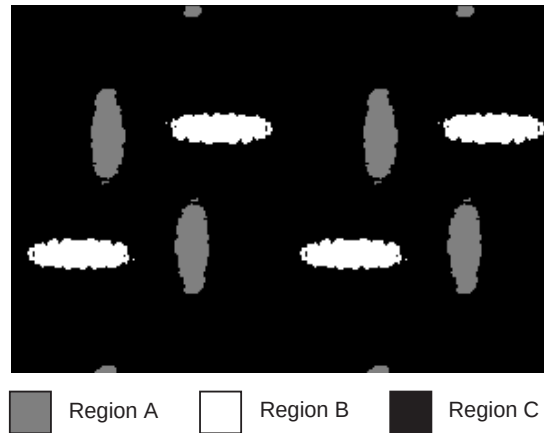
Fig. 5.7. The classification map of the image in Fig. 5.6, produced by the trained KM Net. The texture regions A and B are correctly extracted as instructed by the training sets.
