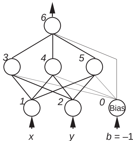
Fig. 3.3. A small three-layered network.
