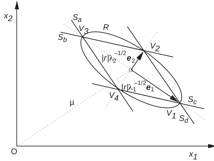
Fig. 4.9. Model switching by replacement of an O_2 unit R by 2^L O_1 units ( S_a, S_b, S_c, S_d ), for L = 2 , preserving the characterized region. Vectors \mathbf{e}_1 and \mathbf{e}_2 are unit vectors in the first and second principal components of the ellipse. The index for the hidden neuron n is omitted.
