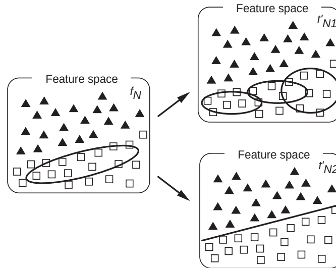
Fig. 2.7. Two switching alternatives in a network that can use locally tuned RBF type units and linear type units.
