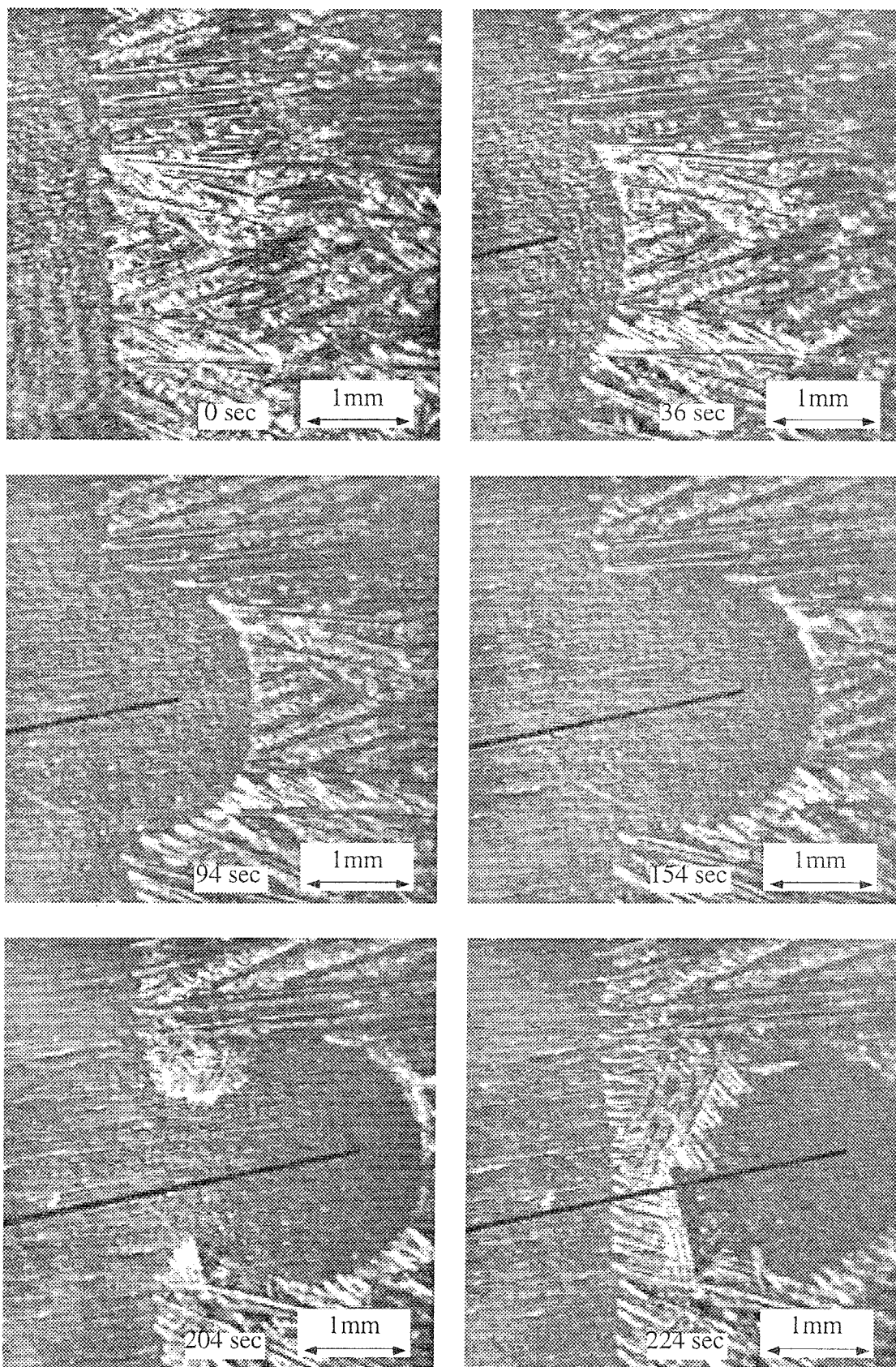
图 5-3-11 The Responce of Dendritic Ice to Injection of High Concentration Solution.
