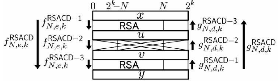
Figure 2.1: Functions f_{N,e,k}^{\text{RSACD}} and g_{N,d,k}^{\text{RSACD}}
