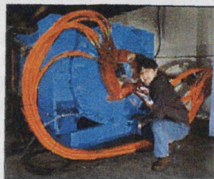
Photo of the new warm helical snake magnet is shown taken at the Tokyo Institute of Technology, who designed the magnet with Masamichi Okumura of RIKEN. Built by the Tokai Engineering Magnet Company in Japan, the new snake was handed by RIKEN.
