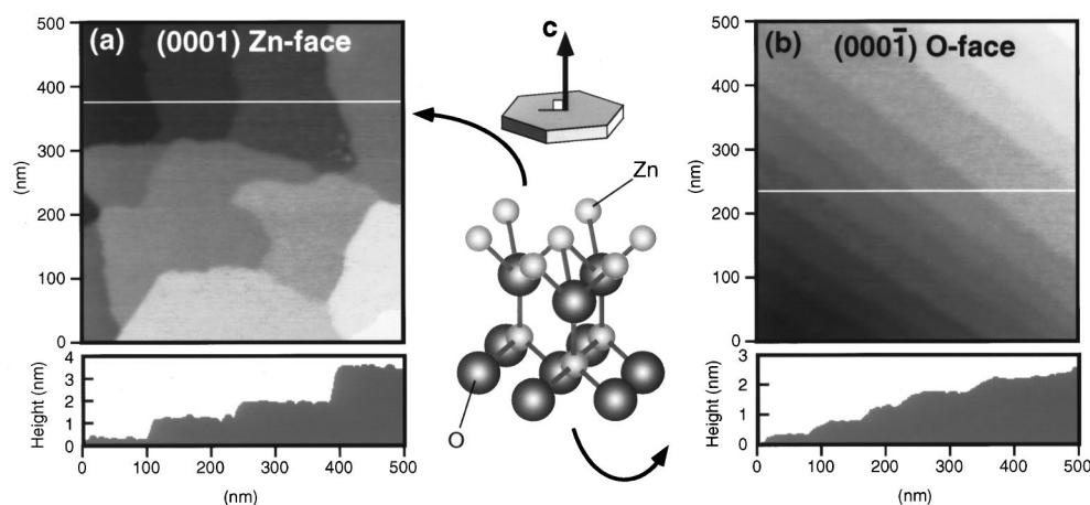
FIG. 1. AFM images (500 nm \times 500 nm) of ZnO single crystals annealed at 1000 ^{\circ} C in air: (a) (0001) surface, and (b) (0001) surface.
