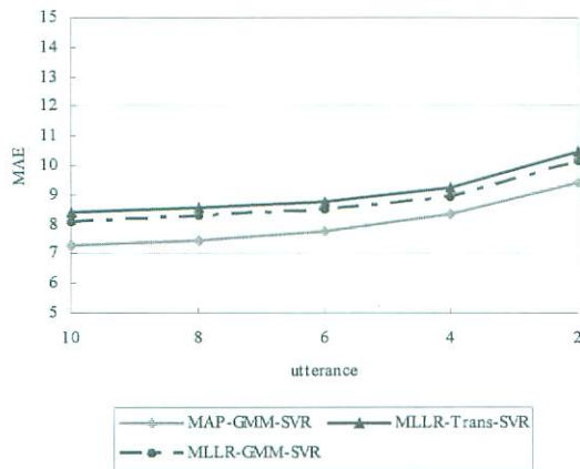
Fig. 5. Number of utterances and MAE using SVR based estimators with different features.
