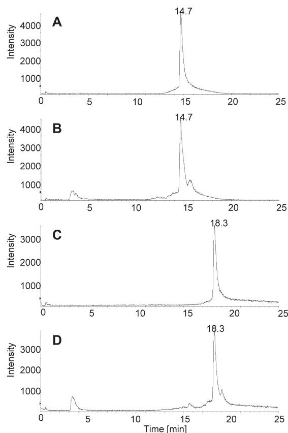
Figure 4. LC/TOF-MS/MS sum ion chromatograms of authentic glycyrrhizin and the extract of cultured stolons as the precursor ion of the parent ion in negative ion scan mode. HPLC chart of (A) authentic glycyrrhizin in System 1 HPLC condition, (B) the extract of the cultured stolon in System 1, (C) authentic glycyrrhizin in System 2, and (D) cultured stolon in System 2. Conditions of Systems 1 and 2 are described in Materials and Methods under "Triterpenoid and sterol analysis of stolons".
