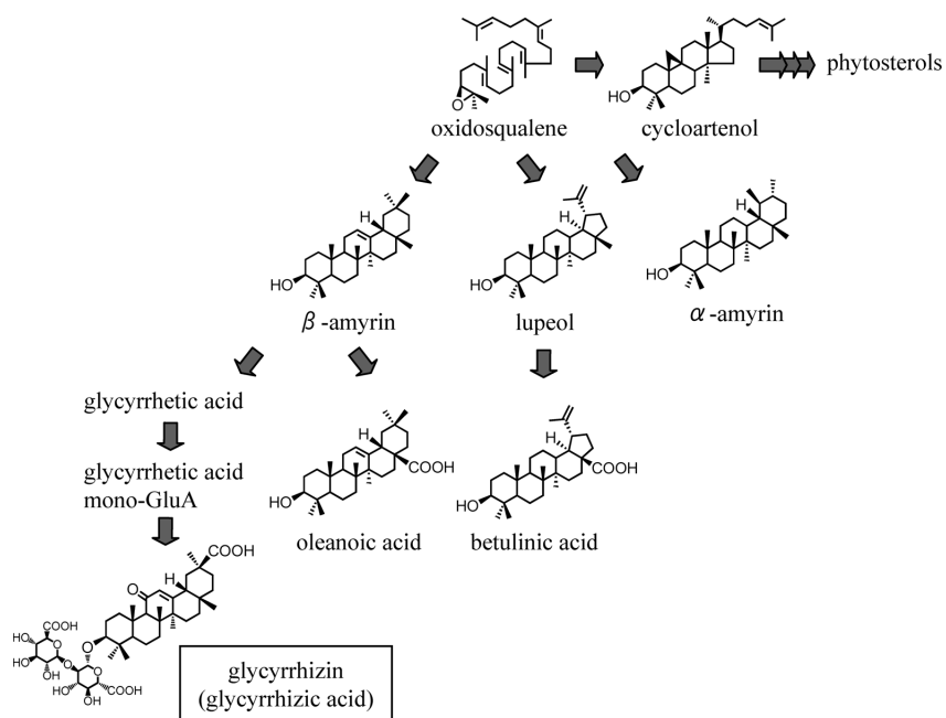
Figure 1. Chemical structures and the deduced biosynthetic pathway for glycyrrhizin (glycyrrhizic acid) and related triterpenoids in licorice plants.
