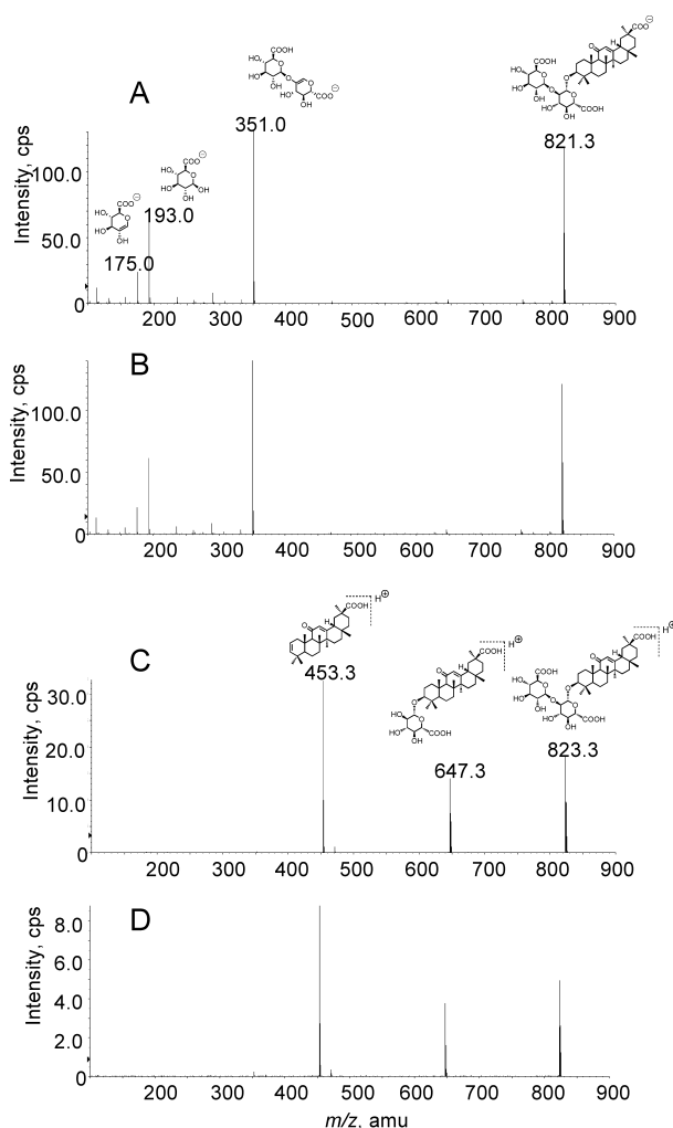
Figure 5. Product ion spectra of precursor ions m/z 821.3, [M-H]^- and 823.3, [M+H]^+ . (A) authentic glycyrrhizin in negative ion scan mode, (B) main peak of the extract of the cultured stolon in negative ion scan mode, (C) authentic glycyrrhizin in positive ion scan mode, (D) main peak of the extract from cultured stolons in positive ion scan mode.
