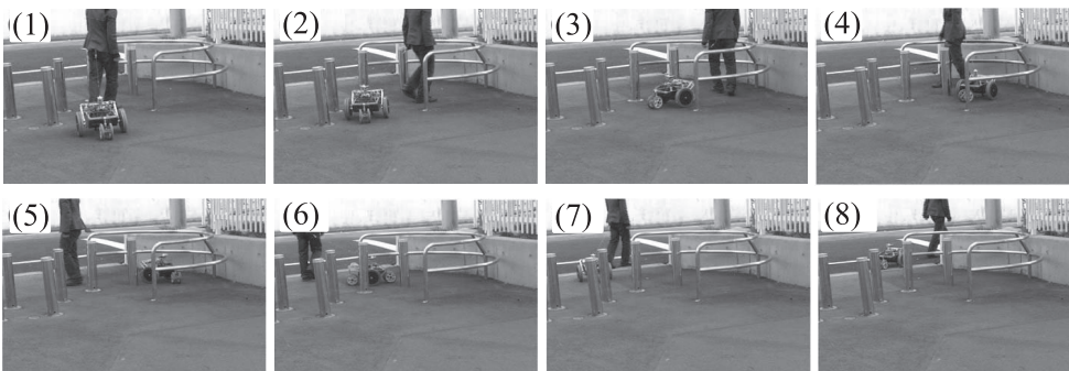
Fig. 21 An experiment passing through bollards in outdoor environment at 2.0 [s] interval capture (left), top view of the path (right)
