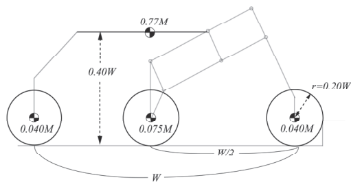
Fig. 7 Simulation model for the dynamics simulator
