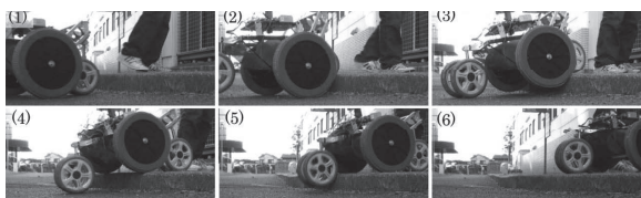
Fig. 19 Step climbing experiment: height of the curb 90 [mm]
