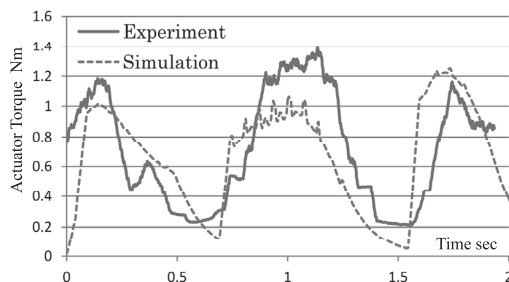
Fig. 20 Driving torque comparison between simulation and experiment negotiating 60 [mm] height step
