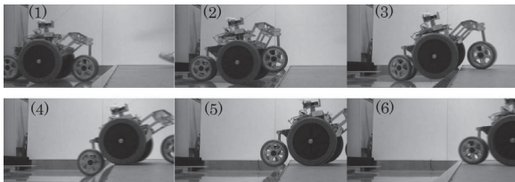
Fig. 18 Step climbing experiment: height of the step 80 [mm]
