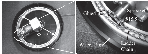
Fig. 12 Developed low-profile in-wheel motor
