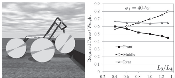
Fig. 8 An example of ODE simulation (left) and required force (right)
