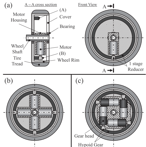
Fig. 11 Proposed low-profile in-wheel motor
