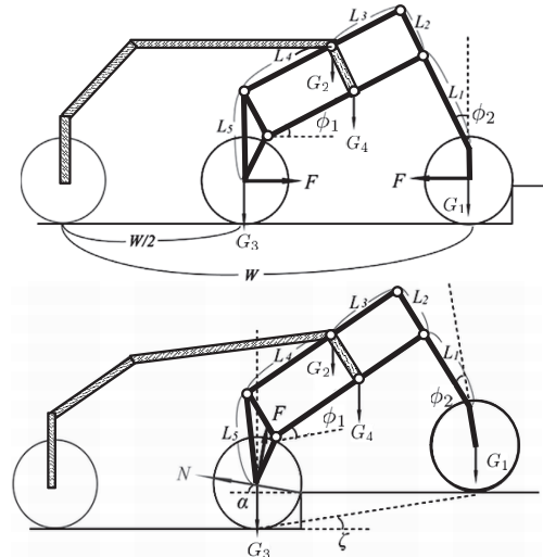
Fig. 5 Static force analysis: front wheel negotiating (top), middle wheel negotiating (bottom)
