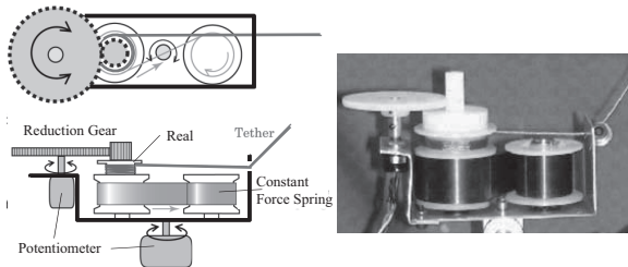
Fig. 13 Tether mechanism to measure the tether length and direction
