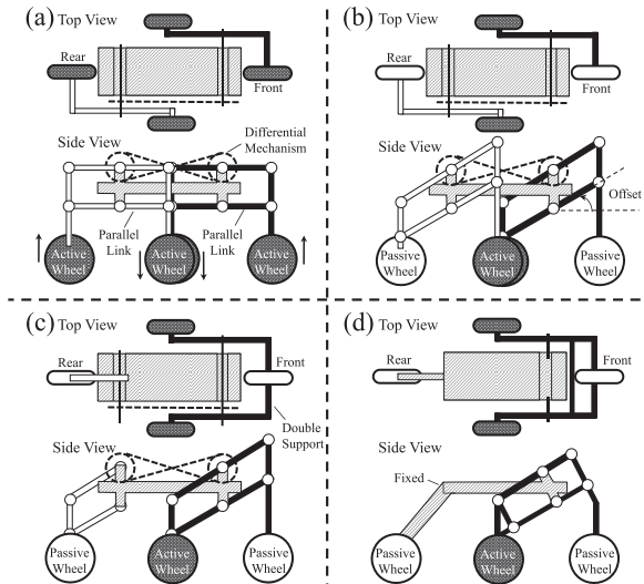
Fig. 4 Modification of the bogie link system: (a) Hien II with four active wheels, (b) introducing initial offset to the bogie links, (c) double support beam structure for the bogie links, (d) fixing the rear wheel steering axis to the body (final design)
