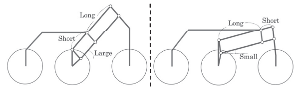
Fig. 6 Results of the static force analysis: suitable for the front wheel negotiation (left), for the middle wheel negotiation (right)
