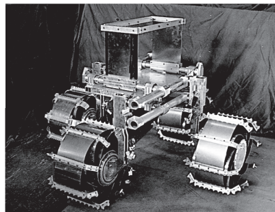
Fig. 3 Prototype model of a mars exploration rover “Hien II”
