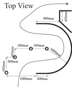
Fig. 21 An experiment passing through bollards in outdoor environment at 2.0 [s] interval capture (left), top view of the path (right)
