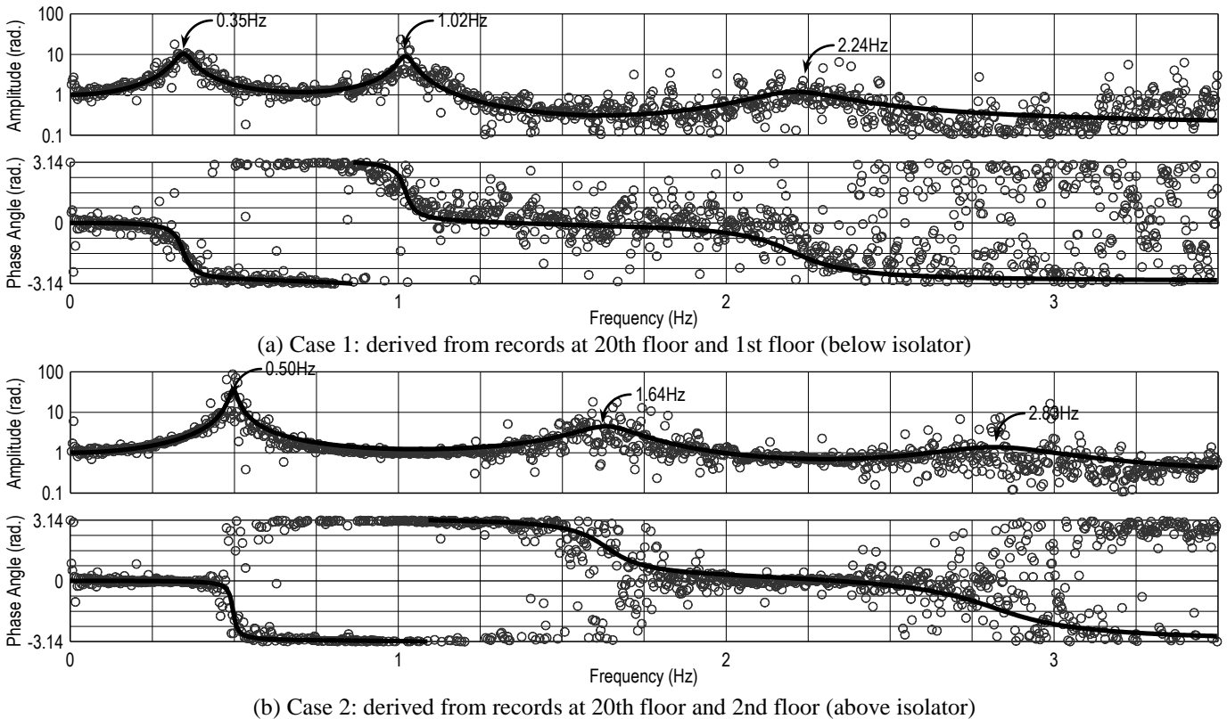
Figure 9. Example of transfer function and curve-fitting in X-direction
