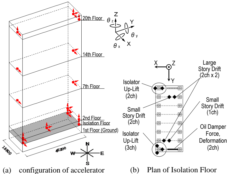
Figure 4 Monitoring System
