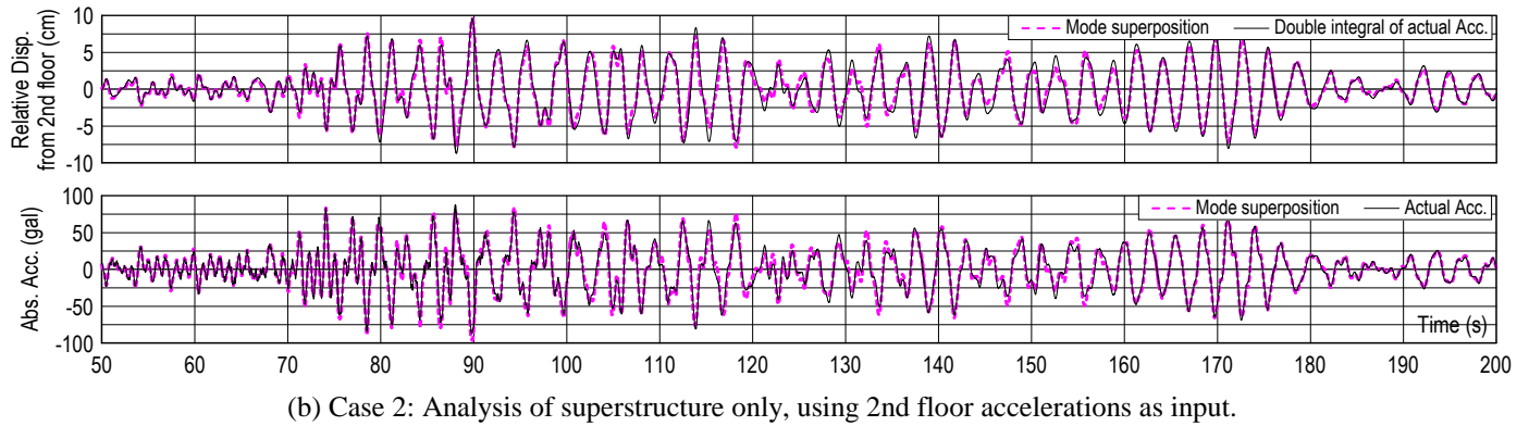
Figure 10. Comparison of top-level behavior between recorded data and modal analysis using identified modal frequencies and damping ratios in X-direction
