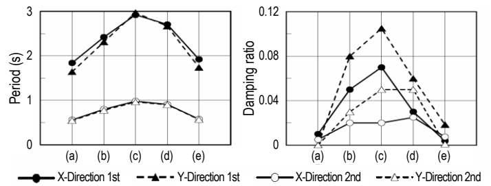
Figure 14. Vibration periods and damping ratios obtained before and after significant earthquake
