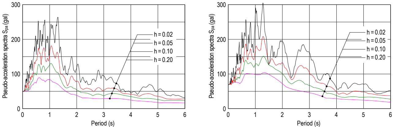
Figure 7. Response spectra for base motions in X and Y directions
