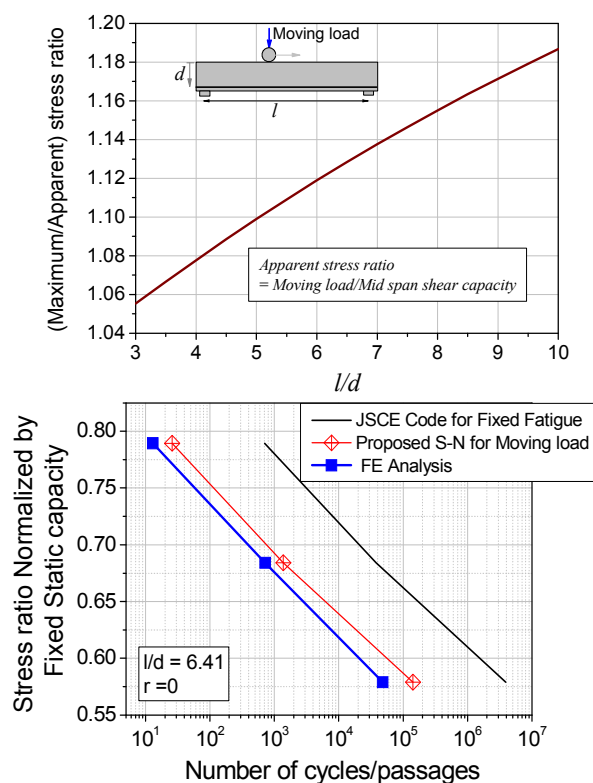
Fig. 10 S-N diagram base on simplified shear fatigue estimation method as compared to FE analysis.
