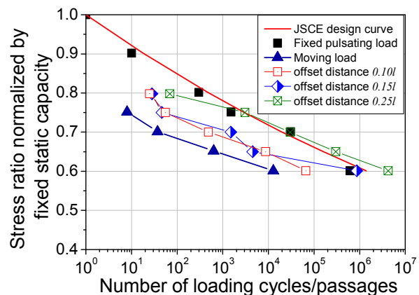
b) S-N relation for different offset distance
