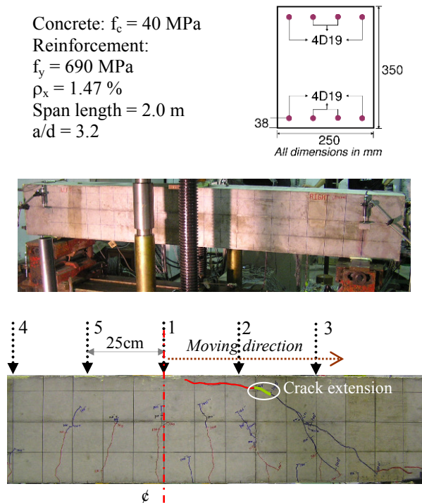
Fig. 2 Material and geometric details, loading set-up and crack pattern.
