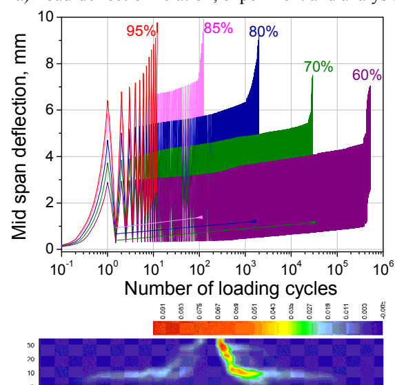
b) fixed pulsating load
