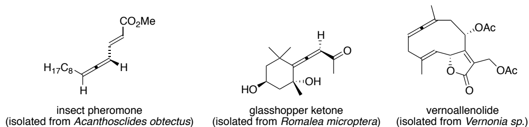
Figure 1. Allenes in natural organic compounds.
