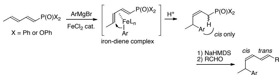
Scheme 11. Iron-catalyzed \delta -addition of aryl Grignard reagents to \alpha,\beta,\gamma,\delta -unsaturated phosphorus compounds.
