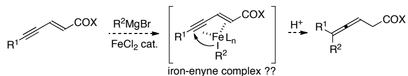
Scheme 12. Extension to conjugated enynes.
