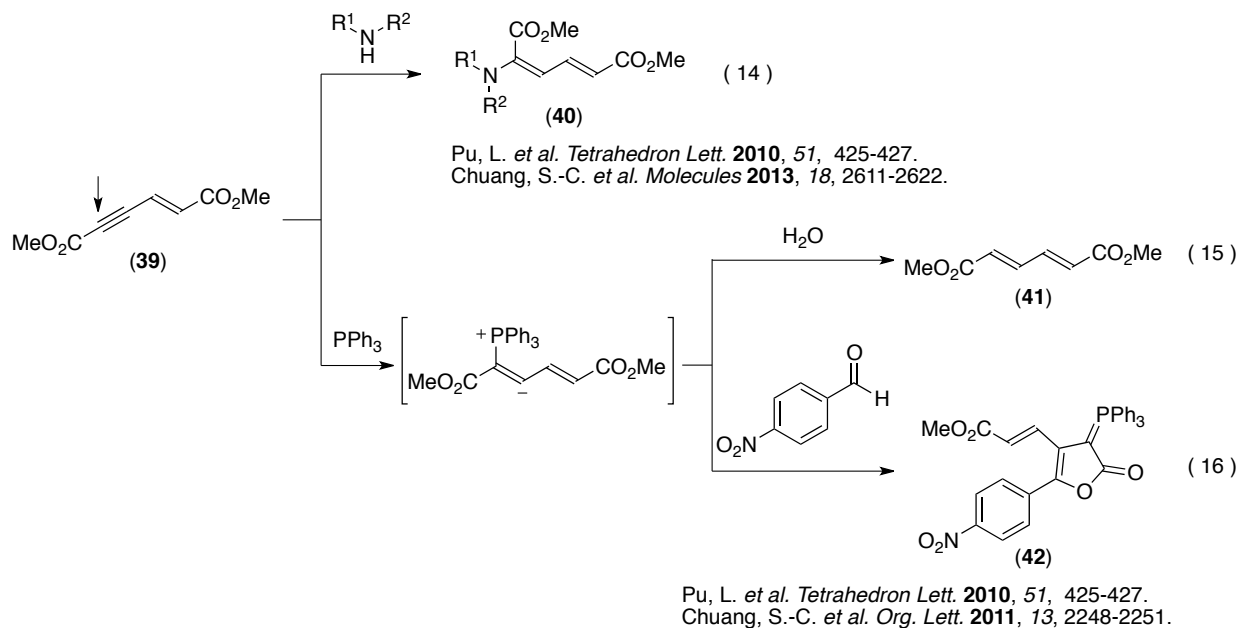
Scheme 6. Nucleophilic addition to 2-alken-4-ynedioates.
