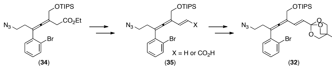
Scheme 5. Synthetic plan A to the same intermediate.
