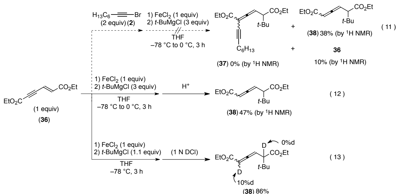
Scheme 5. Grignard addition to 2-alken-4-ynedioate
