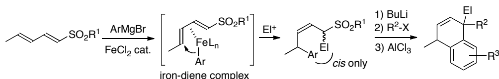
Scheme 10. Iron-catalyzed \delta -addition of aryl Grignard reagents to \alpha,\beta,\gamma,\delta -unsaturated sulfones.
