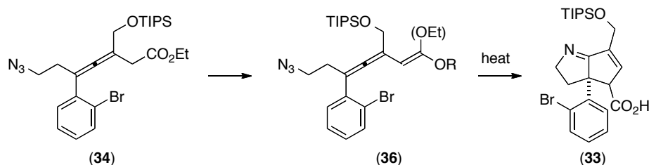
Scheme 6. Synthetic plan B to the similar intermediate.
