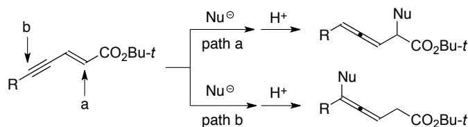
Scheme 2. Michael vs anti -Michael addition to enynoate.
