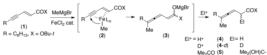
Scheme 13. Iron-catalyzed 1,6-addition of aryl or methyl Grignard reagents to enynoates and -amides.
