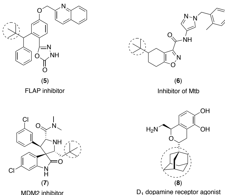
Figure 1. Drug design with tert -alkyl groups.
