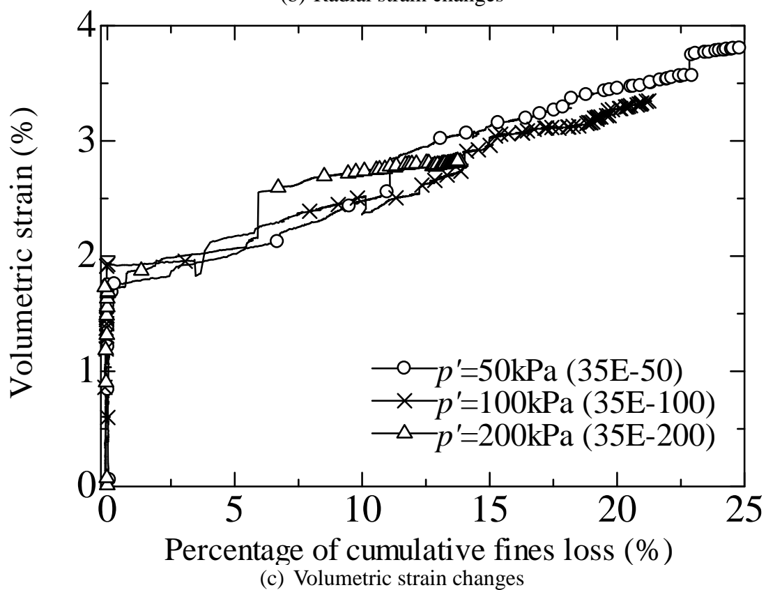
Figure 5.17 Axial, radial and volumetric strain versus percentage of cumulative fines loss under different effective confining pressures for specimens with 35% fines content
