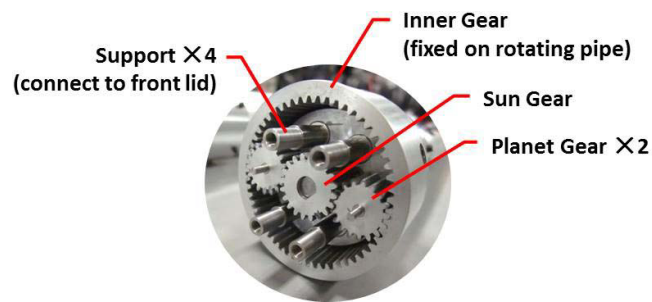
Fig. 5.1.2: Planetary gear set
