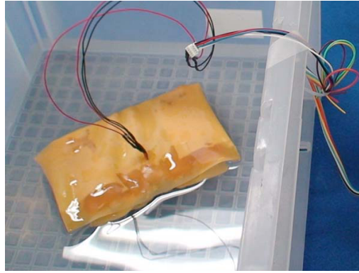
Fig. 3.2.9: Watertightness experiment
