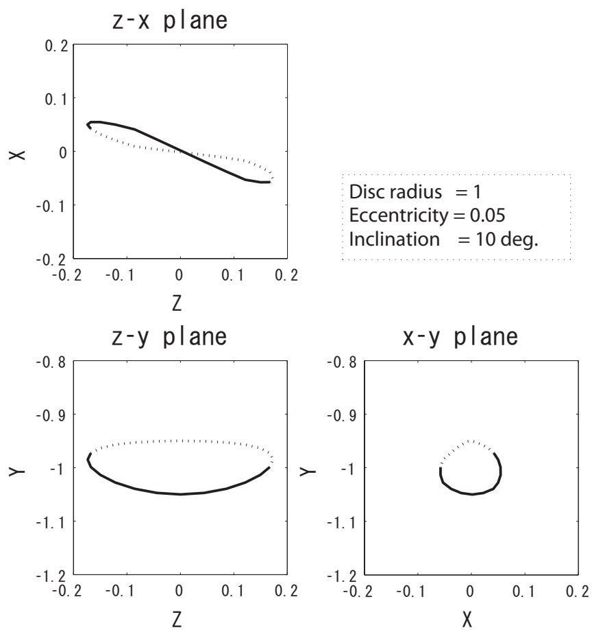
Fig. 4.2.6: Shape of the trajectory in different views
