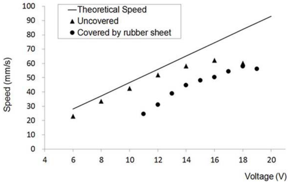
Fig. 3.2.7: Proceeding speed of PD-II
