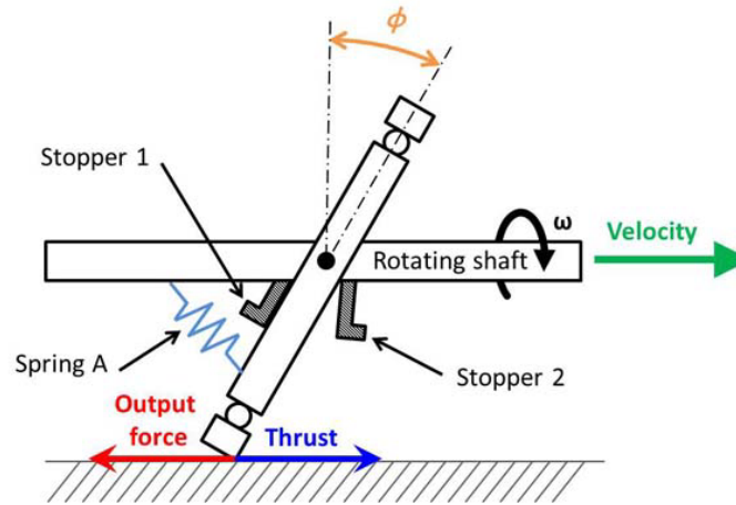
Fig. 6.2.3: Concept of load-sensitive RS-Wave mechanism
