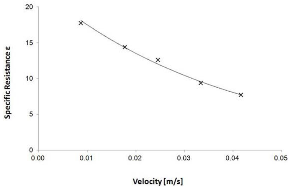
Fig. 5.5.2: Specific resistance \varepsilon calculated with P_L
