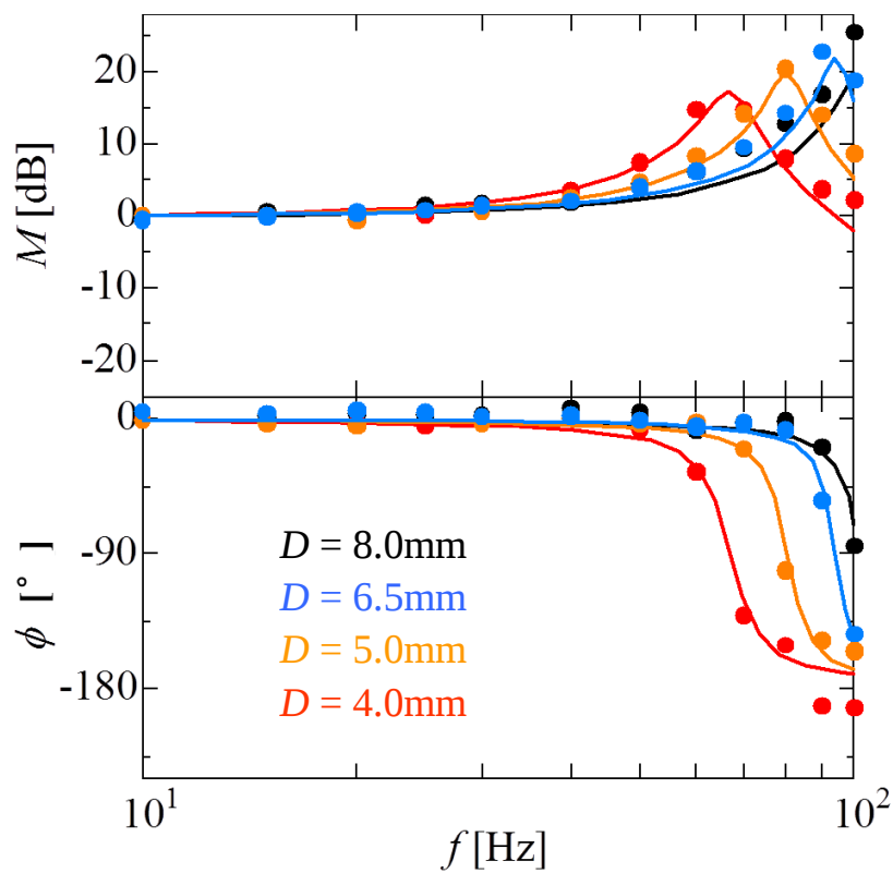
Fig.2.13 Bode diagram ( L = 1.0\text{m} )
