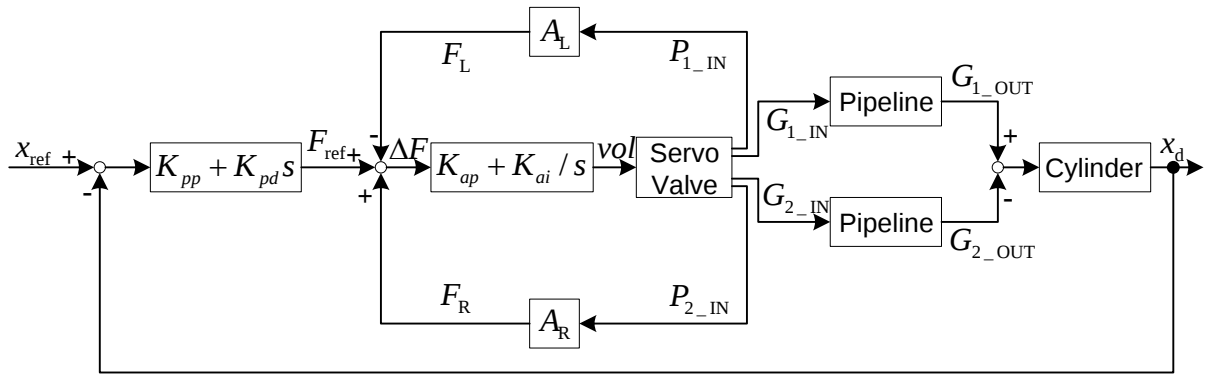
Fig.3.10 Block diagram (pressure signals measured by sensors at the control ports of the servo valve)
