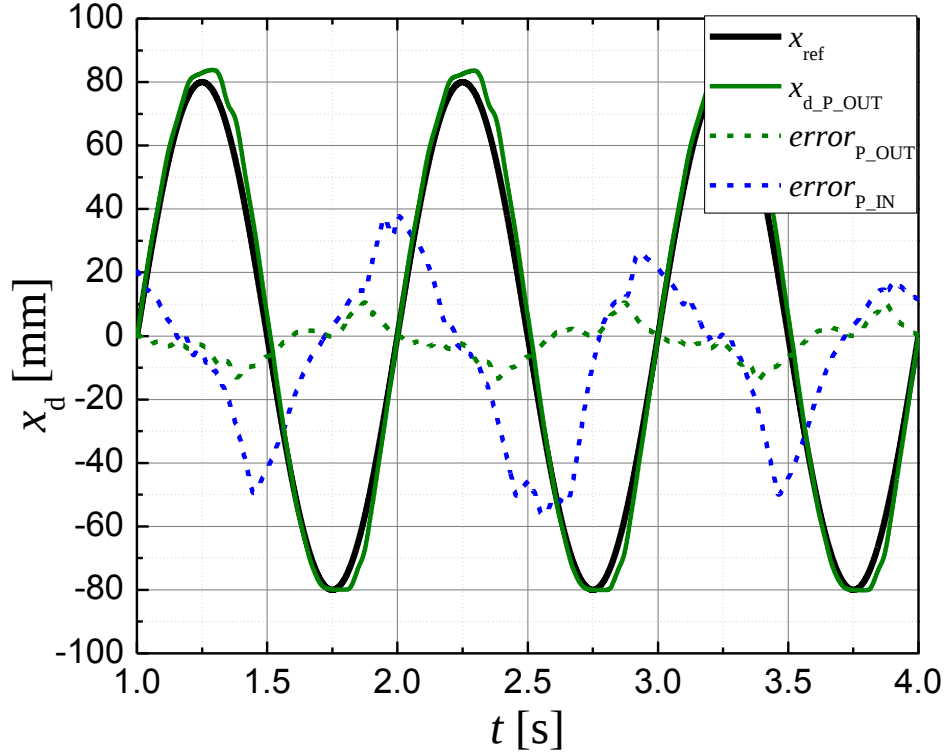
Fig.3.14 Experiment results (pressure signals measured by sensors at the cylinder chambers, D=7.65\text{mm} , L=10.0\text{m} )
