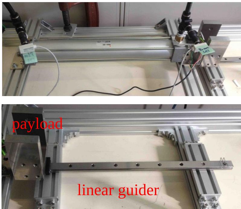
Fig.3.2 Photo of experimental apparatus
