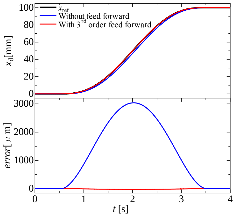
Fig.2.29 Experimental results (3 rd order) ( D = 8.0\text{mm} , L = 1.0\text{m} , \omega_v=100\text{Hz} , \zeta_v = 0.7 )
