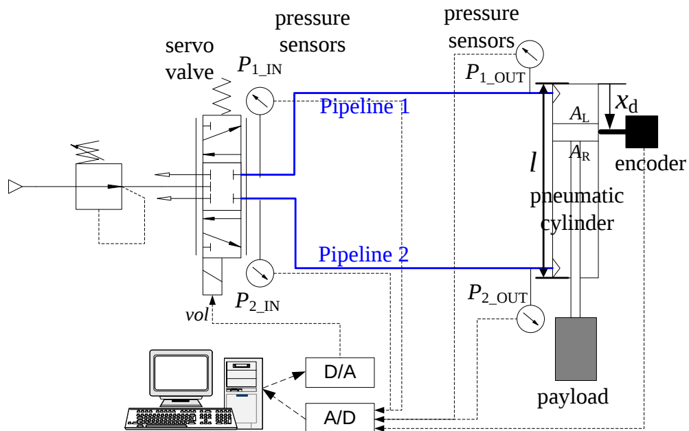
Fig.3.1 Experimental apparatus
