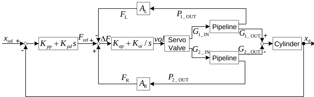
Fig.3.11 Block diagram (pressure signals measured by sensors at the cylinder chambers)
