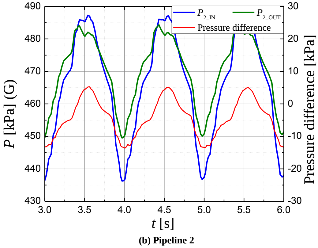
Fig.4.6 Experimental results of pressure ( D=6.10\text{mm} , L=2.0\text{m} , f=1.0\text{Hz} )
