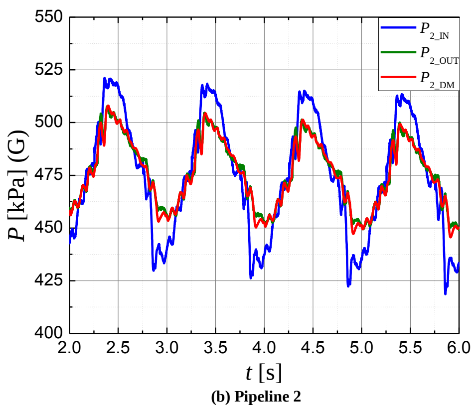
Fig.3.18 Experimental results of pressure (when the system is doing free movement, D=7.65\text{mm} , L=10.0\text{m} )
