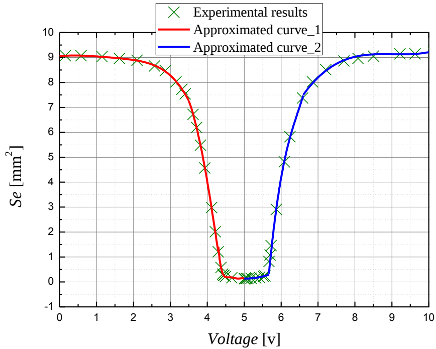
Fig.3.7 Se -Voltage characteristics of the servo valve
