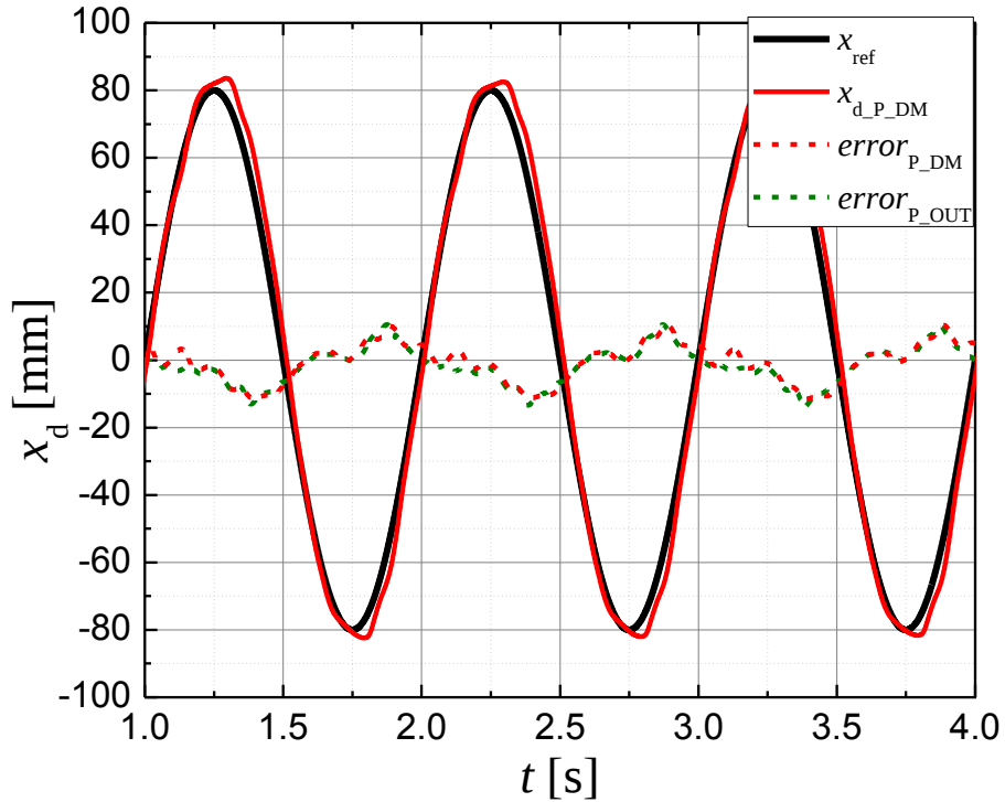
Fig.3.20 Experimental results (pressure signals estimated by the distributed model, the system is done free movement, D=7.65\text{mm} , L=10.0\text{m} )
