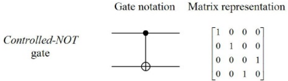
Figure 2.6: CNOT gate..
