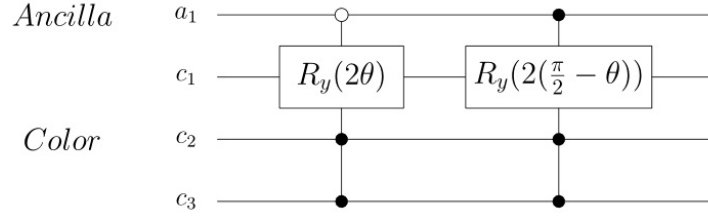
Figure 3.11: The general quantum circuit to realize the \alpha B operator..
