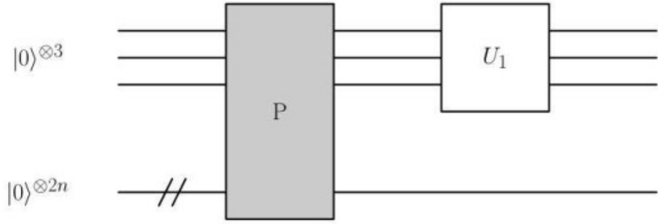
Figure 2.10: Quantum circuit of C_I operations dealing with color channels by U_1 .
