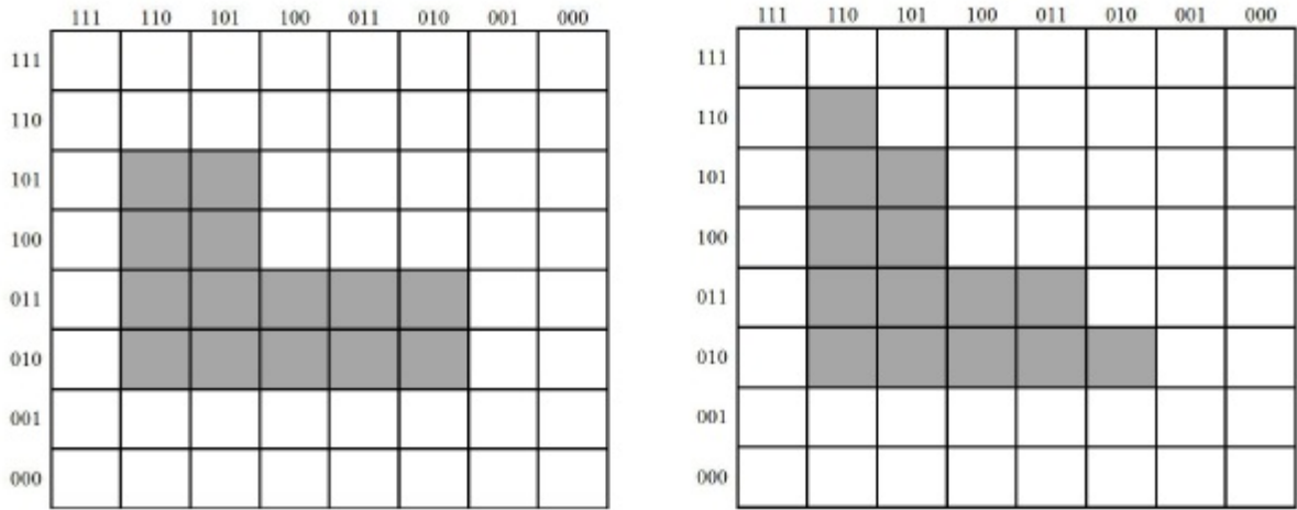
Figure 4.16: An example of two-point swapping operation..
