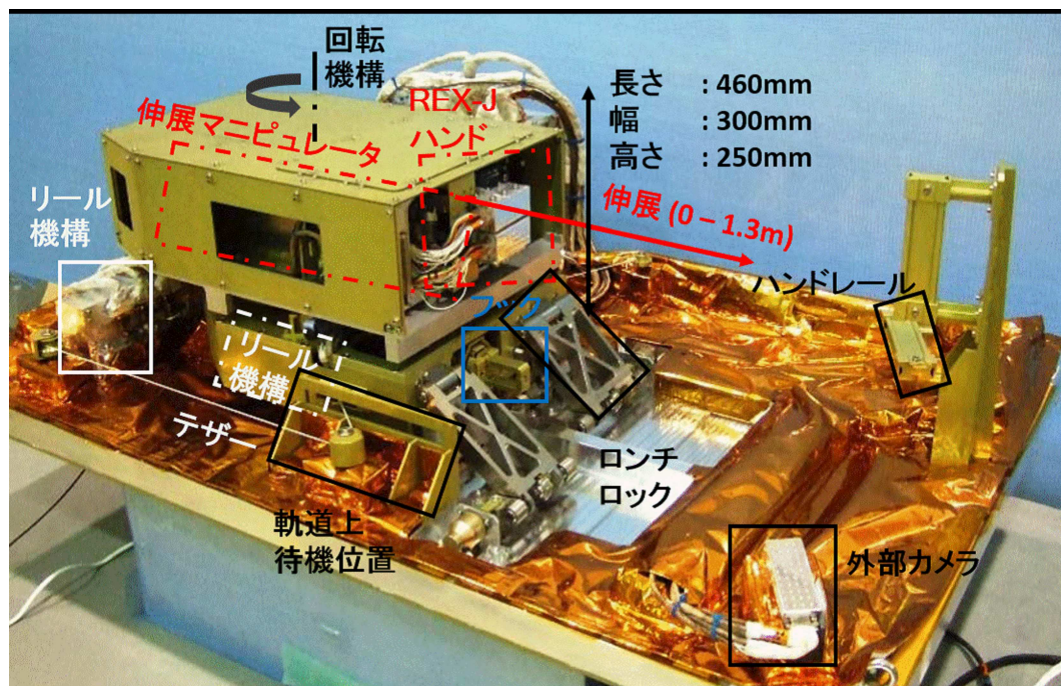
Fig. 5.6 REX-J Flight Model
