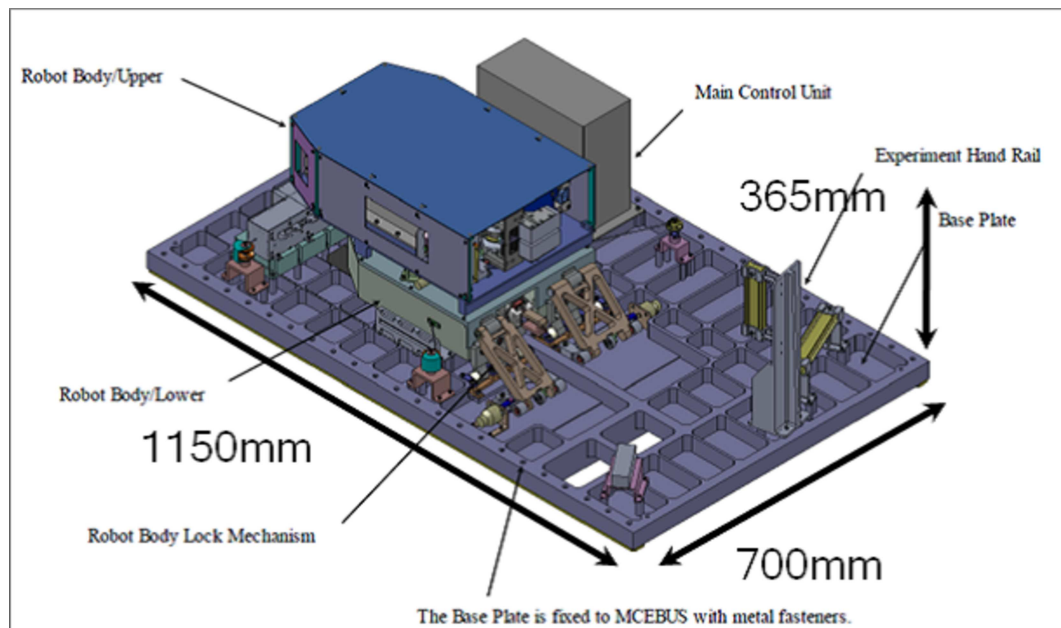
Fig. 5.9 REX-J onboard system
