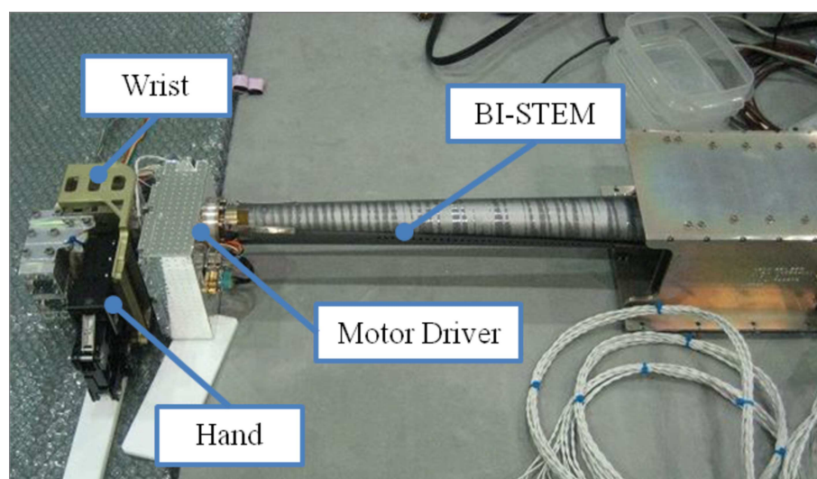
Fig. 2.5 STEM Robot Arm
