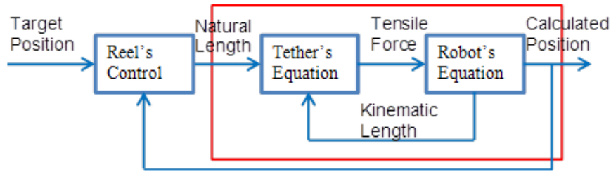
Fig. 3.8 Dynamics Simulator Block Diagram
