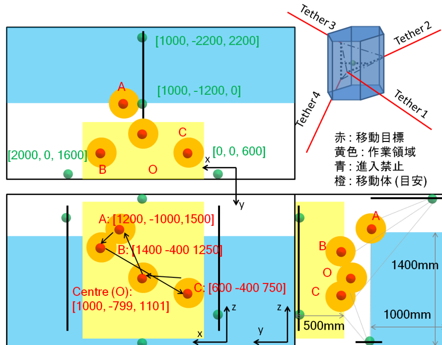
Fig. 4.5 JEM Simulation Model
