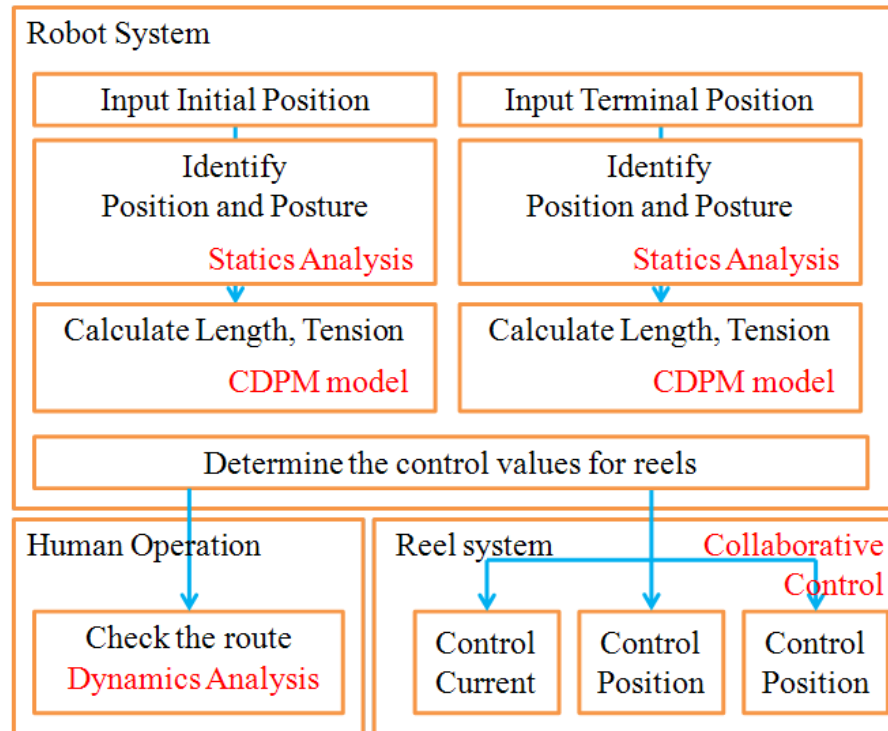
Fig. 3.20 Dynamics Simulator Block Diagram
