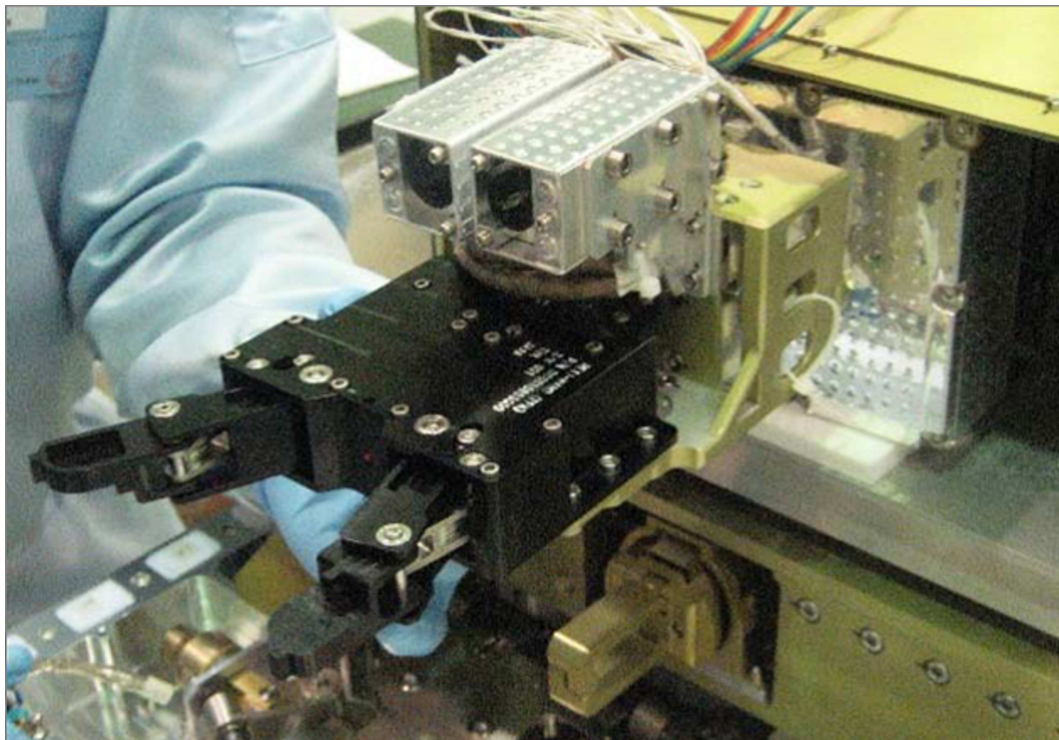
Fig. C.2 STEM Robot Arm Mechanism
