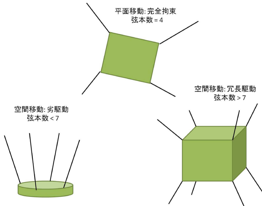
Fig. 3.1 CDPM Class
