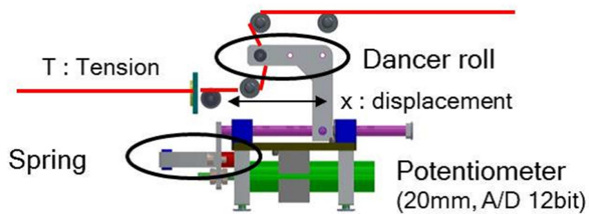
Fig. B.5 Dancer Roll CAD Model
