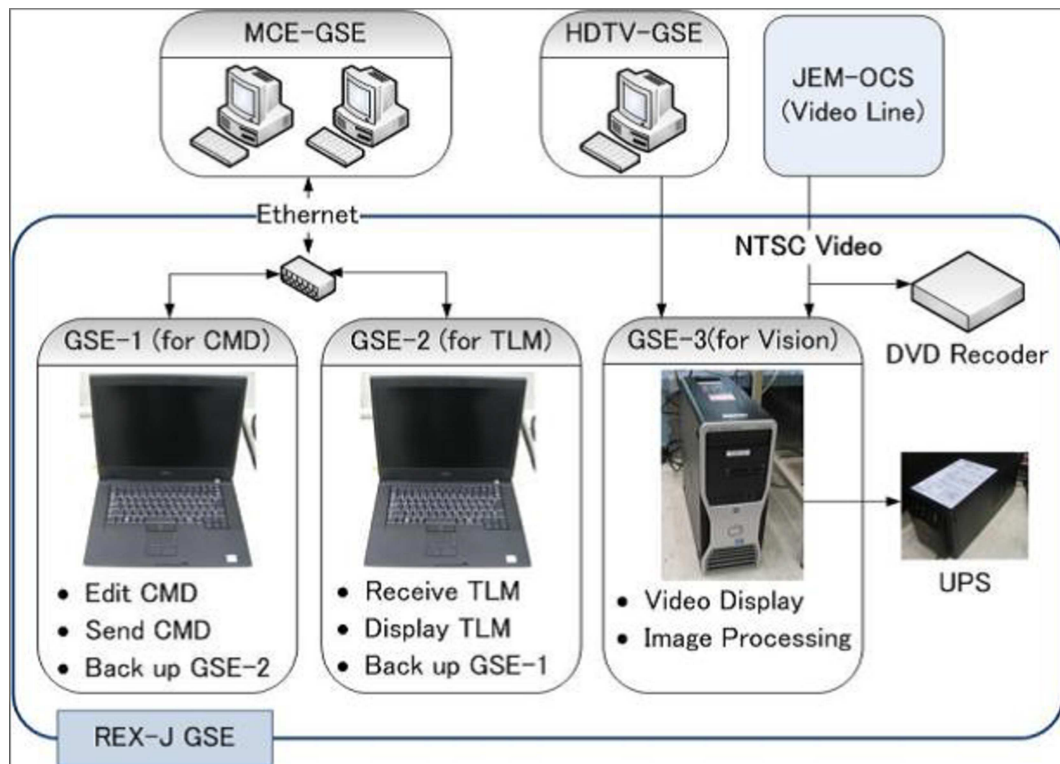
Fig. 5.8 Tele-operation system
