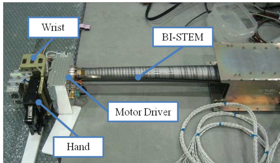
Fig. C.4 PFM of STEM robot arm
