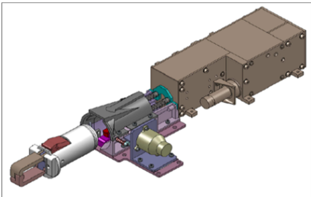
Fig. C.4 PFM of STEM robot arm
