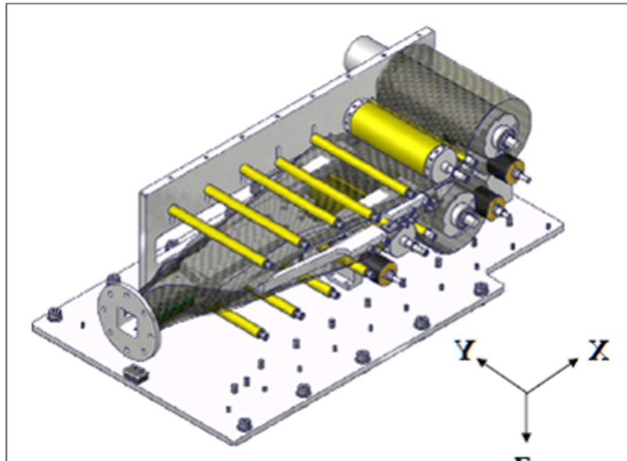
Fig. C.2 STEM Robot Arm Mechanism
