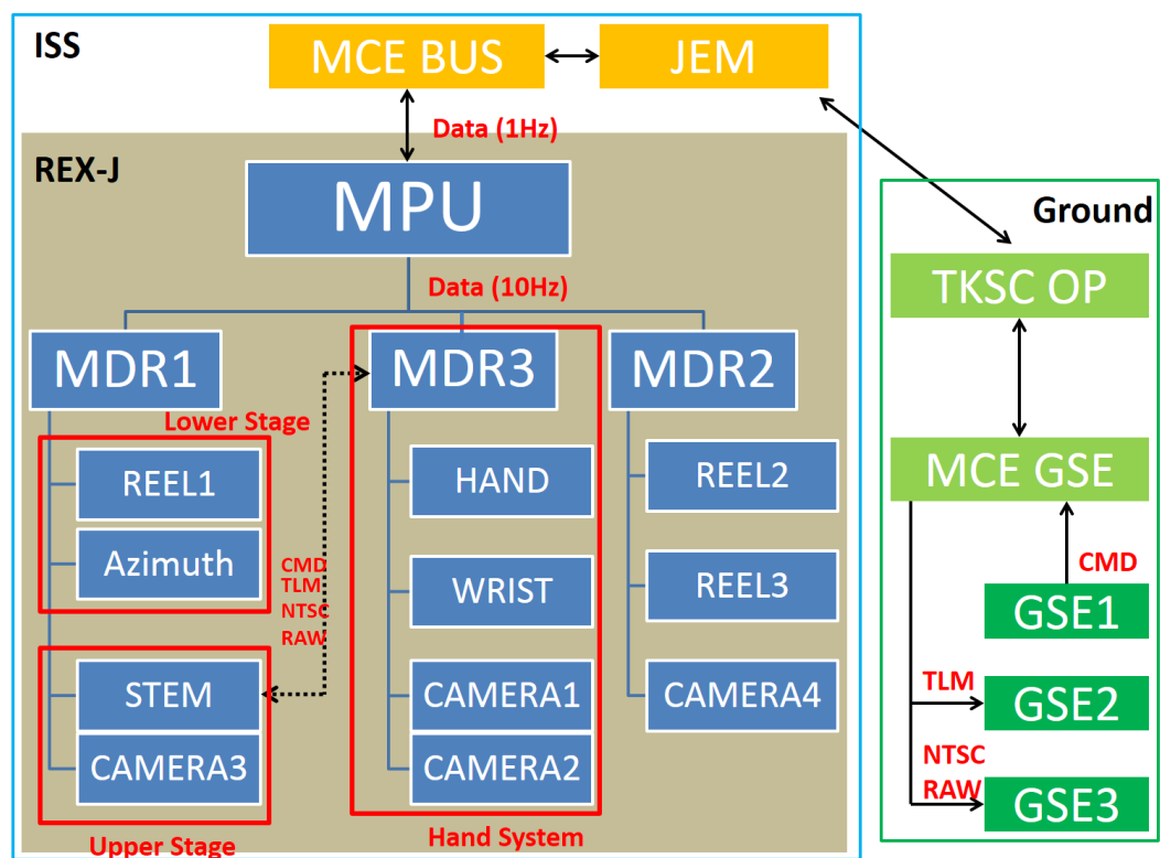
Fig. 5.6 REX-J Flight Model
