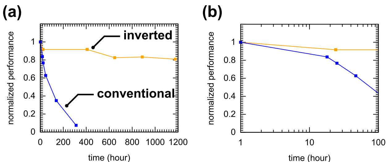
Fig.44 Normalized performance (power conversion efficiency) of conventional and inverted type solar cells. (a) 0 to 1200 hours. (b) 1 to 100 hours. The performance of conventional device was degraded more than 50% after 100 hours; however, inverted device kept its performance 80% after 1200 hours. This degradation was due to the oxidation of aluminum electrode.
