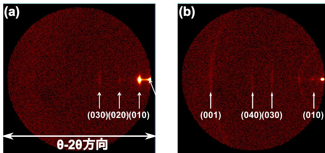
Fig.50 2-dimensional X-ray diffraction patterns of DmPP-O12 and PC 61 BM (2:1 w/w) composite thin film, (a) before and (b) after the thermal annealing.
