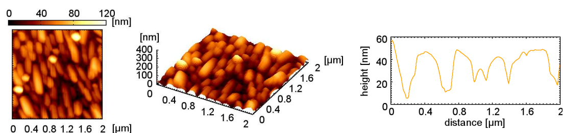
Fig.54 Topography images of DmPP-O12/PC 61 BM (2:1 w/w) composite thin film on a glass substrate determined by AFM. Dynamic force microscope (DFM) mode was used because the organic material was sensitive to a mechanical contact. Measured area was 2.0 \times 2.0 \mu\text{m}^2 . (a) Before and (b) after the thermal annealing. Before thermal annealing, the surface was flat (RMS: 2.0nm) owing to an amorphous nature of PC 61 BM. On the other hand, after annealing, the surface was changed into rough, and a lot of grains were observed.
