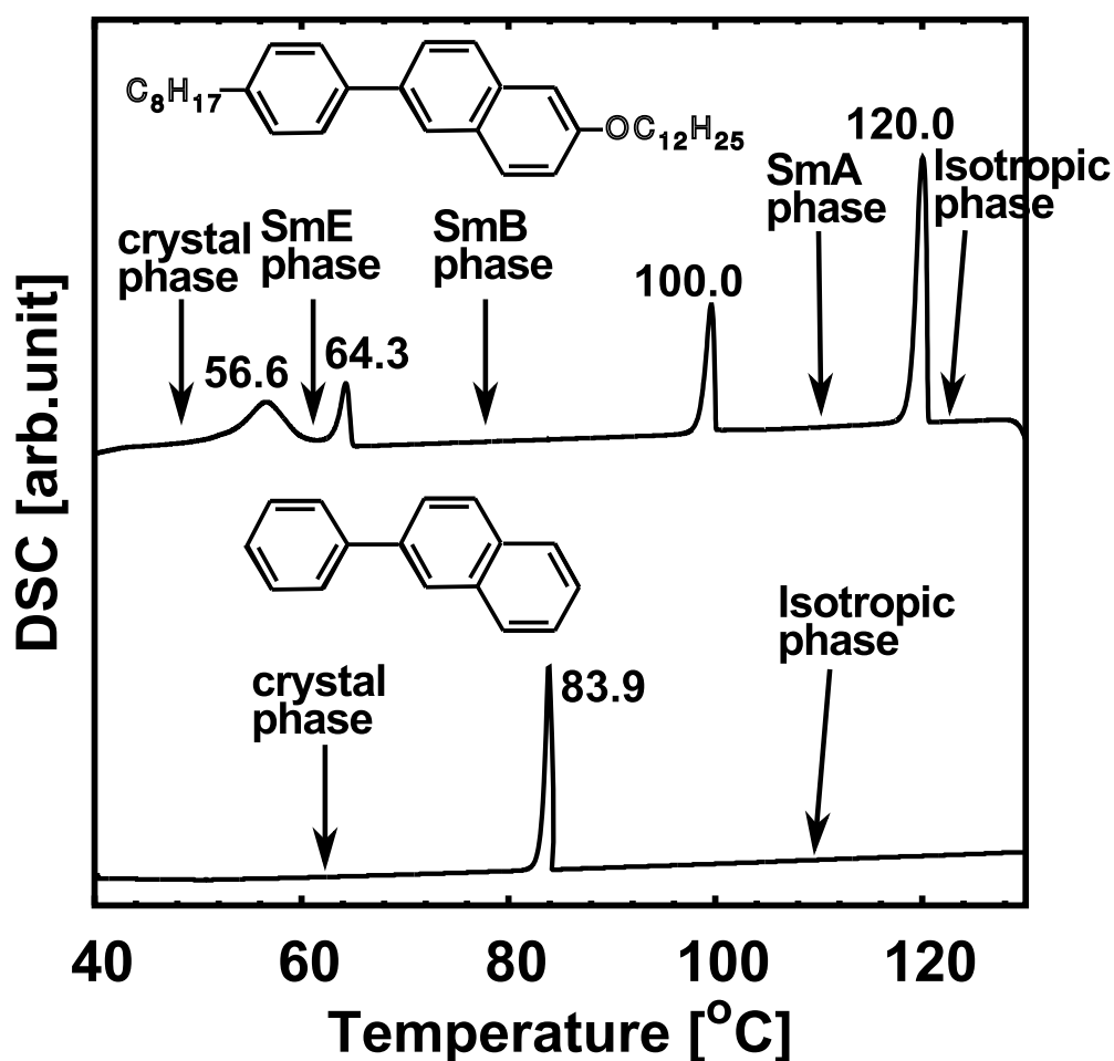
Fig.29 Phase transition behaviors of liquid-crystalline phenyl-naphthalene 8-PNP-O12 and non-liquid-crystalline PNP, determined by differential scanning calorimetry. Temperature scanning rate was 5°C/min. PNP has only one phase transition from isotropic to crystal, which means a melting point. On the other hand, 8-PNP-O12 has four peaks corresponding to SmA, SmB, SmE, and crystal phase transition.
