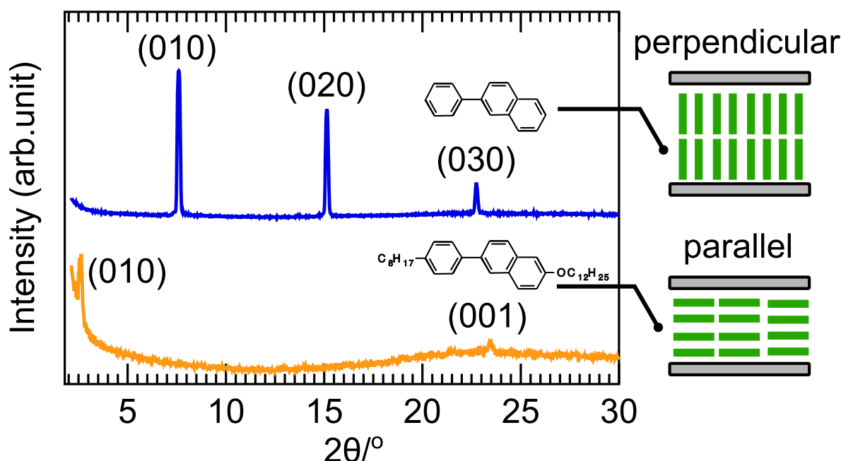
Fig.32 XRD of 8-PNP-O12 and PNP doped with perylene tetraester (10 mol%). The orange line is the result for 8-PNP-O12, and the blue one is for PNP. These films were prepared by removing the glass substrate of the liquid crystal cells with cell thickness of 1\mu\text{m} . XRD measurement was carried out at room temperature.
