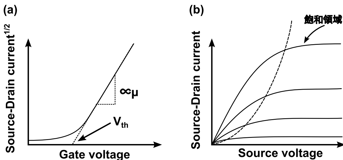
Fig.8 Typical characteristics of organic thin film transistor. (a) Transfer characteristics. (b) Output characteristics.
