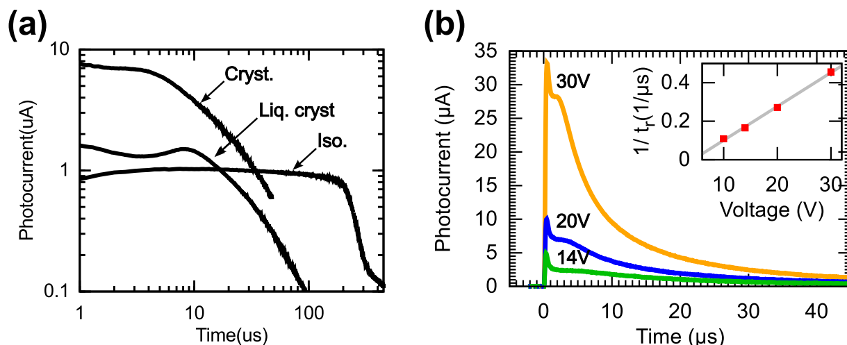
Fig.17 (a) Results of time-of-flight measurement with 8-QTP-8. The cell thickness was 22\mu\text{m} . Measurement was carried out at 205, 110 and 24^\circ\text{C} for isotropic, liquid crystalline and crystalline phases, respectively. An applied voltage was 70, 10 and 20V, respectively. In all cases, clear kink point was observed. The carrier mobility was calculated from the kink points as 3.02 \times 10^{-4} , 4.84 \times 10^{-2} , and 4.84 \times 10^{-2} \text{ cm}^2/\text{Vs} for Isotropic phase, liquid crystalline phase, and polycrystalline phase. (b) Transient photocurrents of 8-QTP-8 at polycrystalline phase ( 25^\circ\text{C} ). The cell thickness was 22\mu\text{m} . The inset shows the inverse of transit time as a function of applied voltages, indicating mobility independent of electric field.
