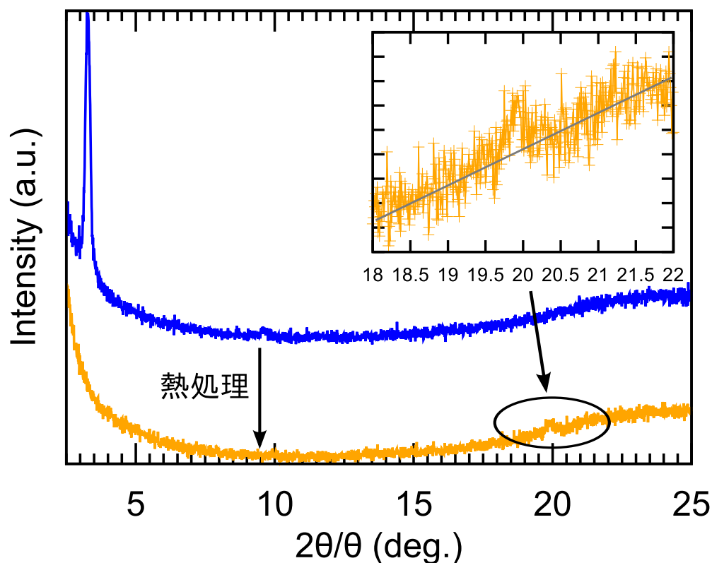
Fig.49 X-ray diffraction patterns of DmPP-O12 and PC 61 BM (2:1 w/w) composite thin film, before (blue line) and after (orange line) the thermal annealing. In both cases, measurement was conducted through a 100 nm Al electrode onto the thin film layer. The inset shows an enlarged view from 18° to 22°. The gray line is calculated by least-squares method.
