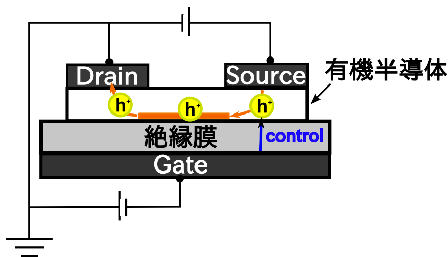
Fig.10 Schematic illustration of device operation of OFETs.
