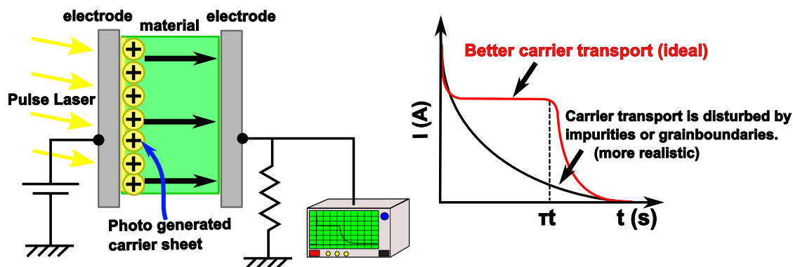
Fig.7 Experimental setup for the time-of-flight measurement. Material is sandwiched by a pair of electrodes. When a pulse laser is illuminated from one side of the electrode, carrier sheet is generated, and conducted by an applied voltage. The carrier conduction is measured as a displacement current with an oscilloscope. Ideal transient photo-current has a kink point like a red line; however in many cases, we just obtain the current like black line owing to the grain boundaries and impurities.
