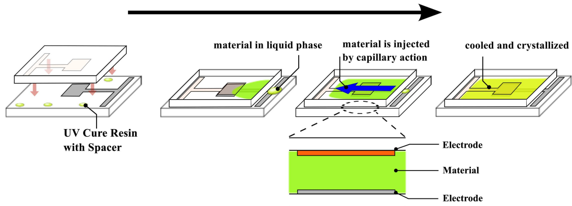
Fig.6 Schematic illustration of fabrication process of glass cell, and injection of a material into the cell.
