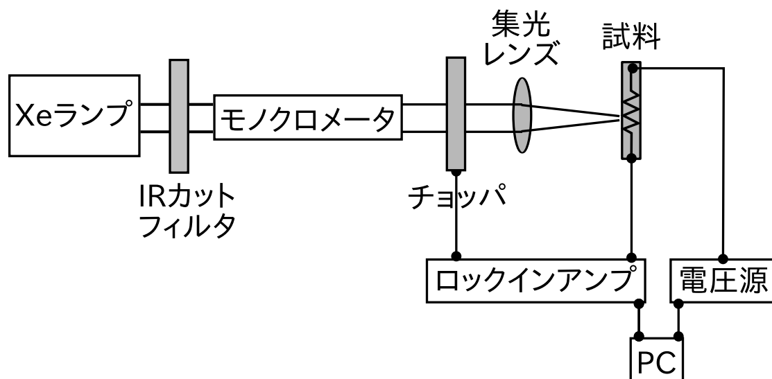
Fig.60 Experimental system for external quantum efficiency. Light source is 500W Xe lamp. The light passes through an IR-cut filter which removes longer wavelength than 800nm. Then the light is separated into single-wavelength by monochromator. A mechanical chopper chops the light with a duty ratio 0.5 in a frequency of 20Hz. Finally, the light is concentrated by a condensing lens and illuminated into a sample. An output signal of the chopper is put into a lock-in amplifier as a reference signal which synchronizes chopper with lock-in amplifier.
