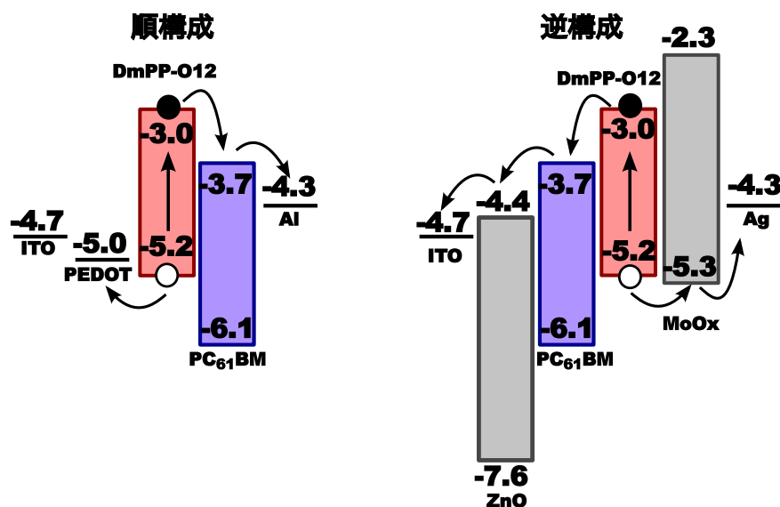
Fig.42 Conventional and inverted structure of organic solar cells.
