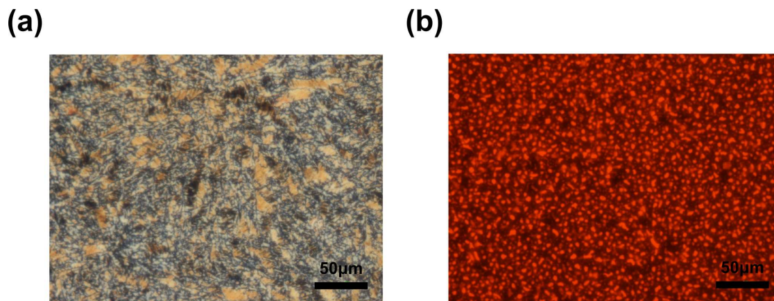
Fig.28 Microscopy images of 8-PNP-O12 doped with 10mol% perylene tetraester. (a) With polarized microscope. (b) With fluorescence microscope. Both measurement was carried out at room temperature with 1.50\mu\text{m} cell. The excitation light wave length for fluorescence was 510-560 nm, and the resulting fluorescence was detected at 590 nm. Only the fluorescence from the perylene tetraester was observed.
