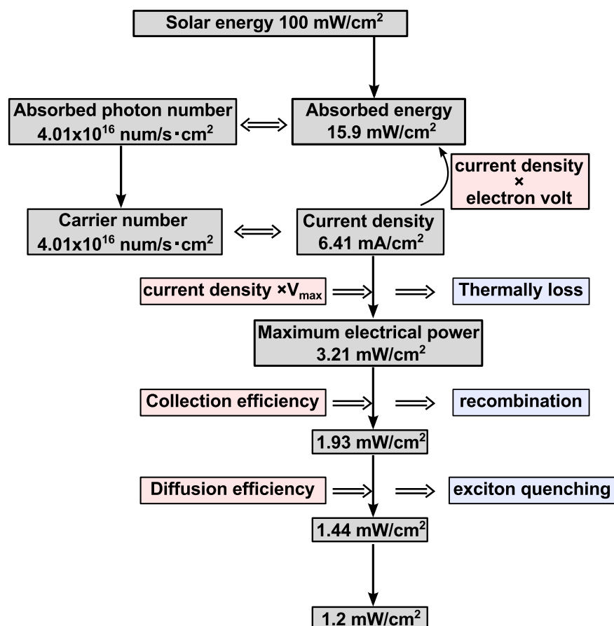
Fig.65 Calculation of efficiency beginning with solar energy.
