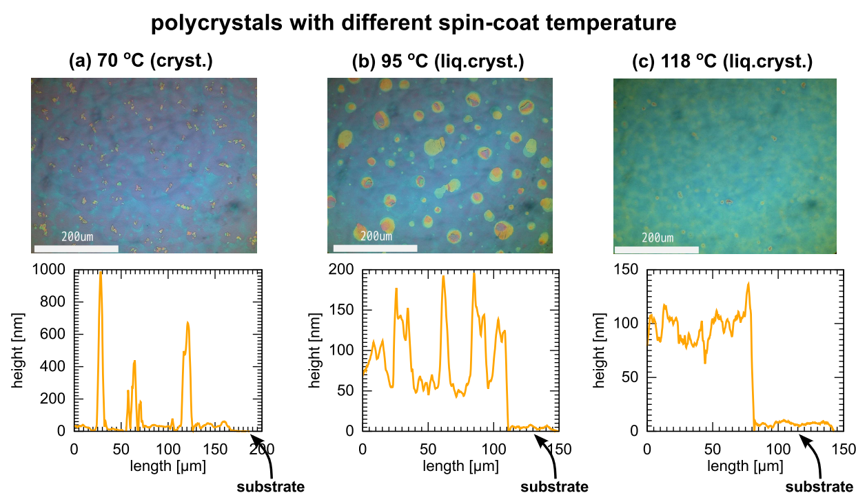
Fig.13 Microscope images of 8-QTP-8 thin film fabricated by spin-coating under various temperature condition. (a) Under 70 °C (crystalline phase). (b) Under 95 °C (Liquid crystalline phase). (c) Under 118 °C (Liquid crystalline phase). Spin-coating was carried out with 1wt% diethylbenzene solution at 3000rpm for 30s. Below each photograph, a profile section determined by laser micrograph was shown. Under 70 °C, the resulting film didn't cover the whole substrate, and there were numerous cluster of polycrystal. On the other hand, under 95 and 118 °C, thin films completely covered the substrate.
