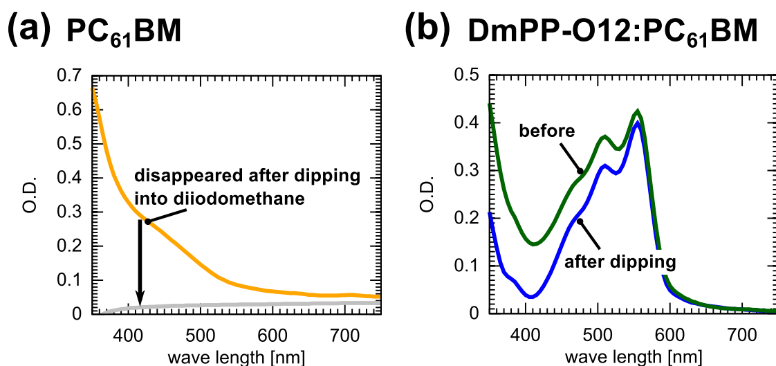
Fig.5.5 Absorption spectra of (a) PC 61 BM, (b) DmPP-O12/PC 61 BM (2:1 w/w) composite thin film. These films were dipped into diiodomethane to remove PC 61 BM. Indeed, absorption of PC 61 BM was disappeared after dipping for 30s. In the composite film, absorption less than 550nm was decreased owing to removing PC 61 BM.
