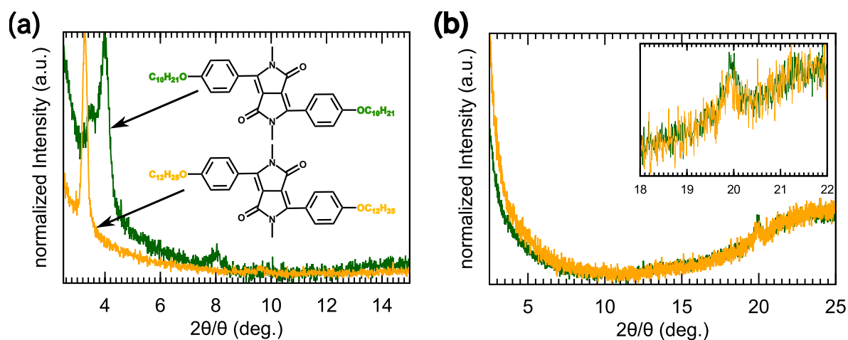
Fig.51 X-ray diffraction patterns of DmPP-O12/PC 61 BM (2:1 w/w) and DmPP-O10/PC 61 BM composite thin film. (a) Before and (b) after the thermal annealing. In both cases, measurement was conducted through a 100 nm Al electrode onto the thin film layer. The d-spacing calculating from lower peaks were smaller in the case of DmPP-O10 than DmPP-O12. This results indicate this sharp peak can be attributed to the molecular long axis. On the other hand, small peak around 20° appeared in both cases, which meant this peak can be attributed to inter molecular distance.
