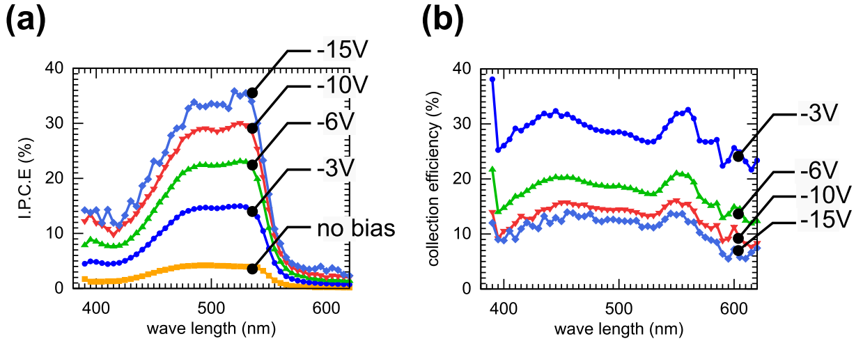
Fig.62 (a) IPCE spectra of preceding sample (inverted structure) before thermal annealing. Reverse biases were applied from 0 to -15V. The quantum efficiencies were improved by the applied bias owing to the enhancement of carrier collection. (b) Carrier collection efficiency calculated from the results of photo-current measurement under reverse bias.
