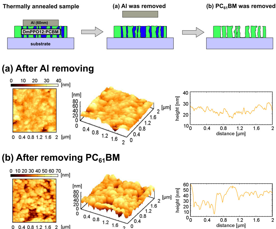
Fig.5.7 Topography images of DmPP-O12/PC 61 BM (2:1 w/w) composite thin film on a glass substrate with Al back-contact electrode. (a) after removing Al, (b) after dipping into diodomethane for 60s. The film had been thermally annealed at 60 °C for 30s before removing the Al electrode. Measured area was 2.0 \times 2.0 \mu\text{m}^2 .
