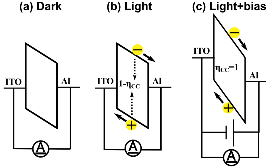
Fig.59 energy diagram under short circuit condition. (a) under dark. The fermi level of each electrode is matched owing to the short circuit. (b) Under light. Carriers are generated in D/A interfaces and transported along a internal electric field. Carrier collection efficiency is discribed as \eta_{CC} . Some of carriers recombine or become charge transfer exciton again in the ratio of 1-\eta_{CC} . (c) Under light and reverse bias. In this condition, there is a large internal electric field which enhances carrier collection. Hence, \eta_{CC} is close to 100%.
