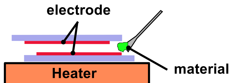
Fig.16 Schematic illustration of injection process of material into glass cells. Glass cell is heated at isotropic temperature: material put at the edge of the cell is melting and injected by capillary action. This process naturally causes crystallization via liquid crystal phase.
