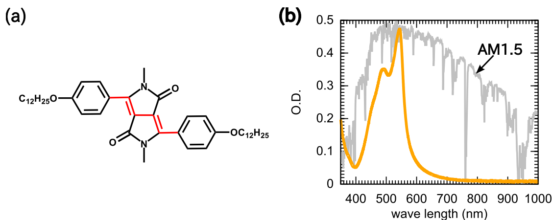
Fig.37 (a) Chemical structure of 3,6-bis(4-(dodecyloxy)phenyl)-2,5-dimethylpyrrolo[3,4-c]pyrrole-1,4(2H,5H)-dione (DmPP-O12). (b) Absorption spectra of DmPP-O12 in polycrystalline thin film. The film was fabricated by spin-coating at room temperature with 1wt% chloroform solution
