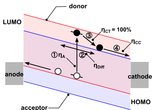
Fig.58 Schematic illustration of photo-carrier generation processes of organic thin film solar cells. (1) Light absorption in the donor material. (2) Photo-generated excitons diffuse in the bulk. (3) The excitation reached D/A interface changes into charge transfer exciton state. (4) Charge transfer exciton state dissociates into electron and hole, and the free carriers are collected by internal electric field.
