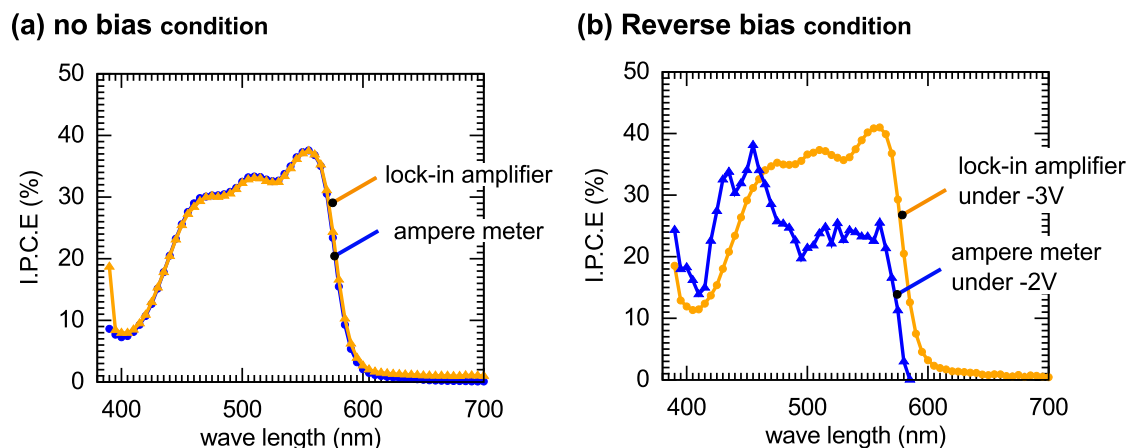
Fig.61 Results of photo-current measurement with a lock-in amplifier and an ampere meter. (a) Without applied bias. (b) Under reverse bias. Measured sample was inverted type with DmPP-O12:PC 61 BM composite photovoltaic layer (same as preceding sample). No bias condition, calculated IPCE measured with a lock-in amplifier well agrees with that measured with an ampere meter. On the other hand, under reverse bias, we could not measure exact photo-current with the ampere meter owing to large dark current. In contrast, the lock-in amplifier gave us reliable results.
