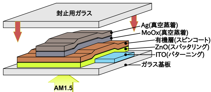
Fig.41 Solar cell structure.
