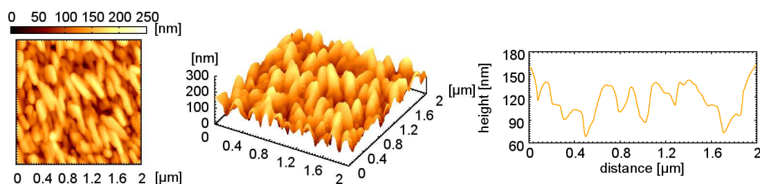
Fig.56 Topography images of DmPP-O12/PC 61 BM (2:1 w/w) composite thin film on a glass substrate. (a) Before and (b) after dipping into diodomethane for 30s. The film had been thermally annealed at 60 °C for 30s before dipping. Measured area was 2.0×2.0μm 2 . Numerous grains owing to the thermal annealing was maintained after dipping. That indicates these grains consist of DmPP-O12, and PC 61 BM was swept out from the liquid crystalline material.
