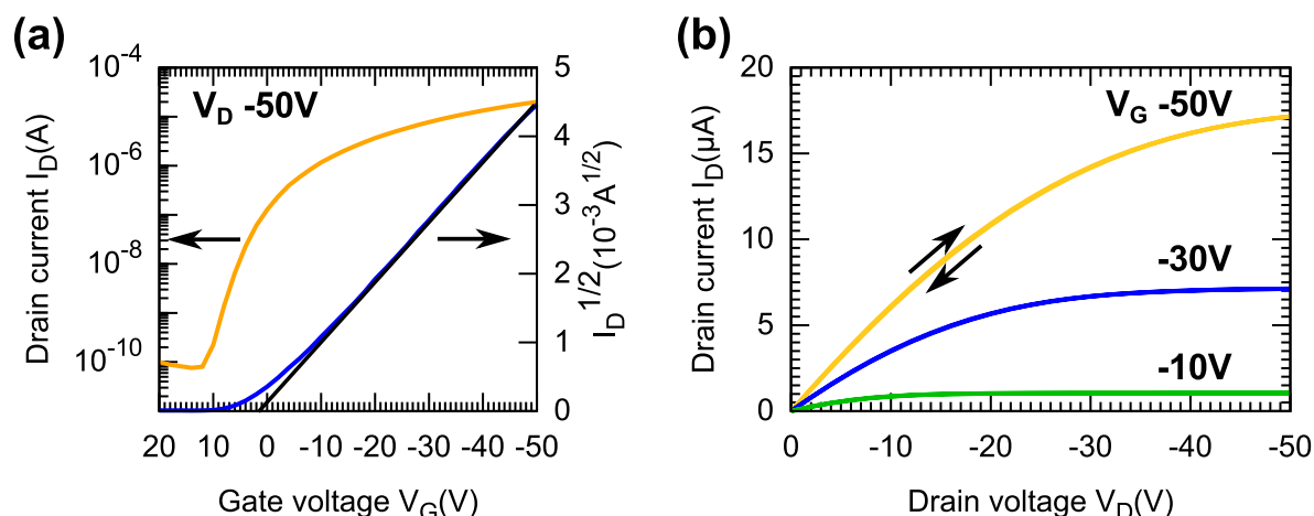
Fig.21 Transfer and output characteristics of OFET with the semiconductor layer of 8-QTP-8. The channel length and width of FETs were 100\mu\text{m} and 1000\mu\text{m} , respectively. The FET mobility was estimated to be 0.14\text{ cm}^2/\text{Vs} in the saturation regime. V_{th} and on-off ratio were 1.9\text{ V} and 10^5 , respectively.
