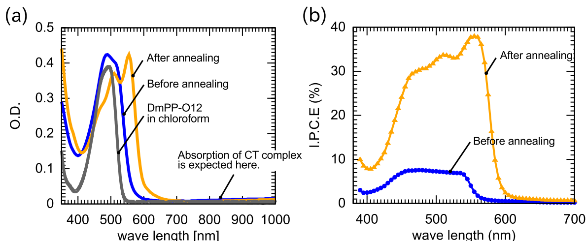
Fig.46 (a) Absorption spectrum of DmPP-O12:PC 61 BM composite thin film of about 200nm. 1 \times 10^{-5} mol/L chloroform solution was also measured for comparison. (b) Incident photon to current efficiency (IPCE) of the cell before and after annealing. Light absorption redshifted after thermal annealing owing to the enhanced molecular interaction of the donor material. The absorption in the visible region increased by about 30% after the thermal annealing, but this cannot explain such drastic improvement in the cell performance. The IPCE spectra also red-shifted corresponding to the redshift of the absorption, while the value of the IPCE is enhanced in the entire spectrum range.
