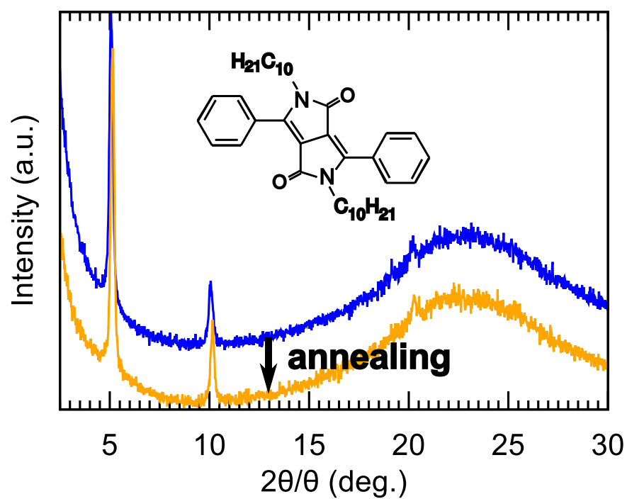
Fig.52 X-ray diffraction patterns of non-liquid crystalline Dec-PP-Ph and PC 61 BM (2:1 w/w) composite thin film, before (blue line) and after (orange line) the thermal annealing. In the case of non-liquid crystalline material, molecular orientation did not change.
