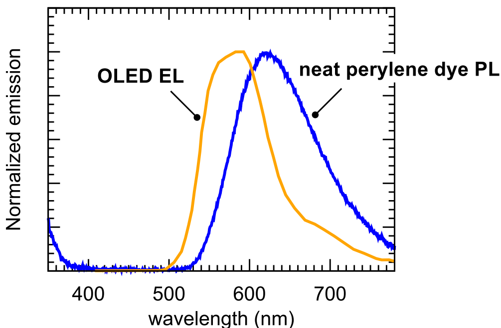
Fig.34 Normalized EL spectra of OLED and PL spectra of neat perylene dye and 8-PNP-O12. The excitation light wave length used for PL measurement was 337 nm. Measurement was carried out at room temperature. EL spectrum didn't completely agree with PL spectrum because molecular interaction of perylene dye was different in neat thin film and mixture thin film.
