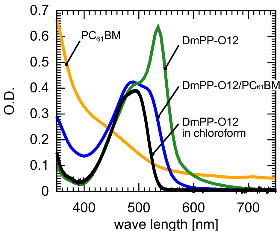
Fig.40 Absorption spectra of DmPP-O12:PC 61 BM mixture, neat DmPP-O12, neat PC 61 BM. Measurement was carried out at room temperature with thin film of about 200nm. 1 \times 10^{-5} mol/L chloroform solution was also measured for comparison. The mixture film has large absorption around 400nm, owing to the absorption of PC 61 BM. The absorption of the mixture blue-shifts compared to neat DmPP-O12 film, because the molecular interaction was weakened in the mixture.
