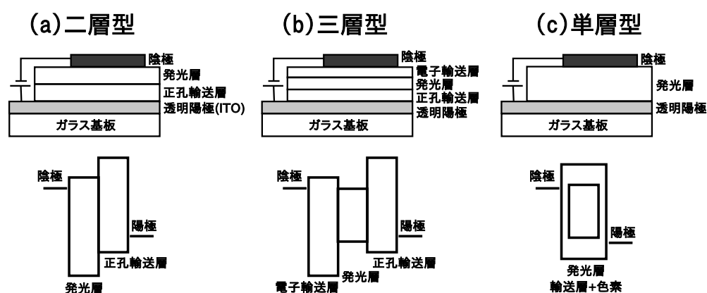
Fig.24 Device structures of typical OLEDs. (a) two-layer, (b) three-layer and (c) single-layer. Energy diagrams are also shown.
