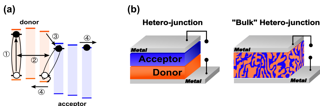
Fig.36 (a) Schematic illustration of photo-carrier generation processes of organic thin film solar cells. (b) Device structures of hetero-junction and bulk hetero-junction.
