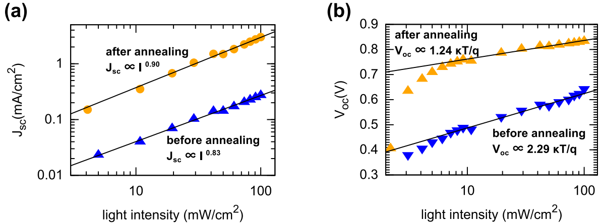
Fig.47 Light dependence of (a) short circuit current ( J_{sc} ), and (b) open circuit voltage ( V_{oc} ).
