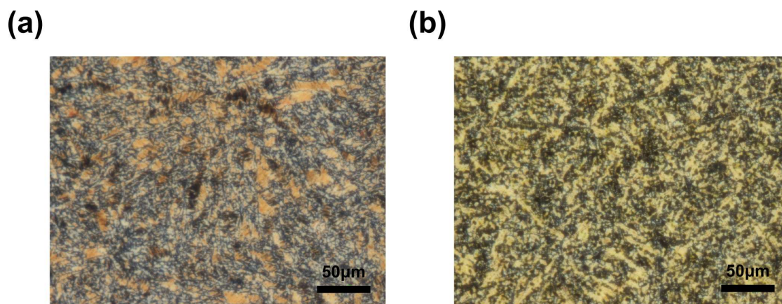
Fig.27 (a) Polarized microscopy image of neat 8-PNP-O12 under crossed nicol. (b) Under the same measurement condition as (a), but 10mol % of perylene tetraester was mixed to 8-PNP-O12. glass cells of 1.36 and 1.50μm were used for (a) and (b), respectively. Measurement was carried out at room temperature.
