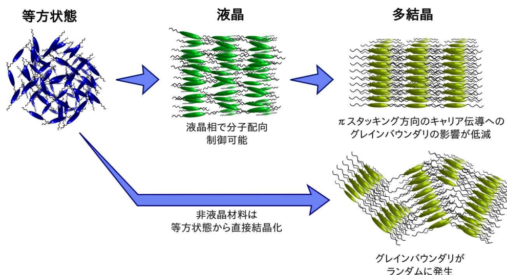
Fig.3 Formation of polycrystalline phase with and without liquid crystalline phase.
