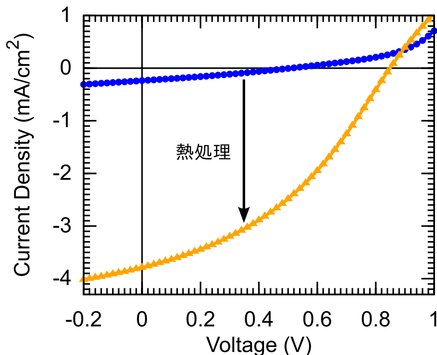
Fig.45 J-V characteristics of ITO/ZnO/DmPP-O12:PC 61 BM=2:1/MoO x /Ag cell under simulated sun light (AM1.5, 100mW/cm 2 ) at room temperature. Electrode area was 4mm×4mm. Thermal annealing was carried out at 60 °C for 30min. Before annealing, the efficiency was 0.035%; however, after the thermal annealing, efficiency was improved more than 30 times than that of before. This enhancement was expected owing to the improvement of both carrier generation and transport.
