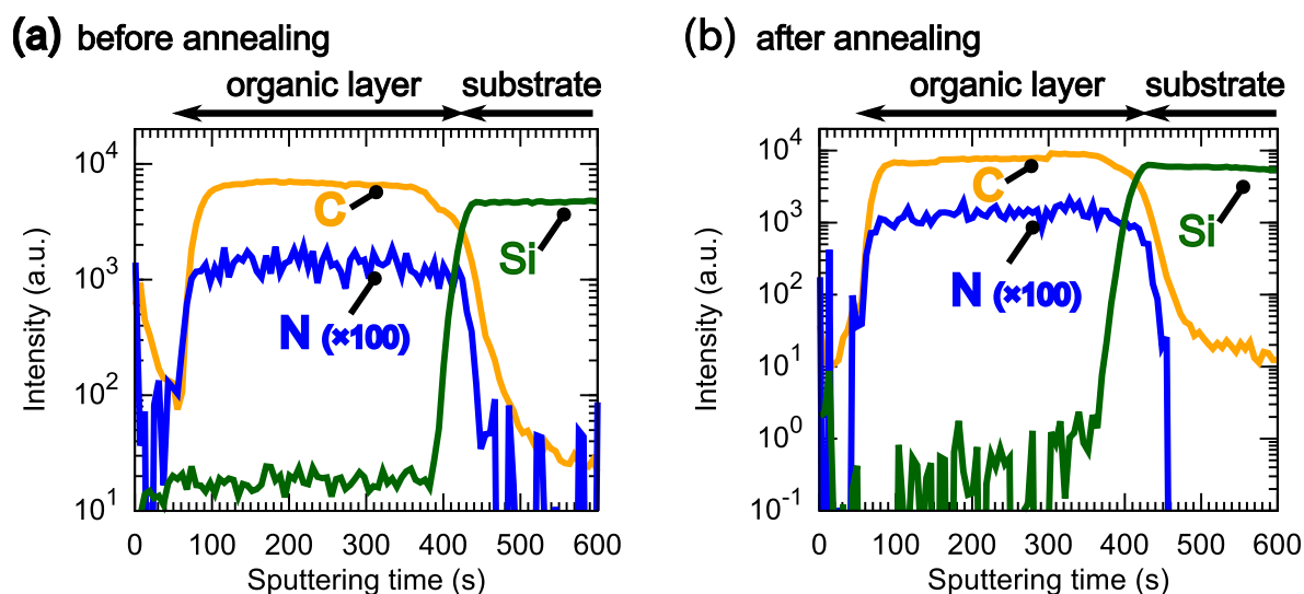
Fig.5.3 Atomic distribution of DmPP-O12/PC 61 BM (2:1 w/w) composite thin film on a glass substrate determined by TOF-SIMS. Primary ion was Bi 3++ , and analyzed area was 300×300μm 2 . (a) Before and (b) after the thermal annealing. In both cases, the distribution of nitrogen which indicated a distribution of DmPP-O12 was uniform in the organic layer. This results mean segregation of each molecules did not occur in a vertical direction to the substrate.
