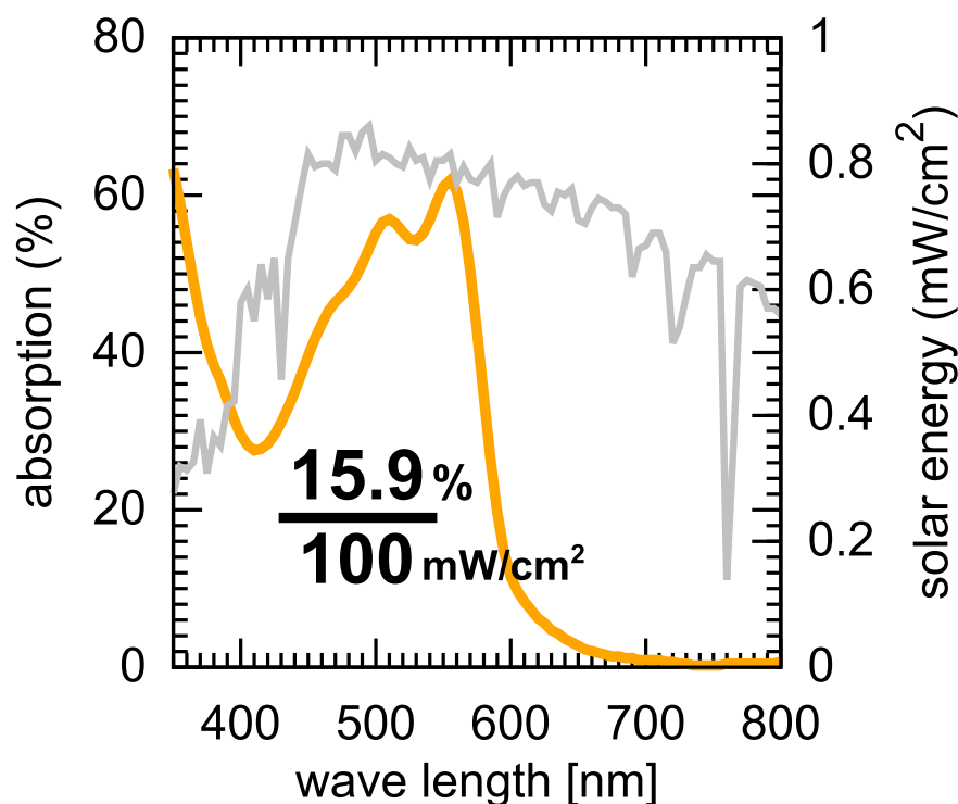
Fig.66 Absorption spectra of DmPP-O12:PC 61 BM=2:1 composite thin film. Solar energy is also shown. The solar power is normalized to its total is 100mW/cm 2 .
