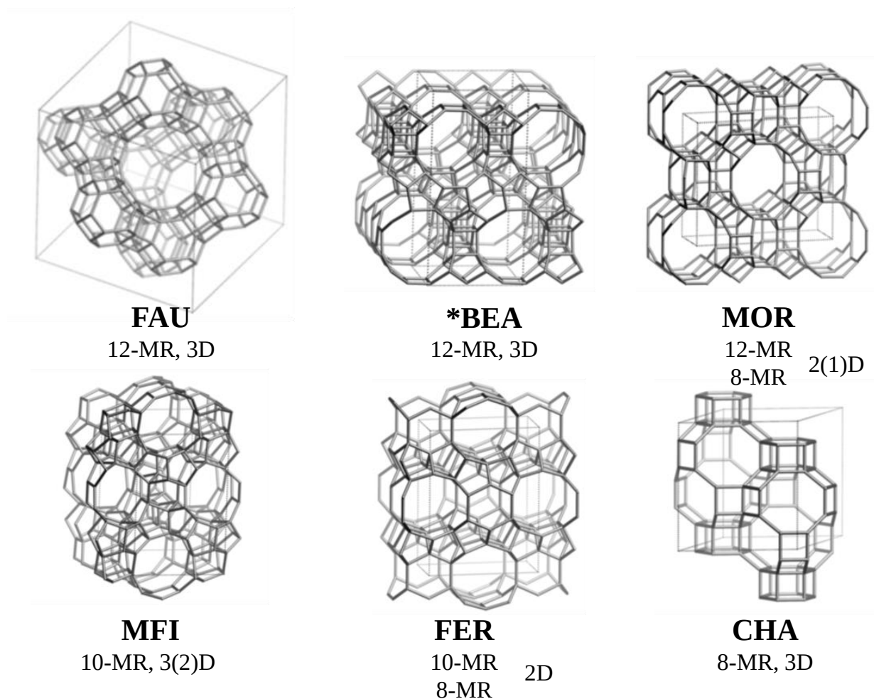
Figure 1.3 Typical zeolite frameworks [9]
