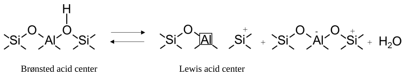
Figure 1.8 Formation model of Lewis acid site by dehydration or hydrolysis of Al-O-Si bond [33]
