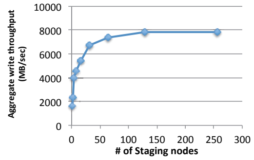
FIGURE 3.13: Aggregate write throughputs
