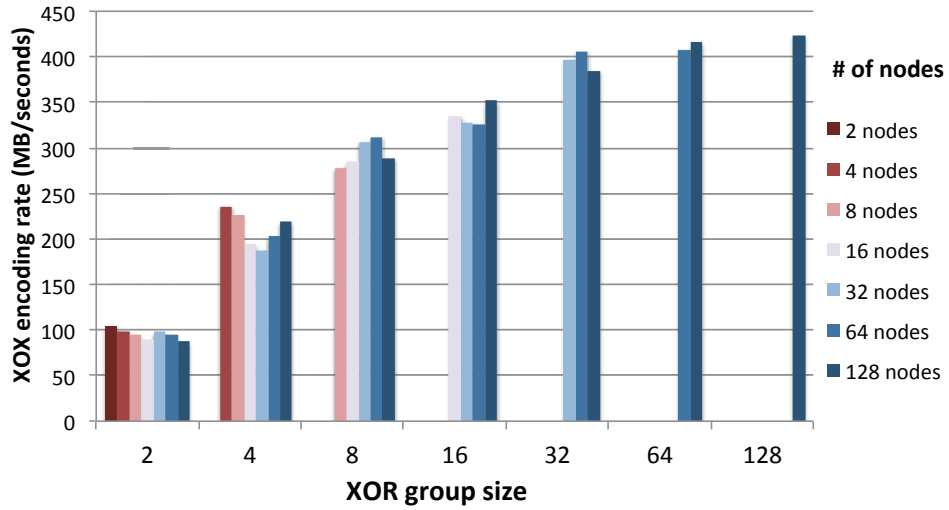
FIGURE 3.19: XOR encoding performance per node
