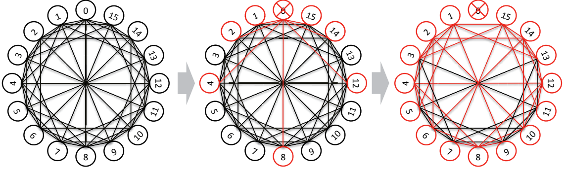
FIGURE 5.8: Left: Structure of the log-ring overlay network ( n = 16 ). Middle: If process 0 fails, processes 1, 2, 4, 8, 12, 14, and 15 are notified by ibverbs. Right: All processes are notified with 2 hops.
