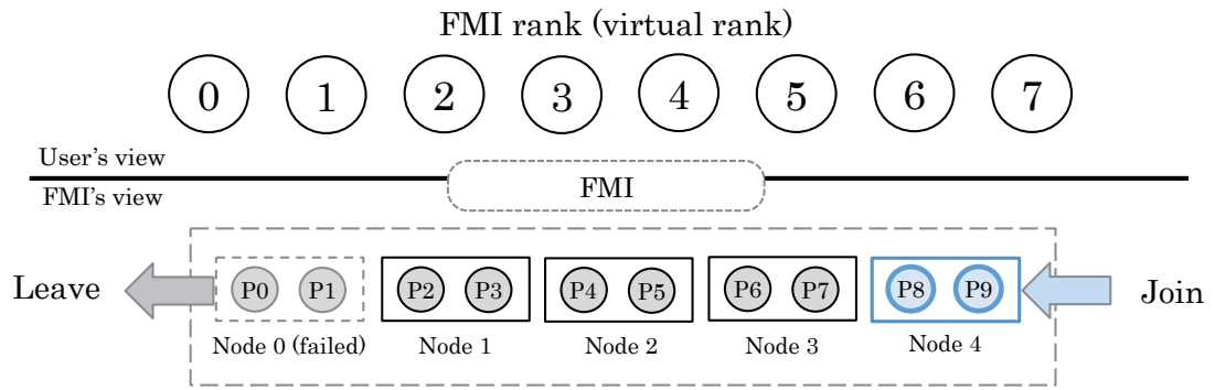
FIGURE 5.3: Overview of FMI
