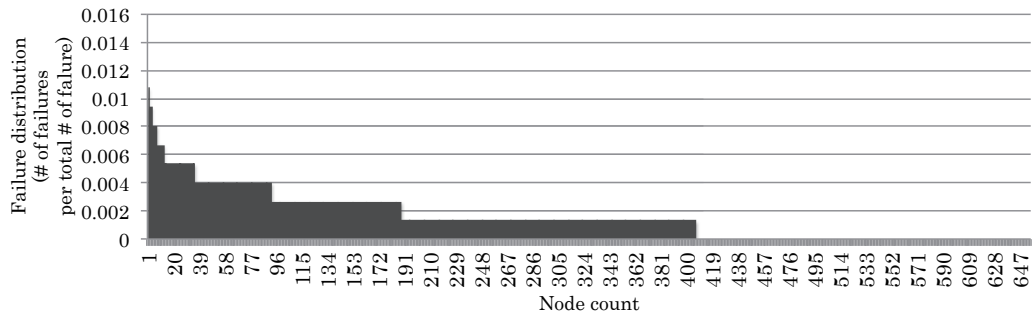
FIGURE 5.1: Tsubame1: Number of failures normalized by total failures (Period: 3.5 years of Oct 26 th 2006 - March 21 th 2010, Total # of failures: 744)
