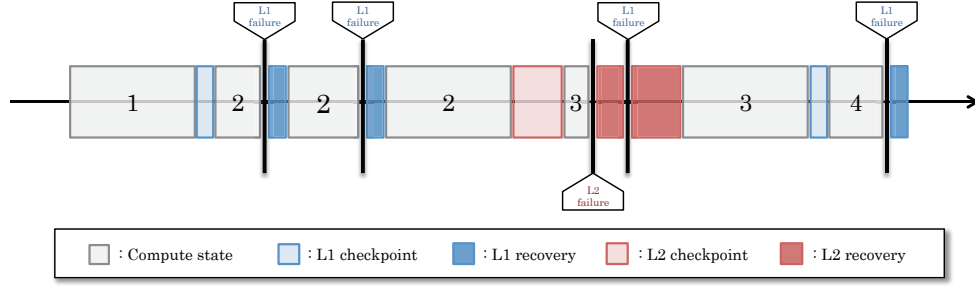
FIGURE 3.15: The multi-level checkpoint/restart simulator transition to compute/checkpoint/recovery states according to failure intervals generated by random numbers for an exponential distribution
