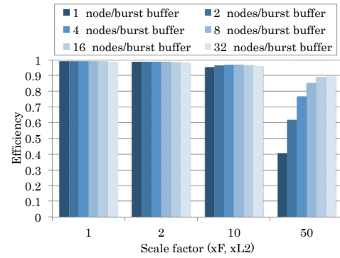
FIGURE 4.11: Uncoordinated: Efficiency in different ratios of compute nodes to a single burst buffer nodes with uncoordinated checkpoint/restart
