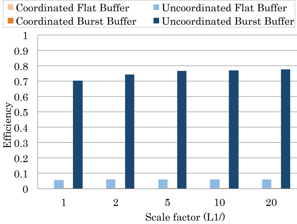
FIGURE 4.8: Efficiency in increasing level-1 checkpoint/restart performance in \times 100 failure rate: L1 checkpoint/restart time/scale factor
