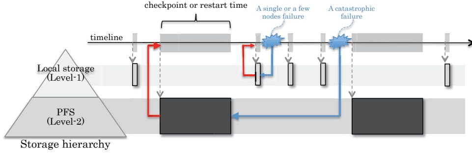
FIGURE 2.8: Multi-level checkpoint/restart
