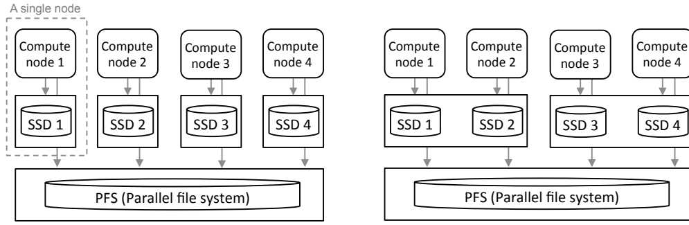
FIGURE 4.2: (a) Left: Flat buffer system (b) Right: Burst buffer system
