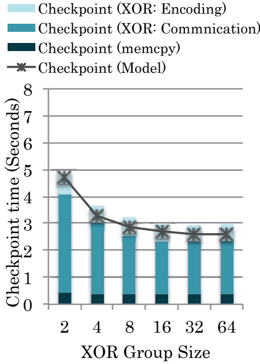
FIGURE 5.11: XOR checkpoint time
