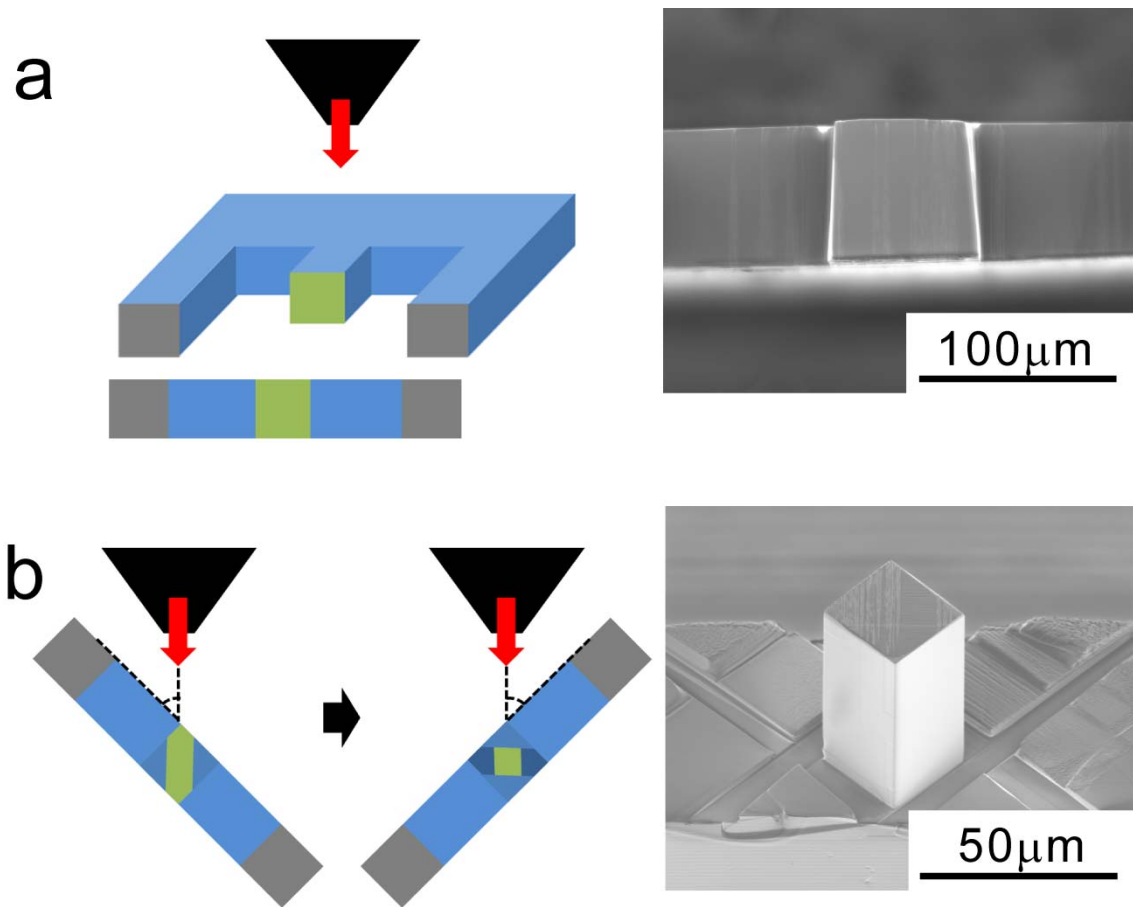
Figure 2-1. Procedures of making compression pillar and SIM images showing the pillar after the procedures: (a) perpendicular irradiation and (b) irradiation from 45 degrees from thin plate.
