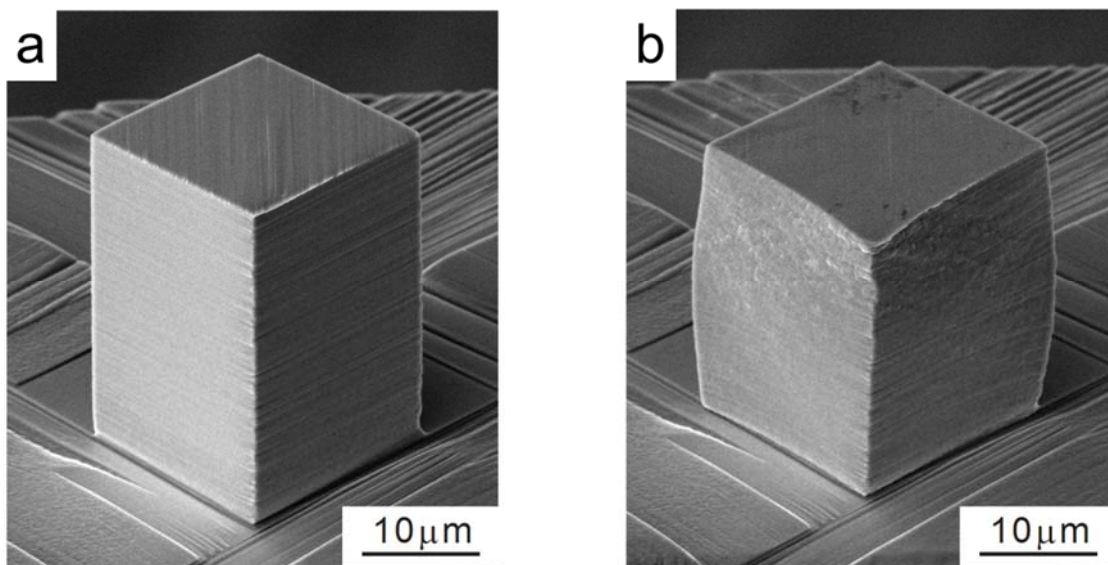
Figure 2-5. Representative SEM images of fabricated pillar (a) before and (b) after compressive deformation.
