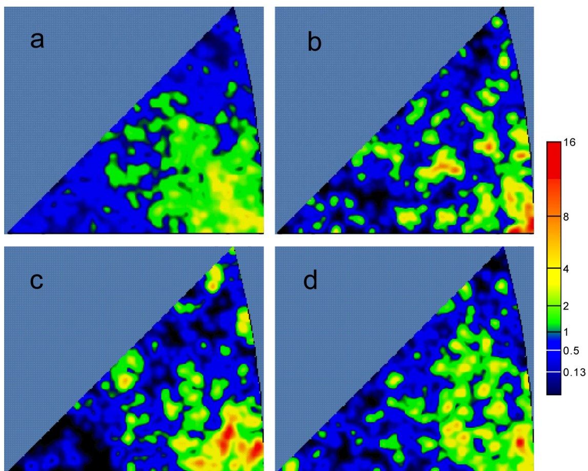
Figure 2-4. Inverse pole figure shows preferred orientation normal to the HPT disk
