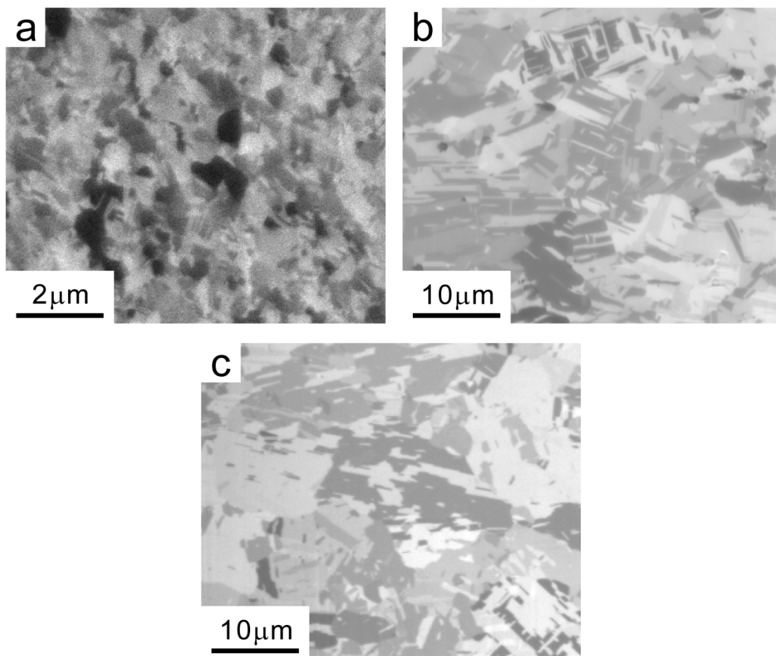
Figure 3-2. SIM images of copper film (a) as deposited ESCE , (b) two months after ESCE and (c) CONV plated.
